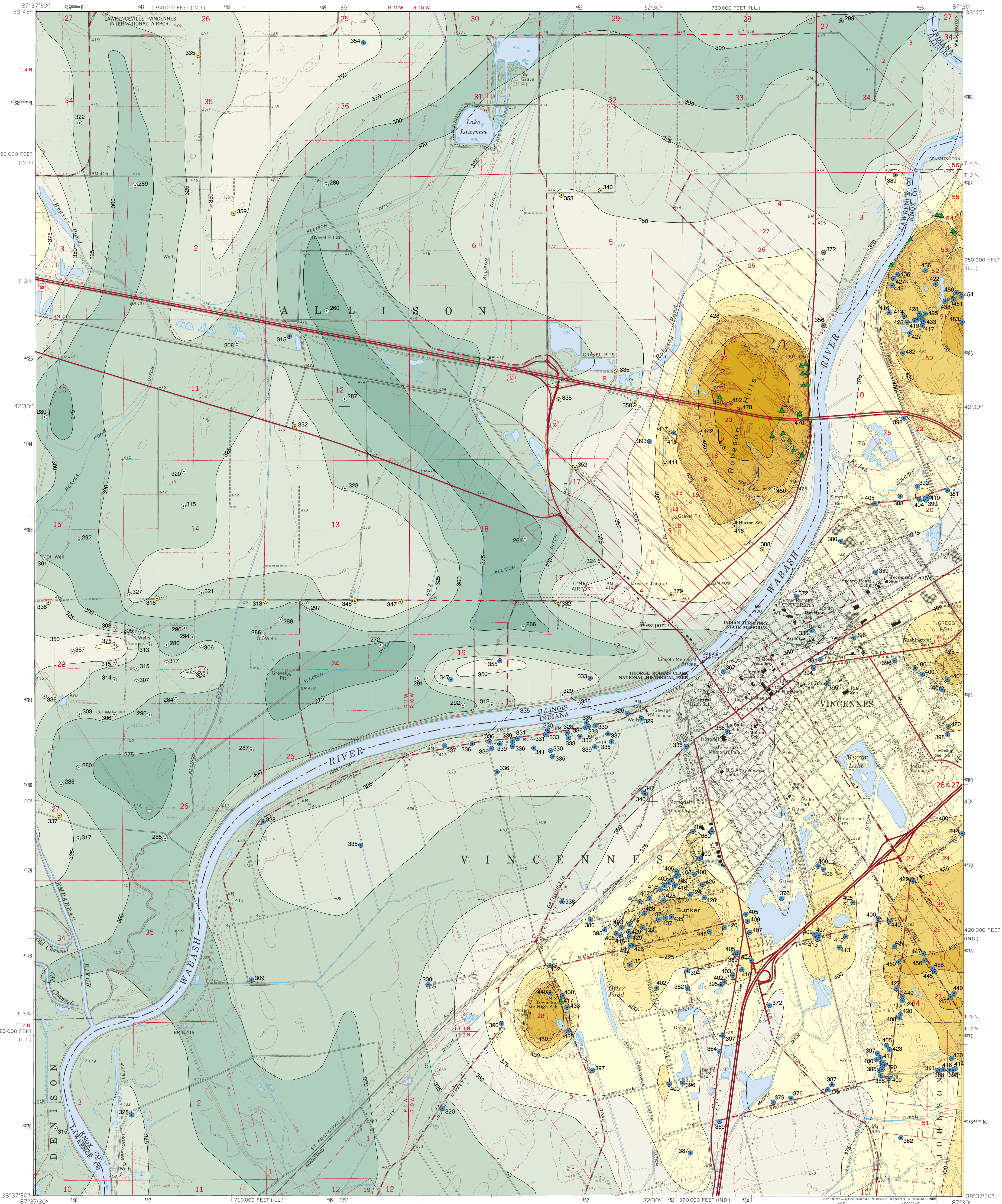
Figure 1 Map of the quadrangle showing a hypothetical landscape of uplands and lowlands prior to Wisconsin Episode glaciation. Present-day, isolated bedrock uplands (indicated by closed contour lines) were likely once contiguous with the adjacent uplands on the east side of the Wabash River Valley. Wisconsin Episode glacial outwash filled the valley to the level where floodwaters were able to flow across divides, eroding drainage channels on the upland spurs, and creating the isolated hills (Fidlar 1936).
