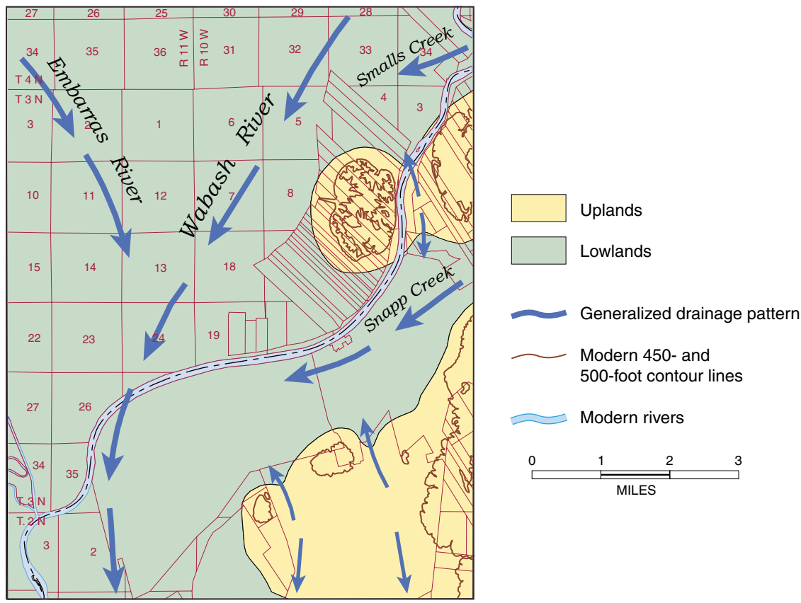
Figure 1 Map of the quadrangle showing a hypothetical landscape of uplands and lowlands prior to Wisconsin Episode glaciation. Present-day, isolated bedrock uplands (indicated by closed contour lines) were likely once contiguous with the adjacent uplands on the east side of the Wabash River Valley. Wisconsin Episode glacial outwash filled the valley to the level where floodwaters were able to flow across divides, eroding drainage channels on the upland spurs, and creating the isolated hills (Fidlar 1936).
