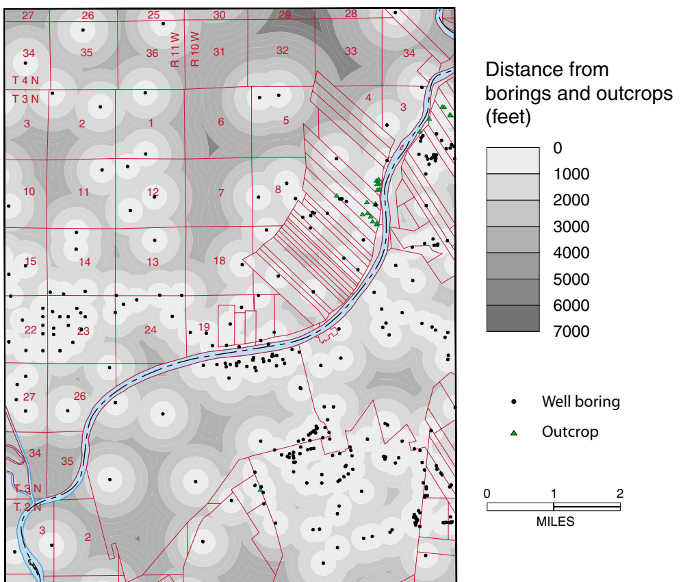
Figure 2 Data distribution map showing subsurface and outcrop data used to construct the bedrock topography map. Data points are buffered by 1000-foot wide contours.
