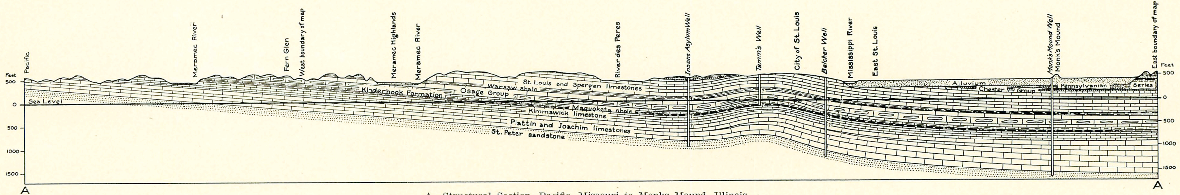
A—Structural Section, Pacific, Missouri to Monks Mound, Illinois.
