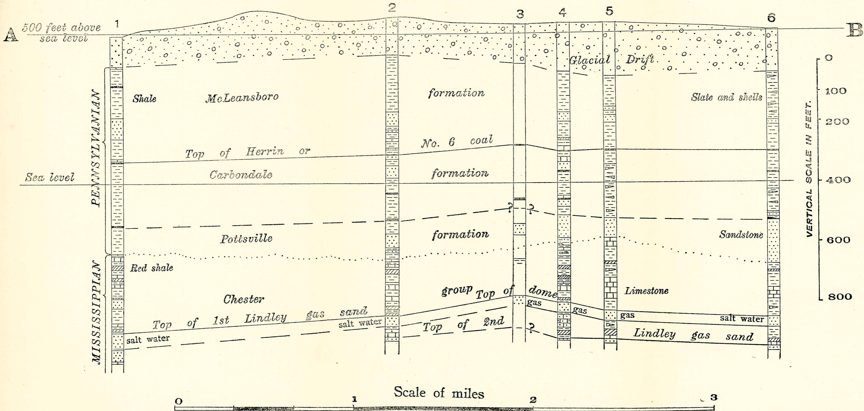
Cross-section through the Greenville Gas Field
