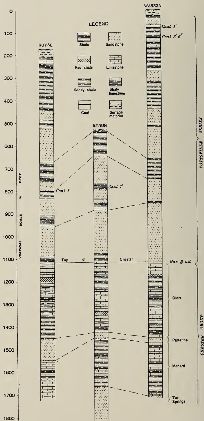
FIG. 8.—Graphic sections of the Royse, Bynum, and Warren wells.
