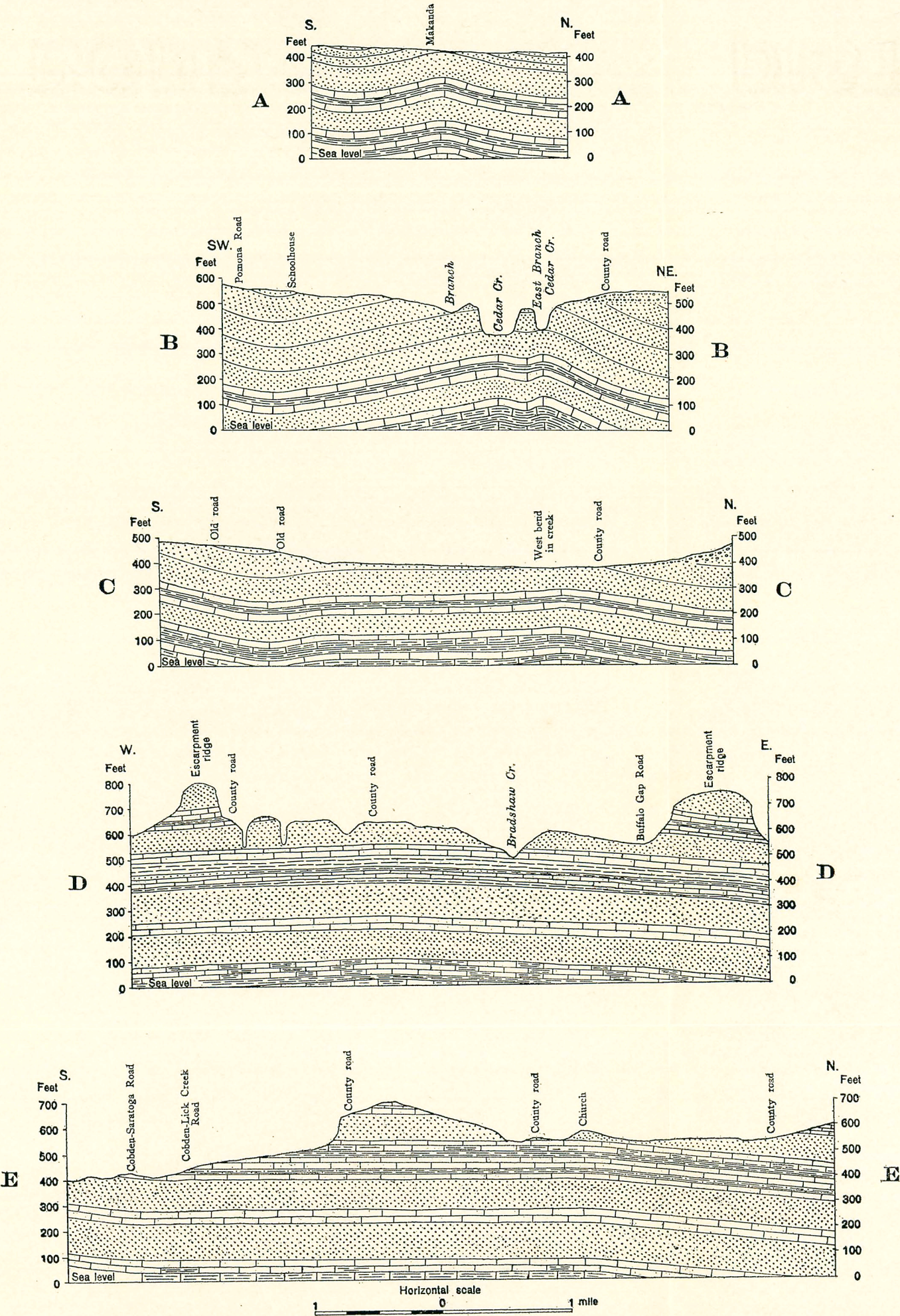
Geologic cross-sections in Williamson, Jackson, and Union counties
