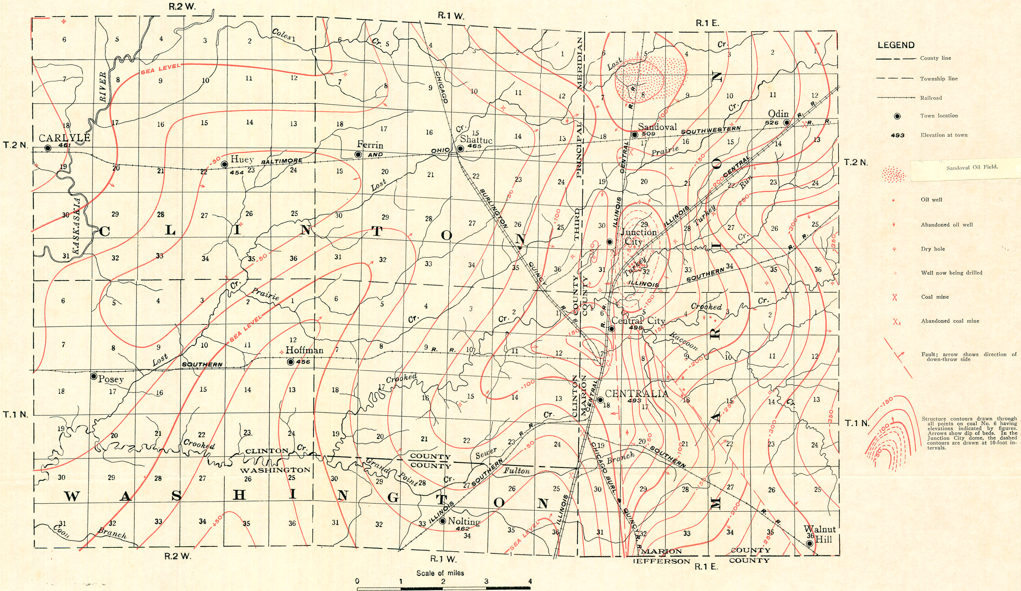
Map showing geologic structure in the Centralia area
