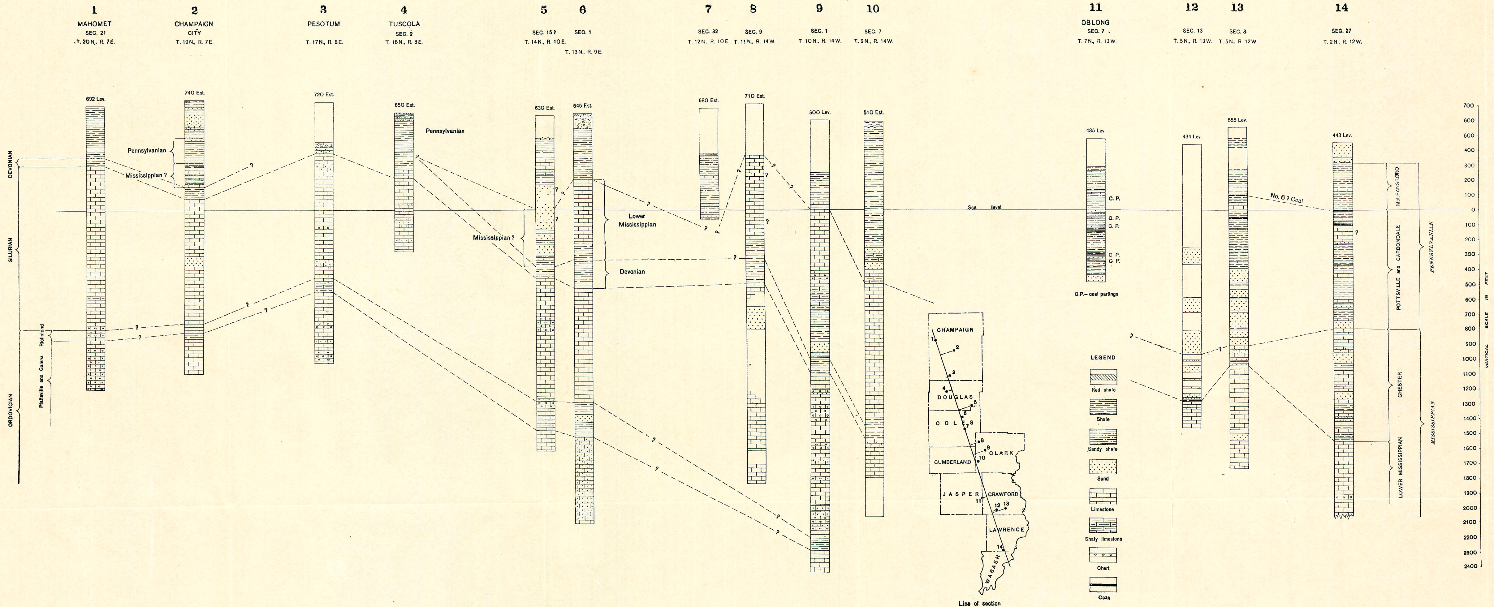
PLATE IV.—Structure section from Mahomet south to southern Lawrence county.
