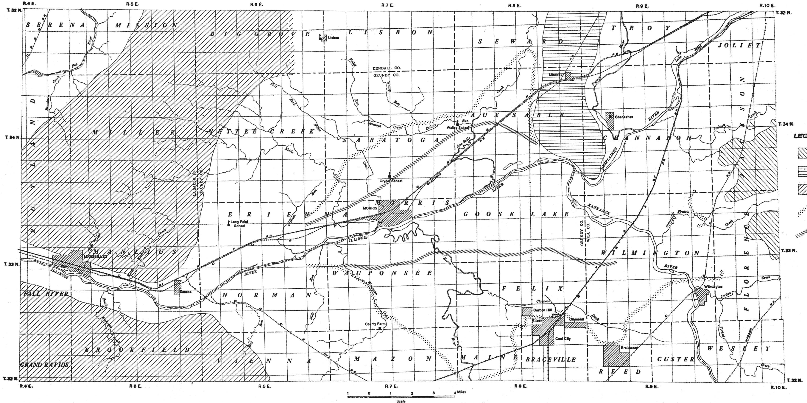
Map of Morris Basin showing major physiographic features
