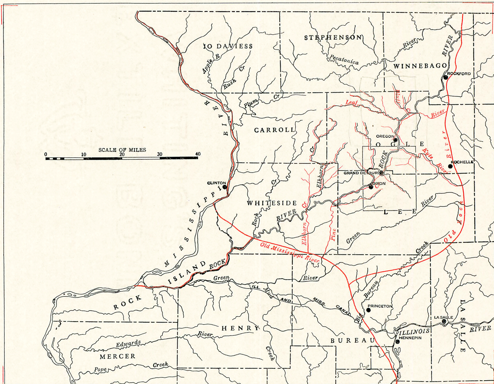
Map showing changes in Rock River and its tributaries resulting from Illinois glaciation.
