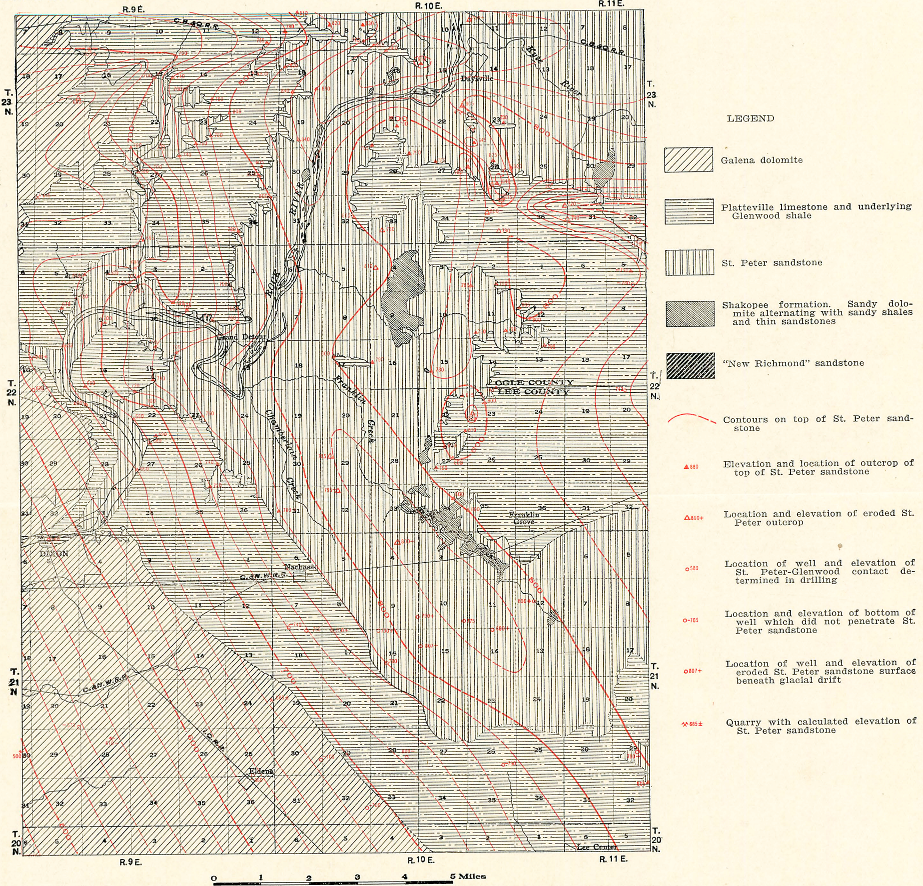
Areal geology map of the Dixon quadrangle with structure contours drawn on the top of the St. Peter sandstone.
