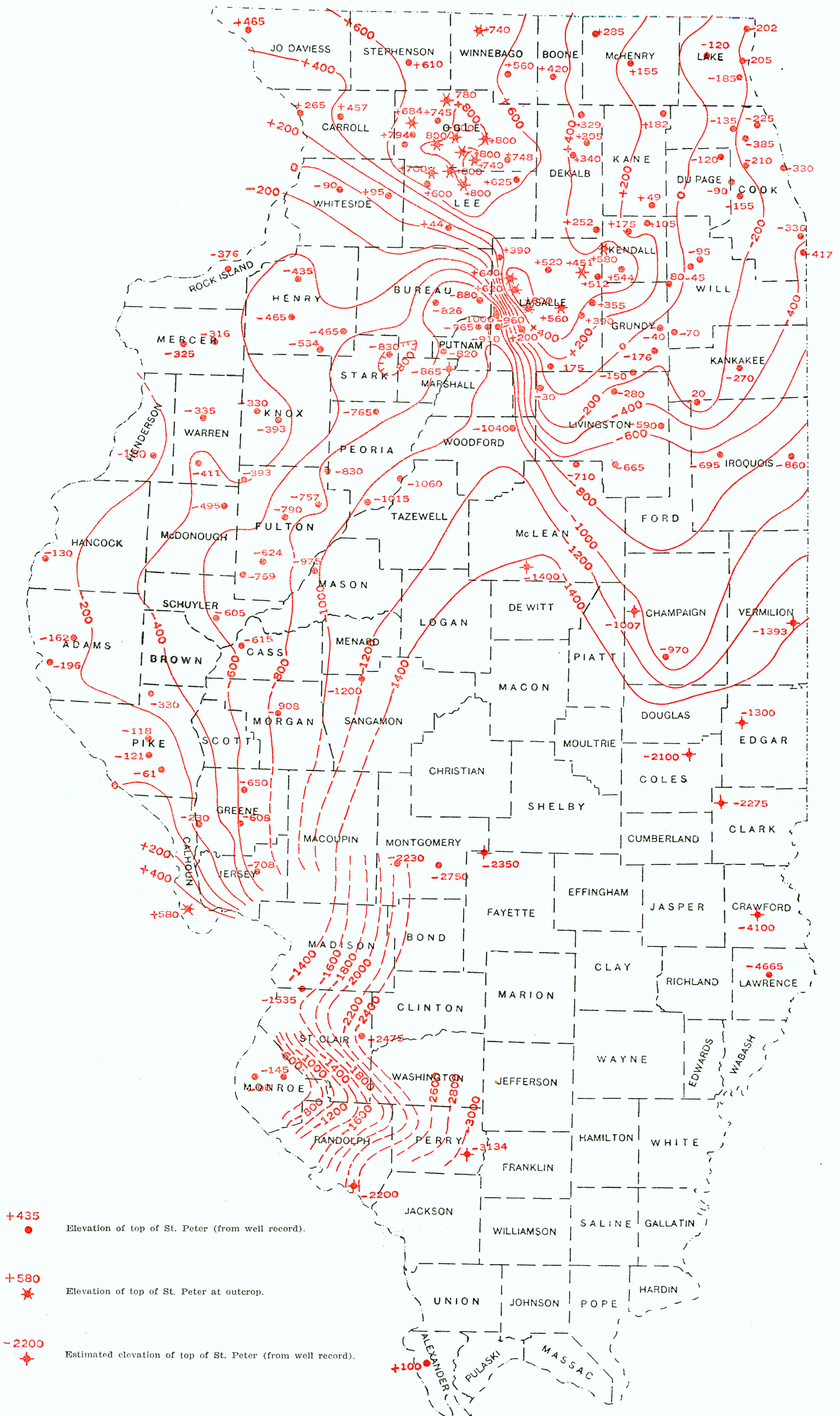
Structure contour map drawn on the top of the St. Peter sandstone in Illinois.
