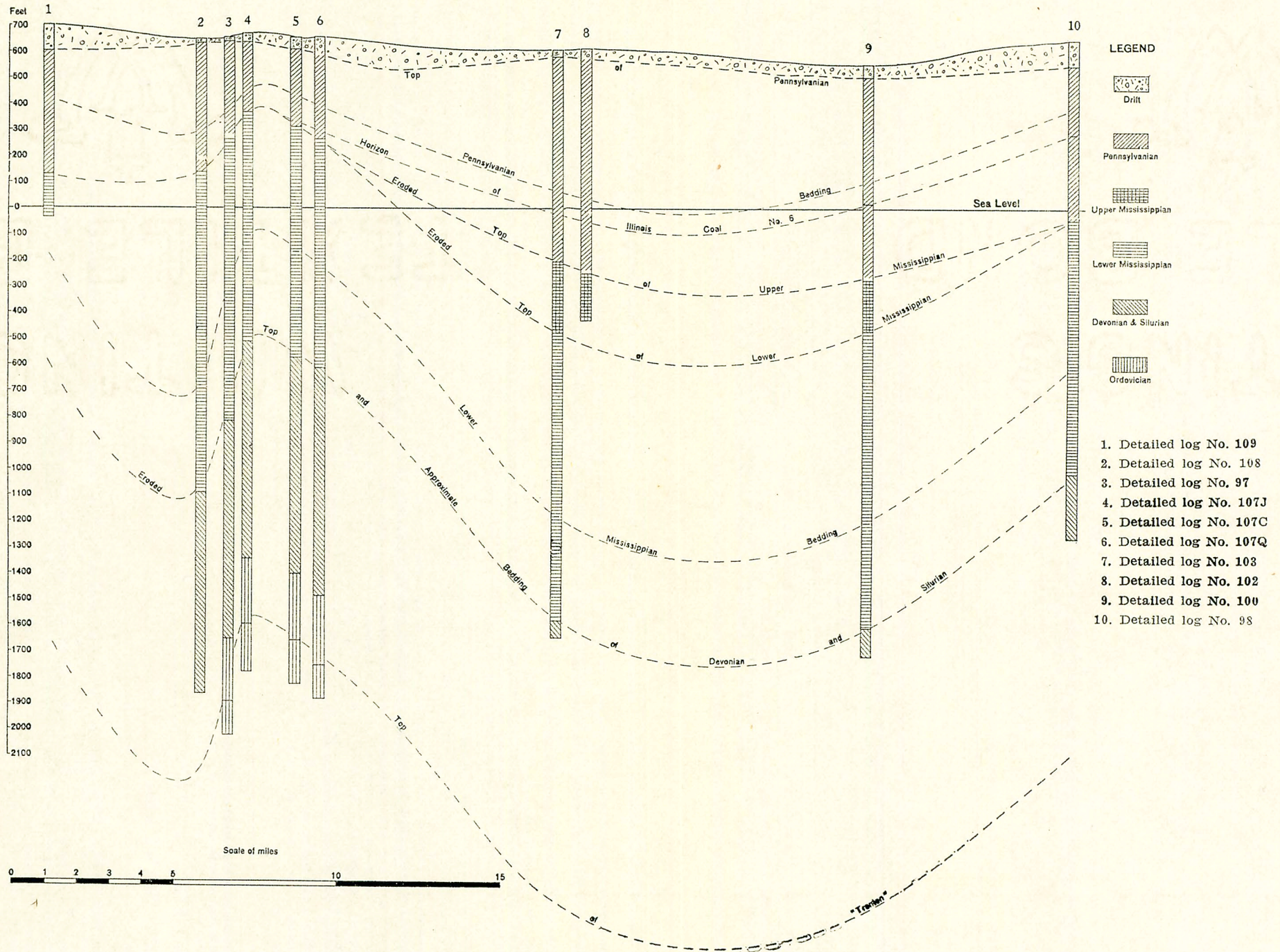
Structural section L-M through the Westfield pool. There is a possibility of a local reversal near logs Nos. 5 and 6 which would modify the bedding lines shown. Farther east, cross folding may cause local effects not indicated. A possible though improbable error may occur in the correlation of log No. 1 in respect to the bedding older than Pennsylvanian. (A set of all the detailed logs to which reference is made in this report is available for examination upon request to the Chief, State Geological Survey, Urbana, Illinois.)
