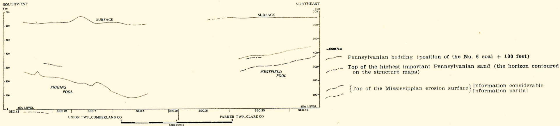
Southwest-northeast section from the Siggins to the Westfield pool, showing the approximate behavior of the Pennsylvania bedding; and the position of the eroded Mississippian top and of the most important Pennsylvania pay with respect to each other and to No. 6 coal in the two pools.
