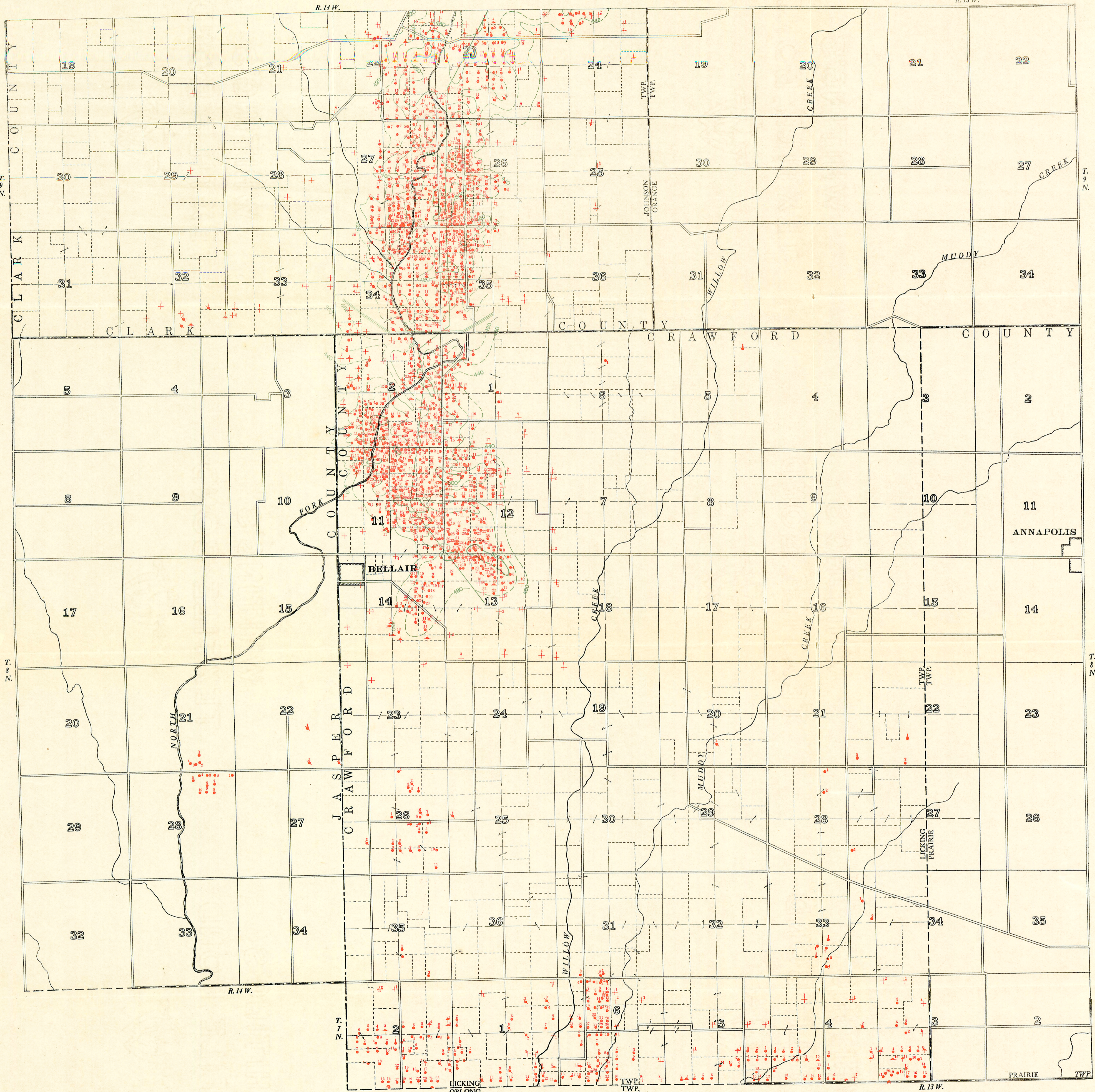
Detailed map of the southern part of the Clark County oil field, showing the South Johnson and Bellair pools; their structure (in green); and the locations of all the wells and dry holes (in red), numbered for reference to the Tables of Well Data.
