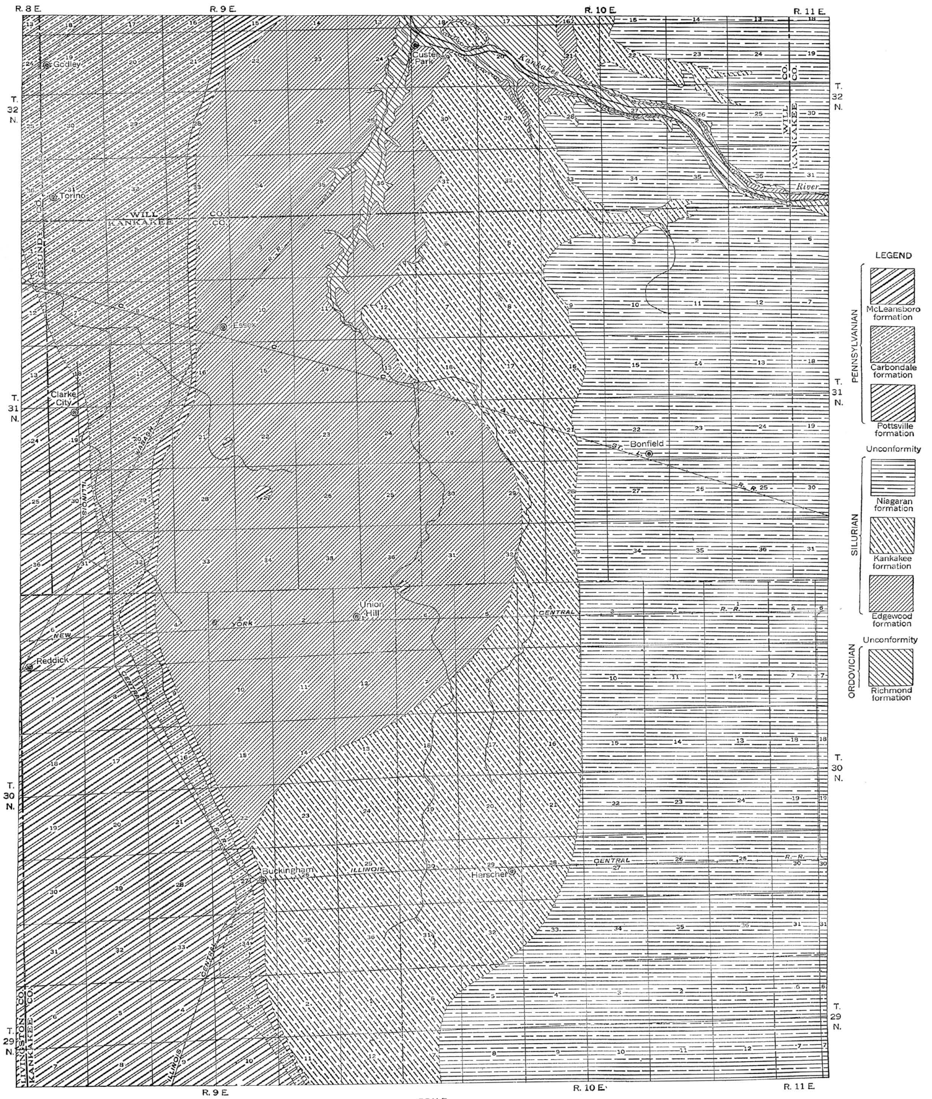
Areal geology of the Herscher quadrangle.
