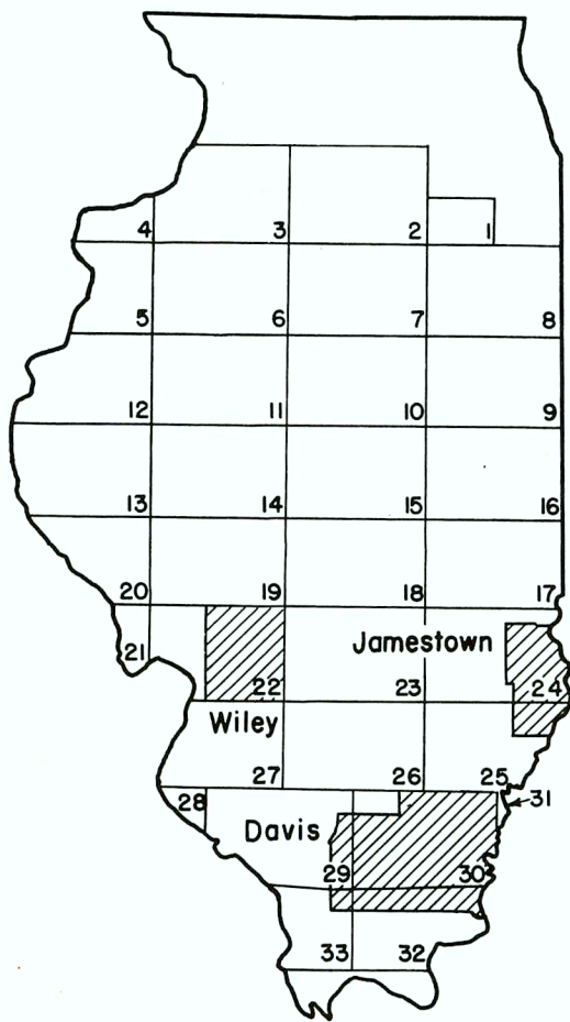
Index Map Showing COAL RESOURCES AREAS and locations of WILEY, JAMESTOWN, AND DAVIS COALS
