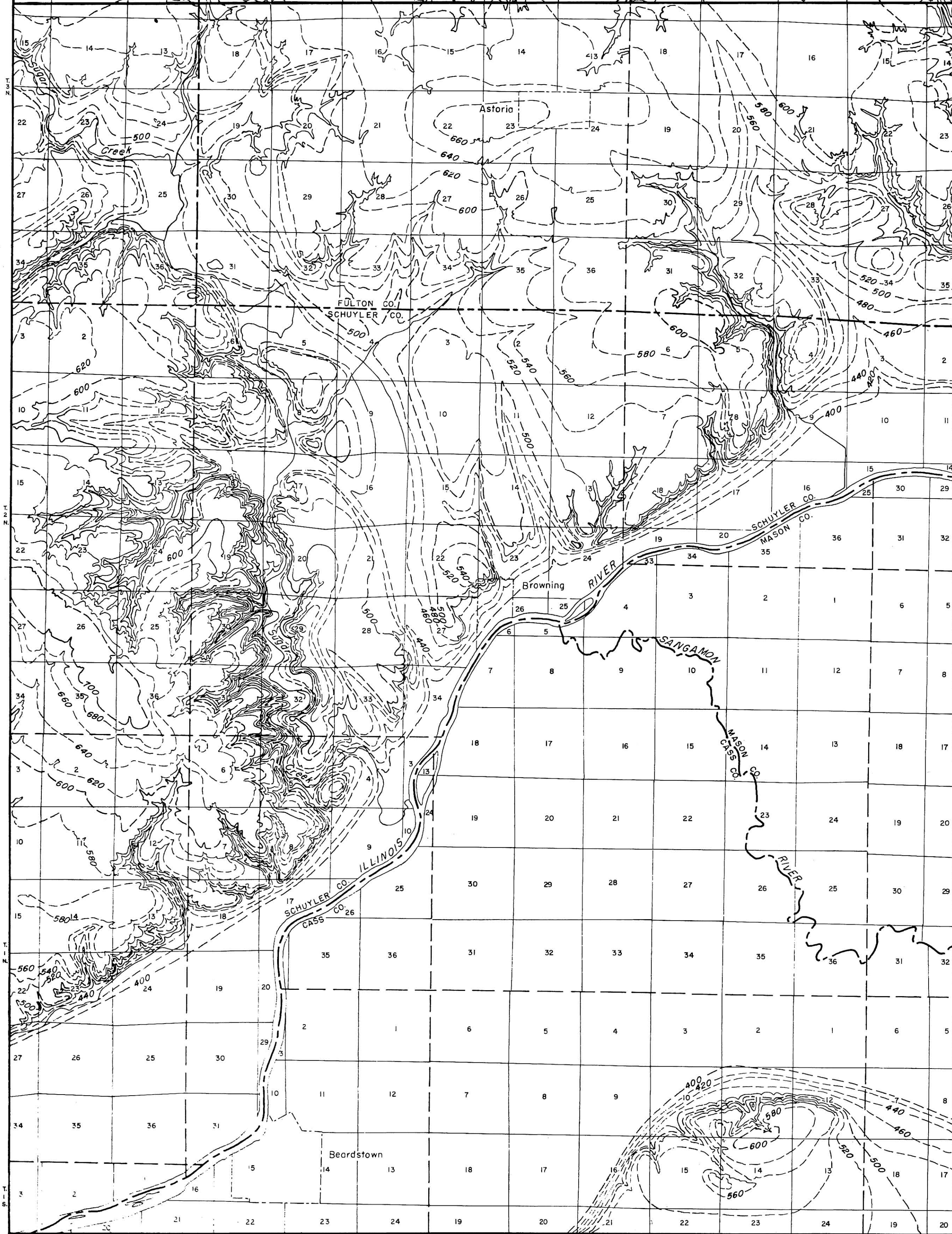
BEDROCK TOPOGRAPHY OF THE BEARDSTOWN, GLASFORD, HAVANA AND VERMONT QUADRANGLES By H. R. Wanless
