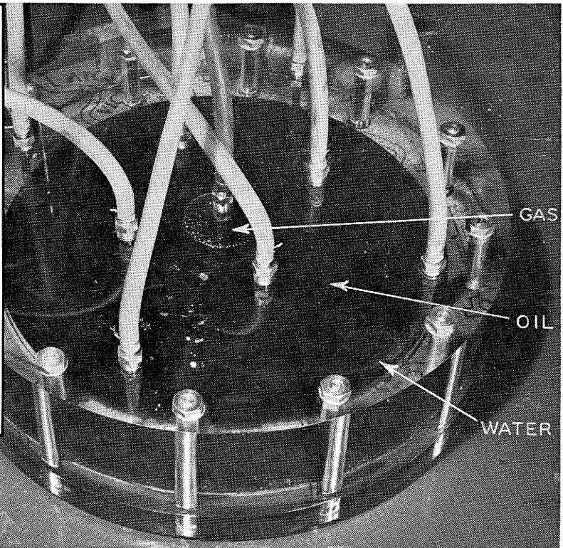
Figure 5. This shows the sand almost full of oil but with gas cap at the top of the structure and water at the extreme lower and outer edge.
