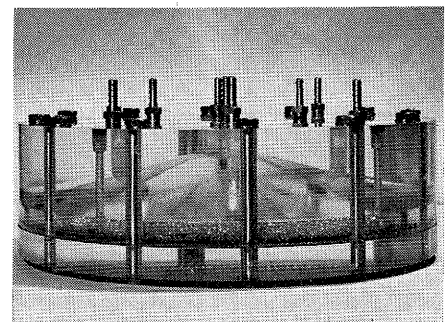
Figure 3. View from the side, showing the transparent model. The structure is evident as well as the glass beads representing the sand.
