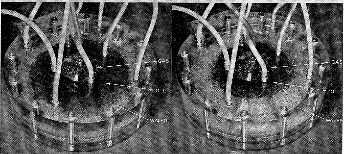
Figure 6. These are two views of the squeeze—the gas cap and water edge having been enlarged and part of the oil vented.
