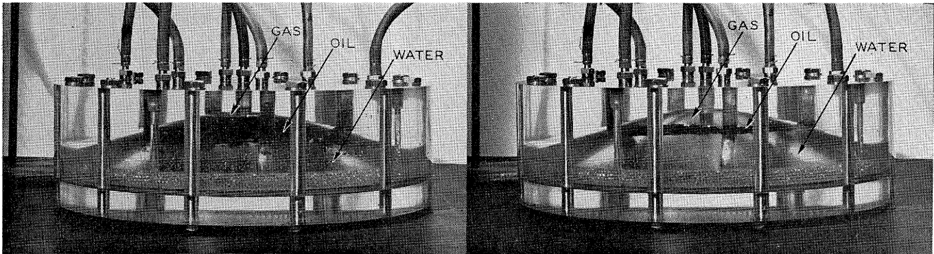
Figure 5. This shows the sand almost full of oil but with gas cap at the top of the structure and water at the extreme lower and outer edge.
