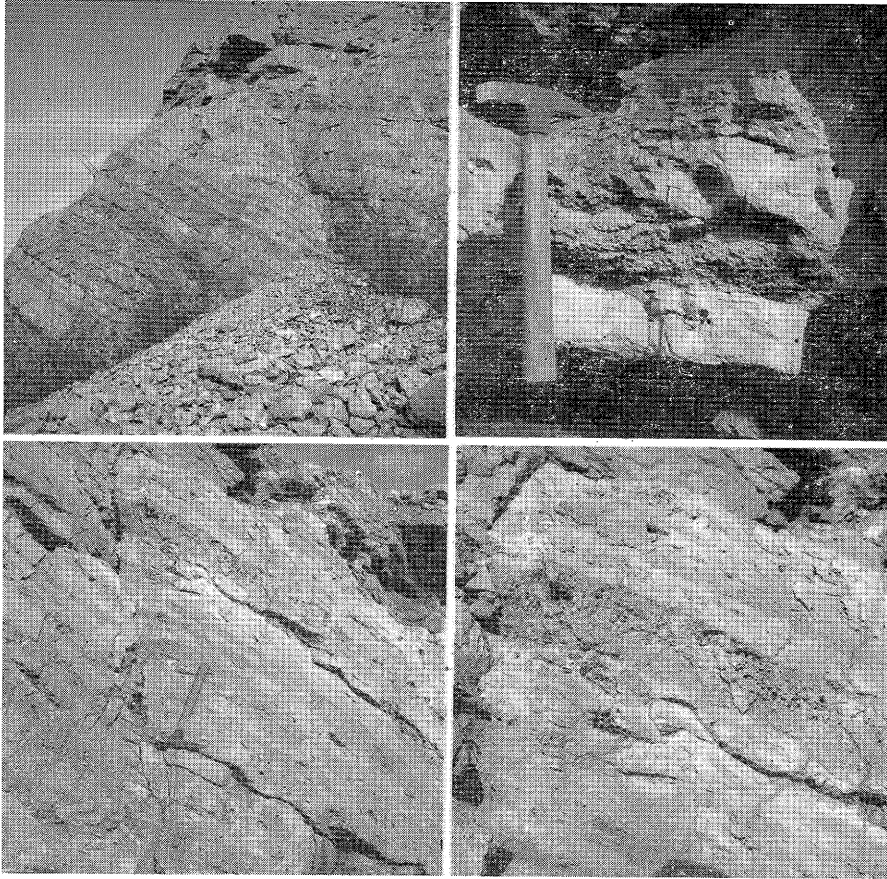
FIG. 1.—Cyclical reef-flank deposits consisting of alternating layers of coarse bioclastic debris (dark) and dense, structureless dolomite (light) in the south flank of Thornton reef in north portion of old (south) quarry of the Material Service Company, Thornton, Ill. Upper left .—Cyclical deposition in flank portion brought out through weathering; dark layers consist of bioclastic debris. Upper right .—Closeup of two coarse bioclastic debris layers with alternating dense dolomite, northeast of section shown in first picture. Lower left .—Cycles farther from the reef core south of those shown above. Lower right .—Closeup of portion above hammer shown at left.
