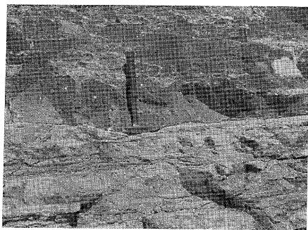
FIG. 6.—Close-up of Chouteau-Sedalia contact at Chautauqua.
