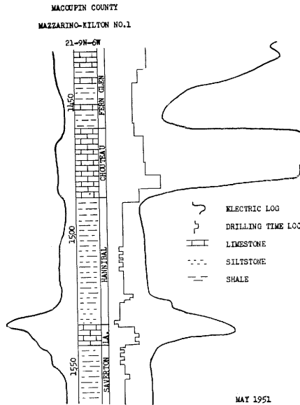
FIG. 5.—Relationship of Chouteau and Louisiana limestones.
