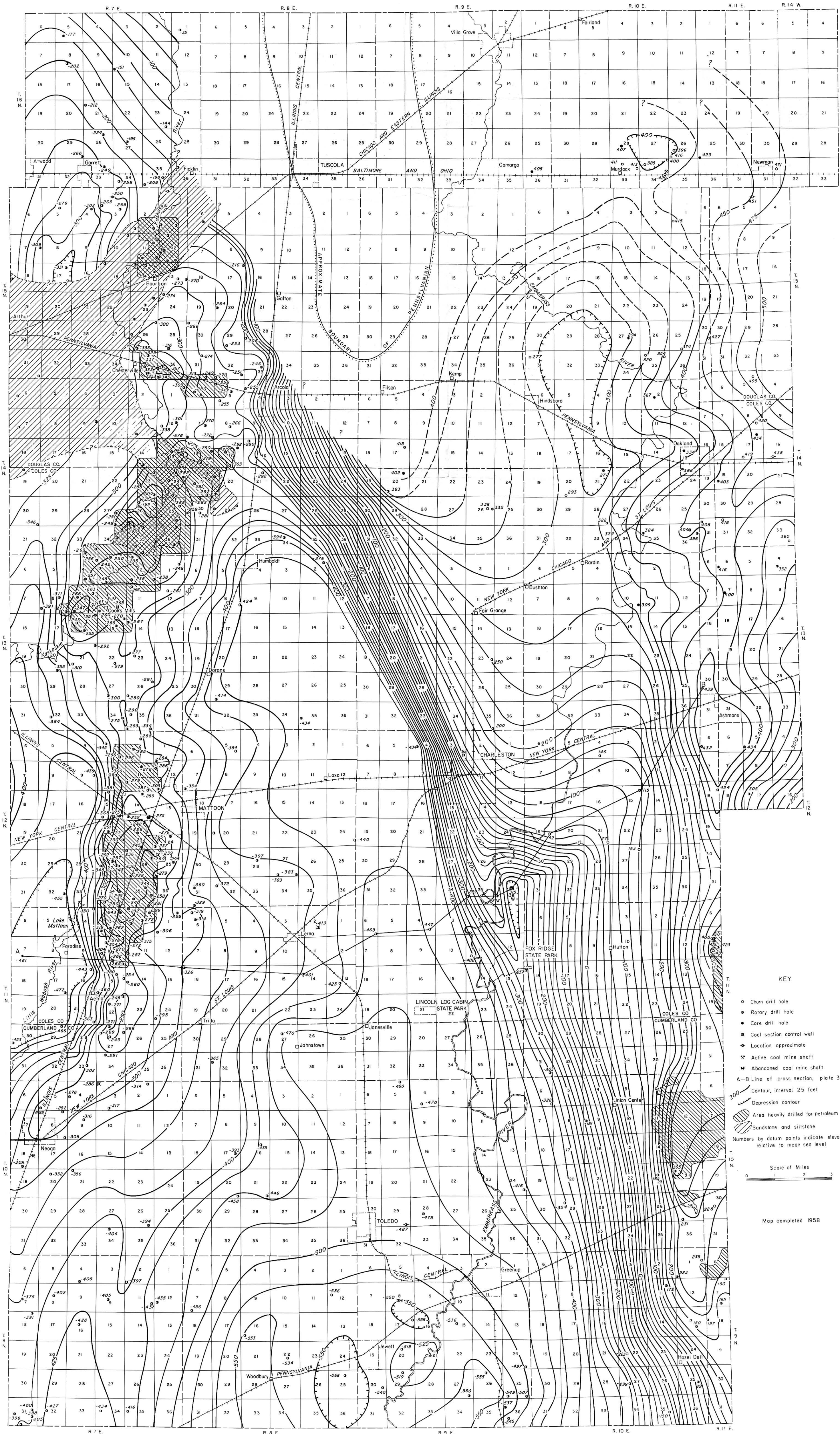
B - STRUCTURE CONTOUR MAP ON TOP OF NO. 6 COAL IN CUMBERLAND, COLES, AND DOUGLAS COUNTIES
