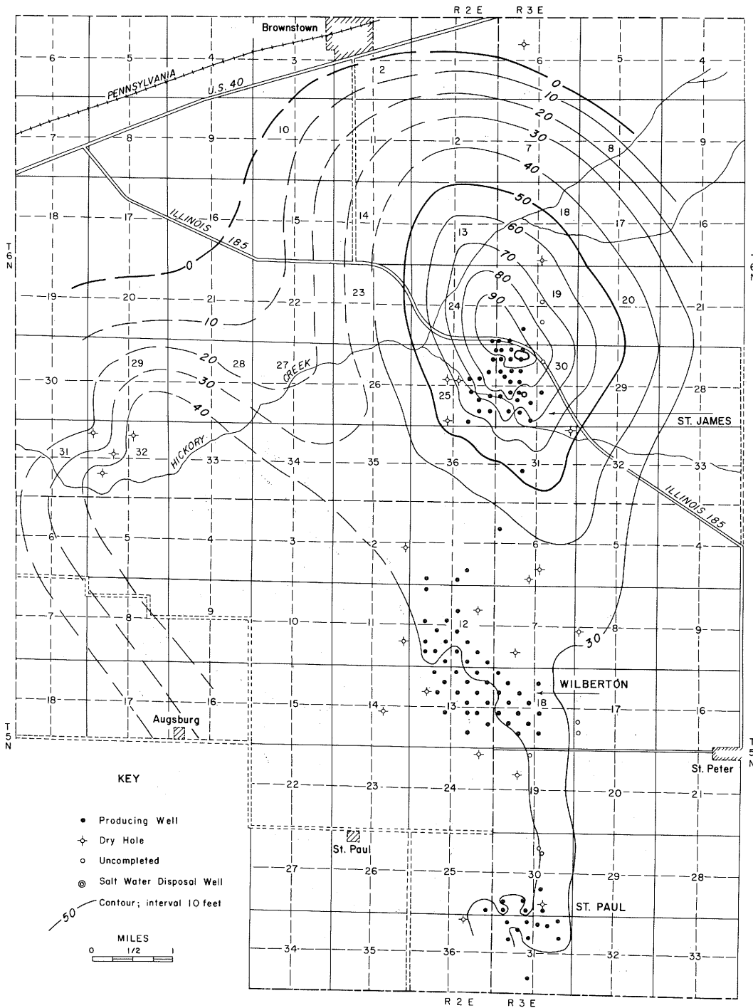
Fig. 4 - Isopach of the Carper sand.
