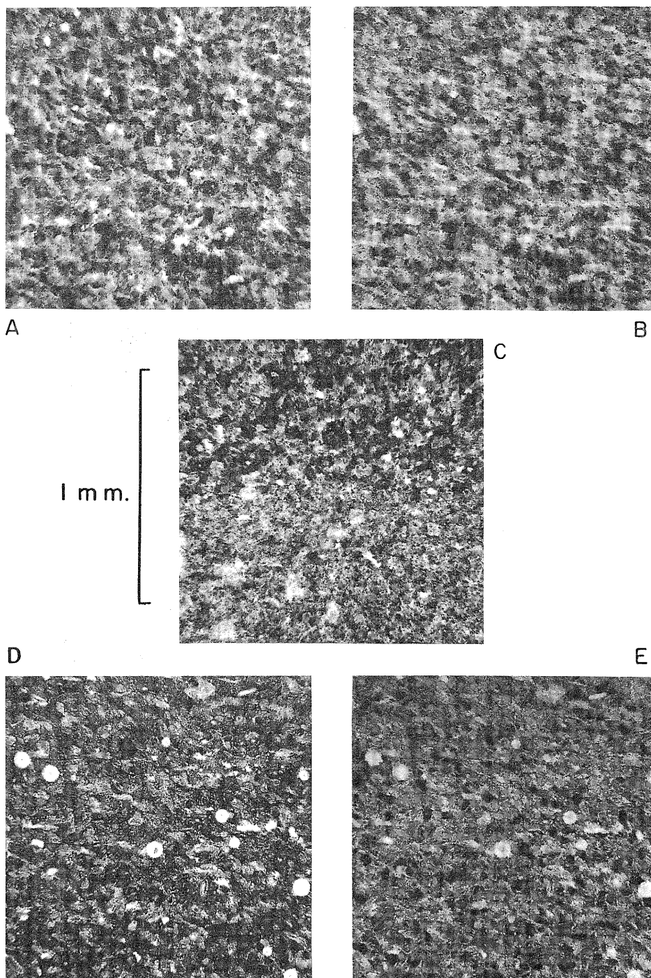
Fig. 7 - Photomicrographs of Carper sand thin sections.
