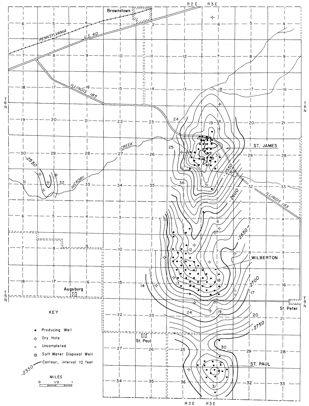
Fig. 6 - Structure map of the top of the Carper sand.
