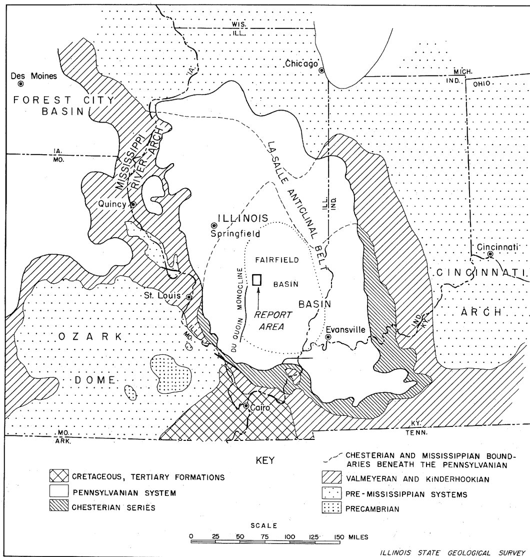
Fig. 1 - Index map showing geologic setting of report area.
