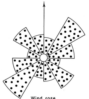
Wind rose showing strike orientation of 383 measured joints
