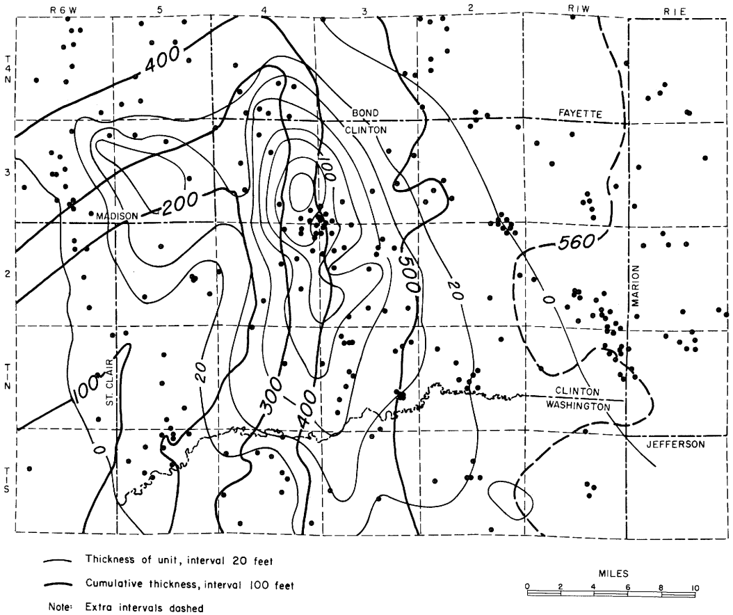
Figure 12 - Thickness of unit H-I and cumulative thickness from base of the Borden to horizon I.
