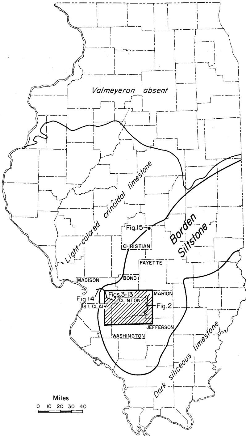
Figure 1 - Areal extent of the Borden Siltstone in Illinois.
