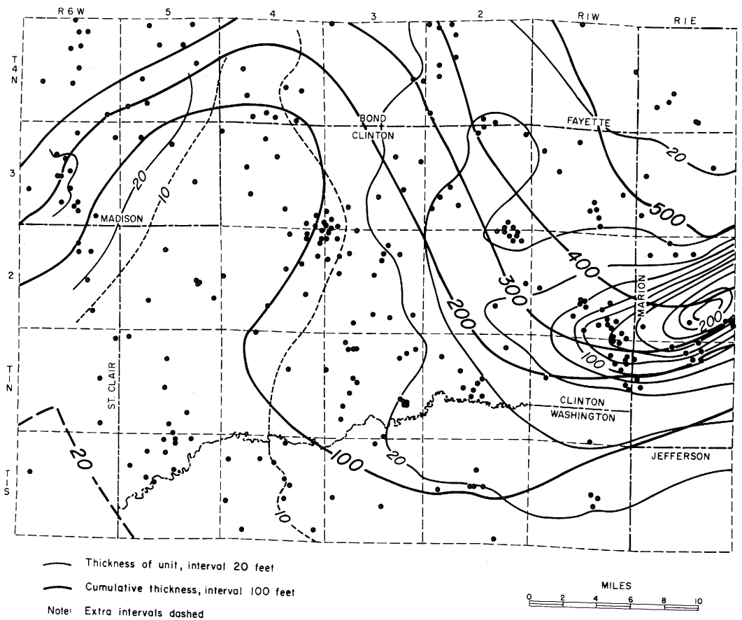
Figure 8 - Thickness of unit D-E and cumulative thickness from base of the Borden to horizon E.
