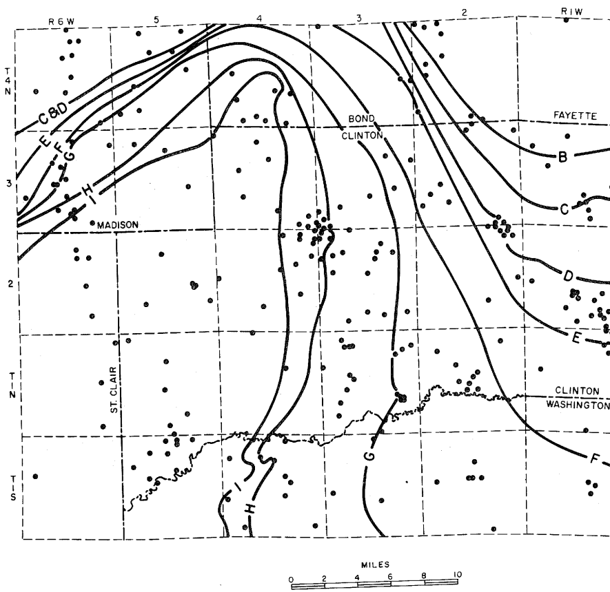
Figure 3 - Advance of the delta as shown by successive positions of the where the Borden reached a cumulative thickness of 300 feet, from figures 5-12.
