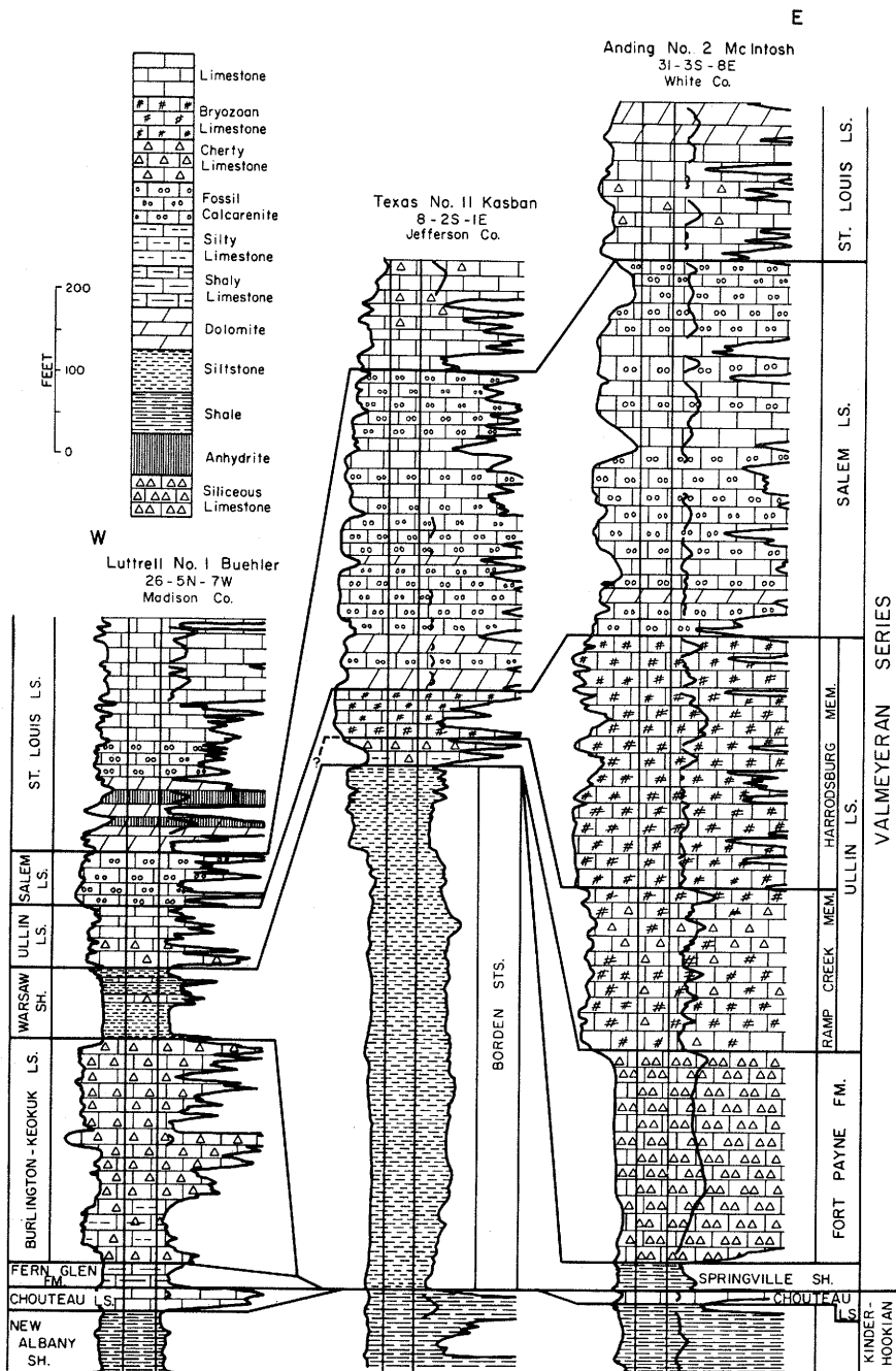
Figure 2 - Electric and lithologic logs showing the four major lower Valmeyeran units and stratigraphic nomenclature.
