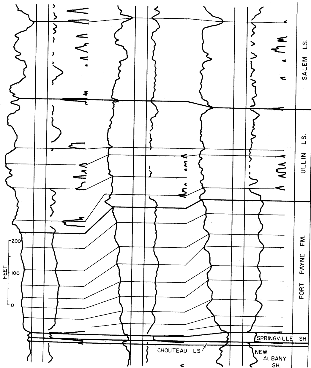
Figure 5 - Cross section showing west dip of inclined bedding in the Fort Payne Formation and Ullin Limestone on the west side of the Fort Payne tongue in Wayne County, Illinois (fig. 3).
