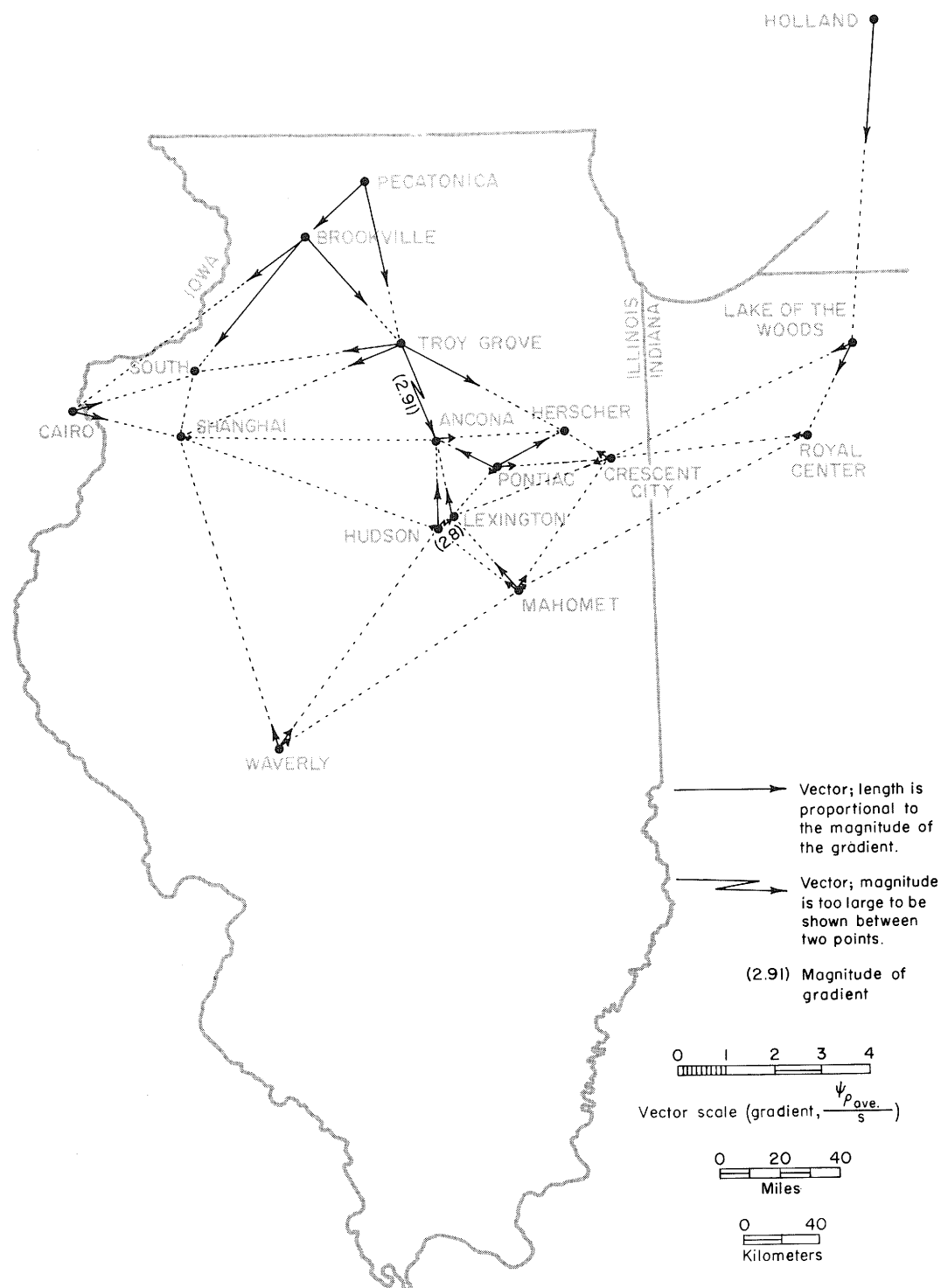
Fig. 19 - (\psi \rho_{ave.})/s for pairs of points in the Ironton-Galesville. Arrows indicate general direction of flow. Length of arrows is proportional to net force available to cause flow. (Data for Holland are for the Franconia.)
