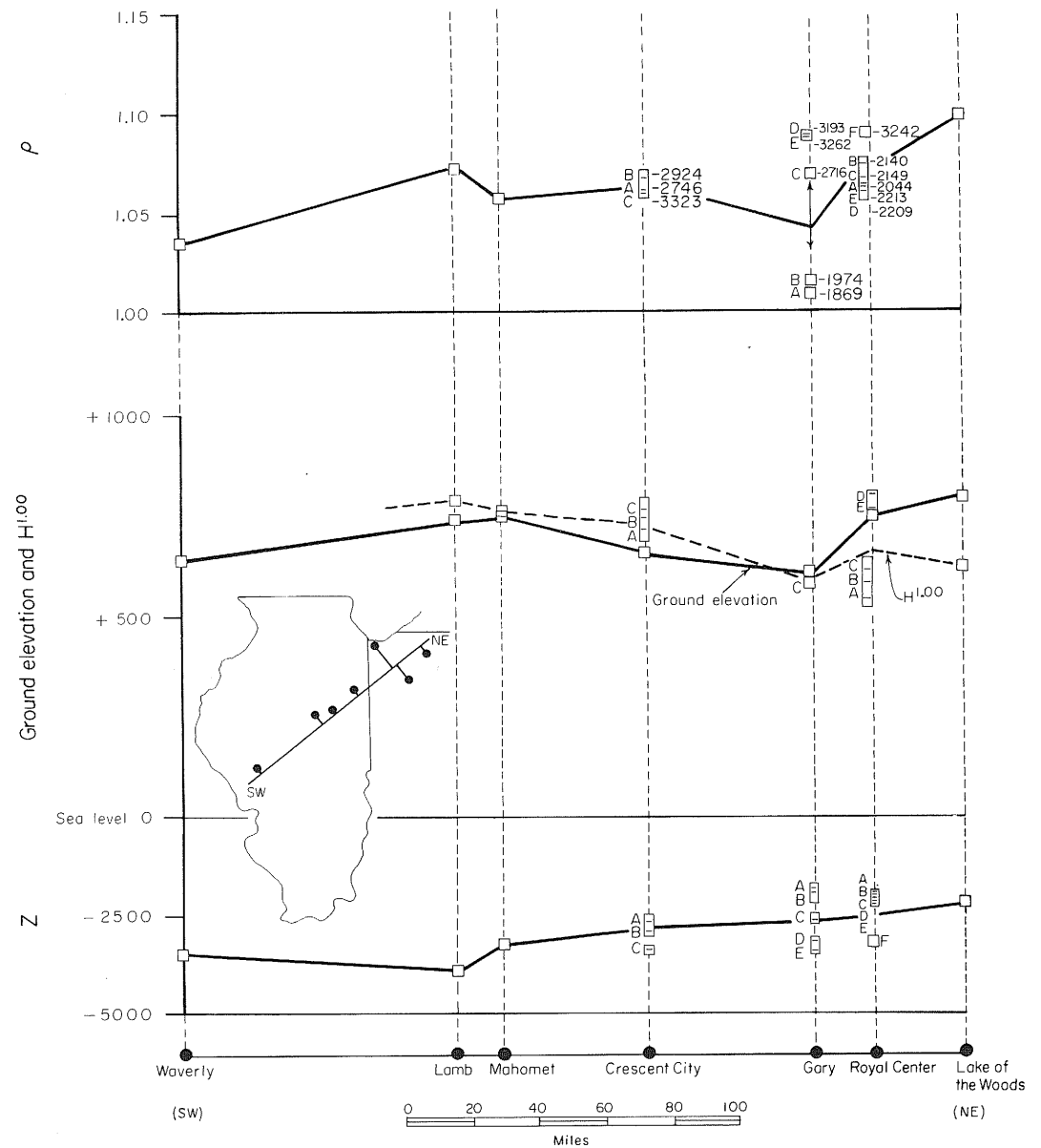
Fig. 6 - \rho , H^{1.00} , Z, and ground elevation for observation points in the Mt. Simon along NE-SW cross section. For Crescent City, Gary, and Royal Center, data are given for multiple observation levels: A, B, C.... On the plot of values of \rho , the numbers opposite the boxes are values of Z for levels A, B, C....
