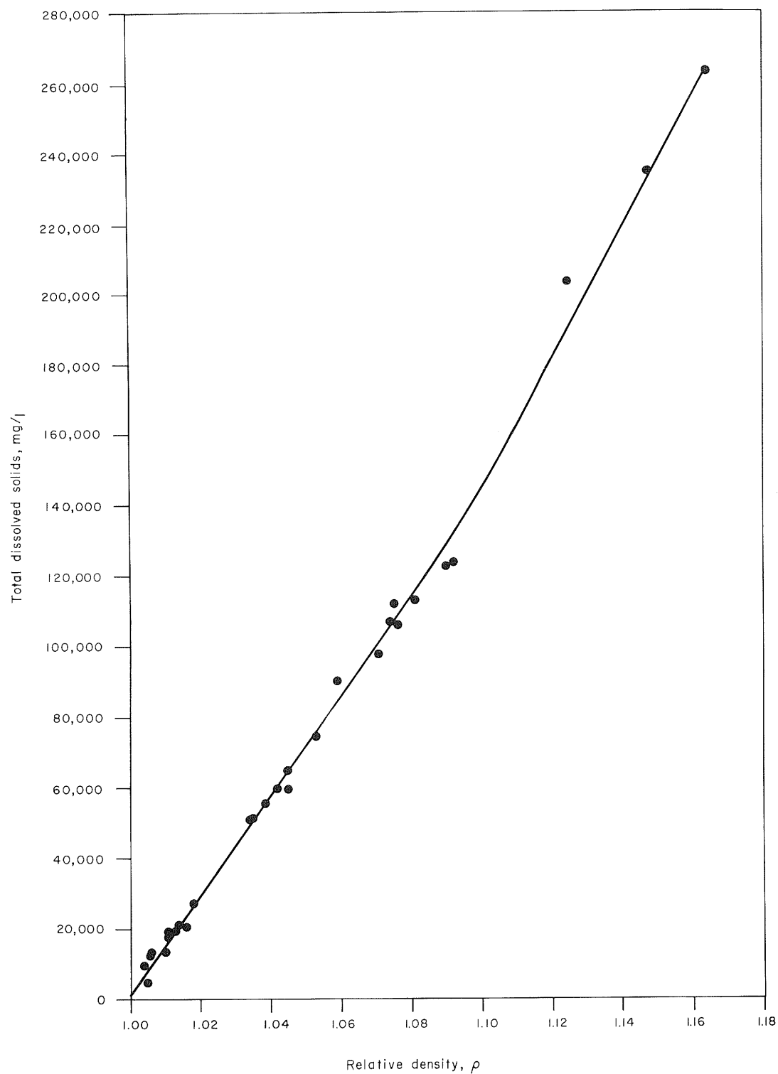
Fig. 9 - Relation between relative density and dissolved-solids content of brines in deep aquifers of the Illinois Basin.
