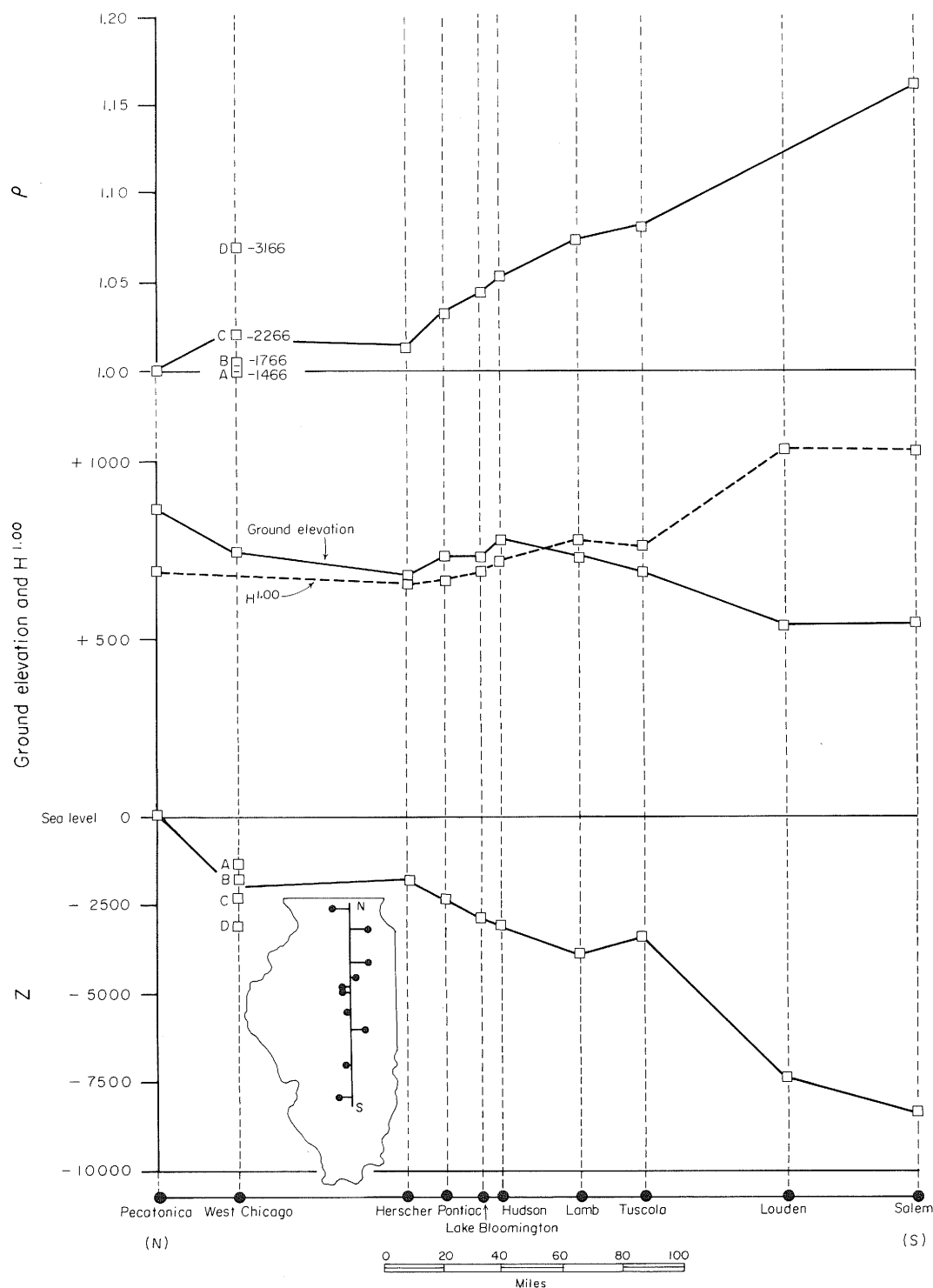
Fig. 5 - \rho , H^{1.00} , Z , and ground elevation for observation points in the Mt. Simon along N-S cross section. For West Chicago, data are given for four observation levels: A, B, C, and D. On the plot of values of \rho , the numbers opposite the boxes are values of Z for levels A, B, C, D.
