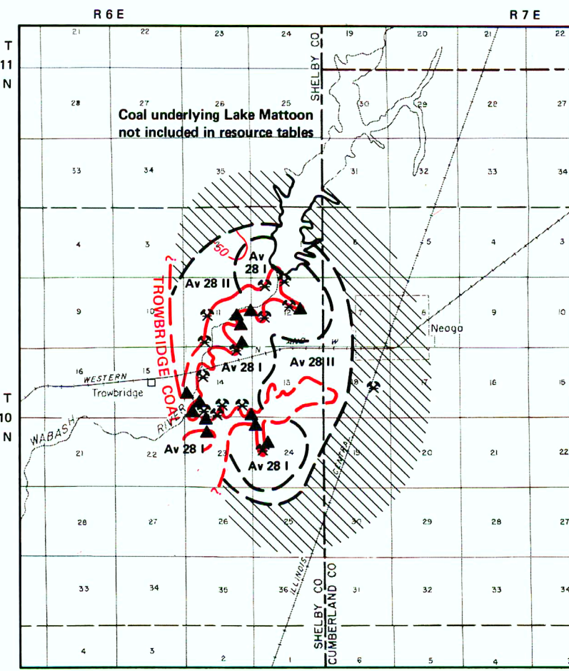
F. TROWBRIDGE COAL
