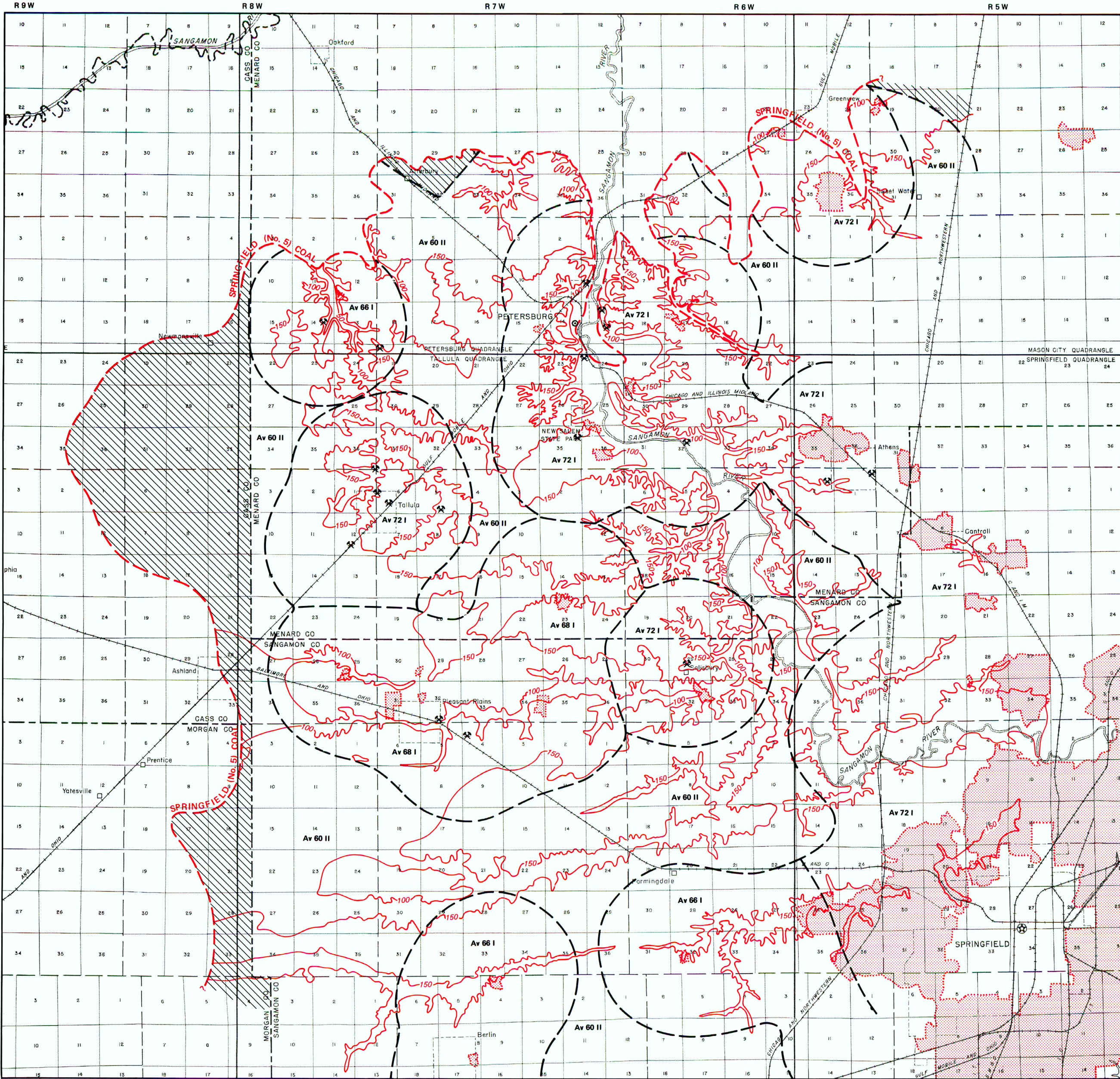
A. SPRINGFIELD (NO. 5) COAL
