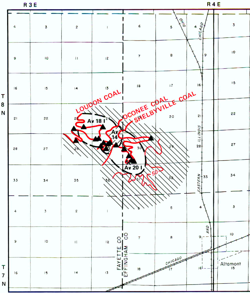
E. LOUDON COAL, OCONEE COAL, SHELBYVILLE COAL
