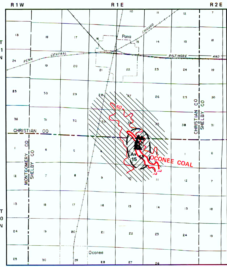
D. OCONEE COAL
