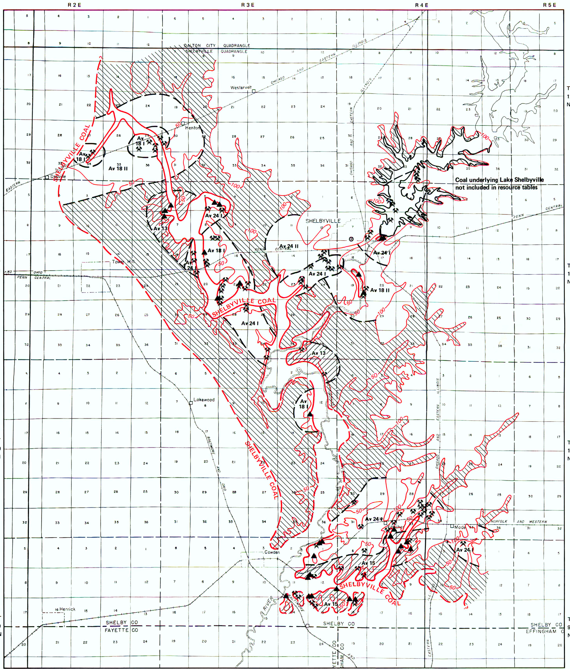
C. SHELBYVILLE COAL
