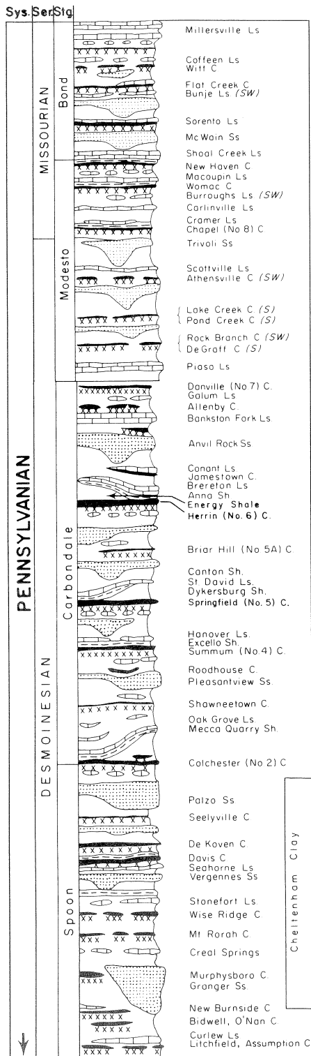
Figure 3. Generalized stratigraphic section of bedrock units along Cottage Grove Fault System. Units below Ste. Genevieve Limestone are rarely penetrated by drilling and are poorly known. Pennsylvanian section (after Willman et al., 1975); Mississippian section (after Swann, 1963).
