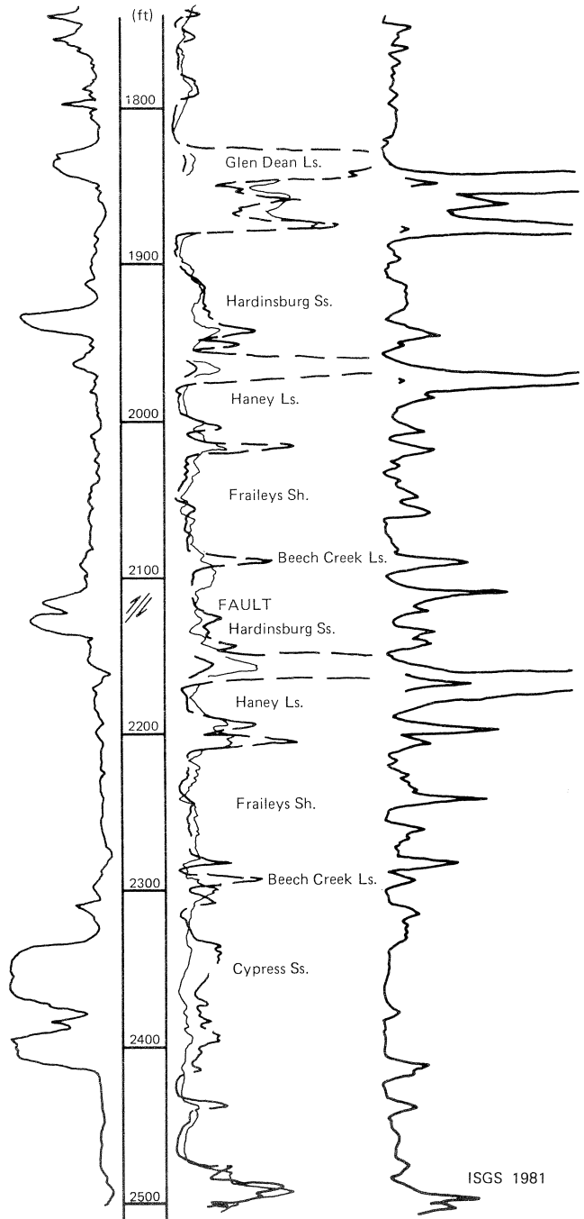
Figure 7. Electric log of oil test in SE \frac{1}{4} SE \frac{1}{4} NE \frac{1}{4} Sec. 4, T. 8 S., R. 2 E., Williamson County, showing approximately 200 feet (61 m) of repetition in the Chesterian strata. A reverse fault at a depth of 2,120 feet (646 m) is indicated. The structure is represented in the Pennsylvanian by an anticline, probably faulted, with over 200 feet (61 m) of closure.
