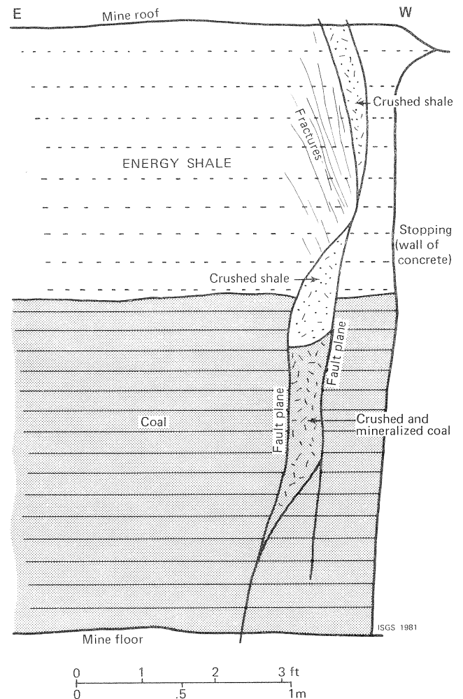
Figure 32. Cross-sectional view of the fault shown in figure 31. The graben form characteristic of many strike-slip faults is shown. The coal and shale between the two fault planes is thoroughly crushed and probably dropped into place during horizontal movement on the two fault planes. Both faults here display prominent horizontal slickensides and grooving, further evidence of strike-slip movement.
