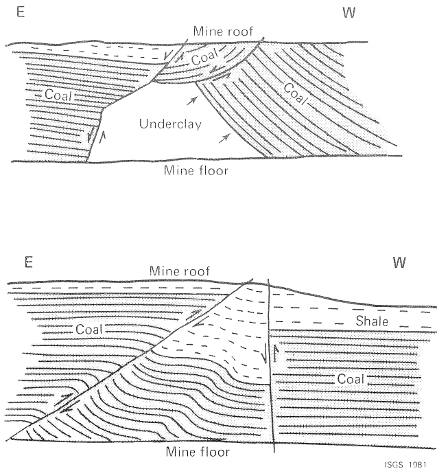
Figure 12. Faults in Mine No. 2, Western Coal Mining Co. Views looking south at two different places along the same NW-trending subsidiary fault. In the upper sketch, fault movement is geometrically normal yet the footwall is strongly folded upward as if by reverse movement. In the lower view, a nearly vertical normal fault and a low-angle reverse fault are parallel and juxtaposed. Such a close association of tensional and compressional features requires either two episodes of faulting and/or a large component of horizontal movement in the fault zone. (Field sketches by Gilbert H. Cady, ISGS mine notes, 1918.)
