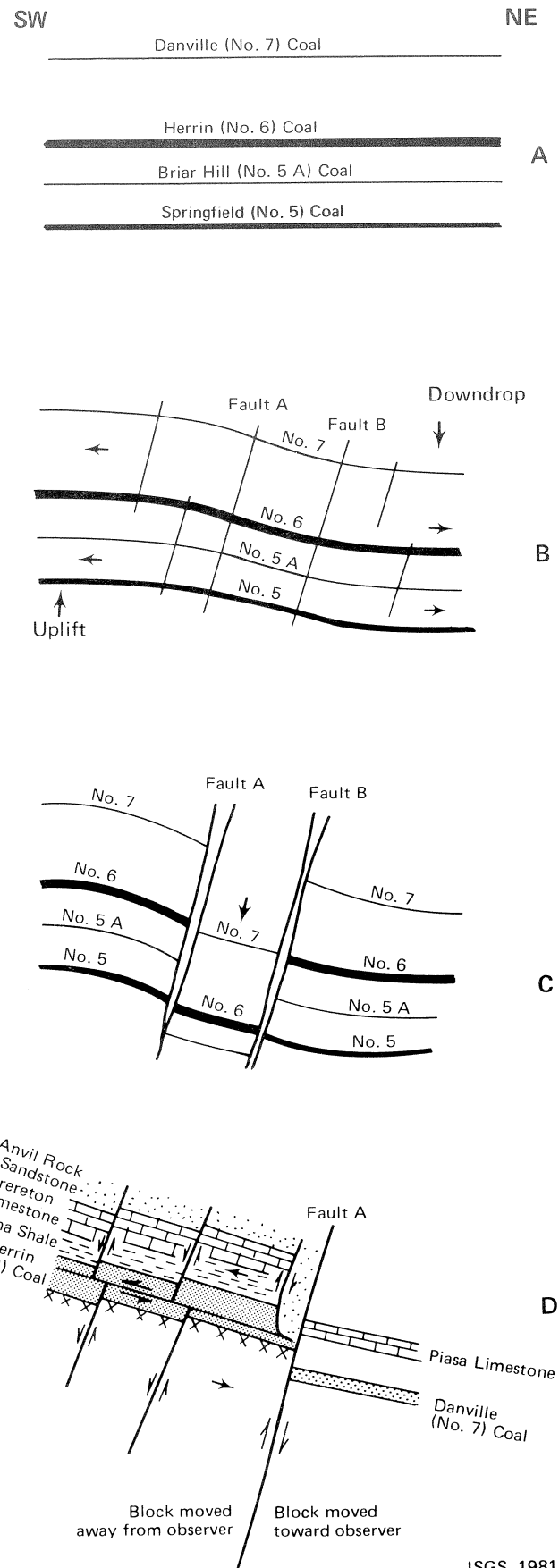
Figure 48. Hypothetical structural history of Study Area 5. (A) Horizontally-layered strata prior to deformation. (B) Initiation of uplift produces monoclinal fold (north limb of Pittsburg Anticline). At the same time horizontal extension produces southwest-dipping normal faults similar to those of Study Area 3. (C) Continued extensional stresses, perhaps accompanied by right-lateral wrenching, pulls the walls of Faults "A" and "B" away from each other, momentarily forming open voids along both faults. The block between the two faults subsides to produce a graben. (D) Detail of Fault "A" showing possible mode of origin of bedding-plane fault. When the walls of the fault pulled apart a slice of rock slid down and wedged in the void, blocking the upper part of the coal from coming back against the fault. The lower part of the coal and underlying strata were able to break free along a bedding plane and close the void below the down-dropped slice.
