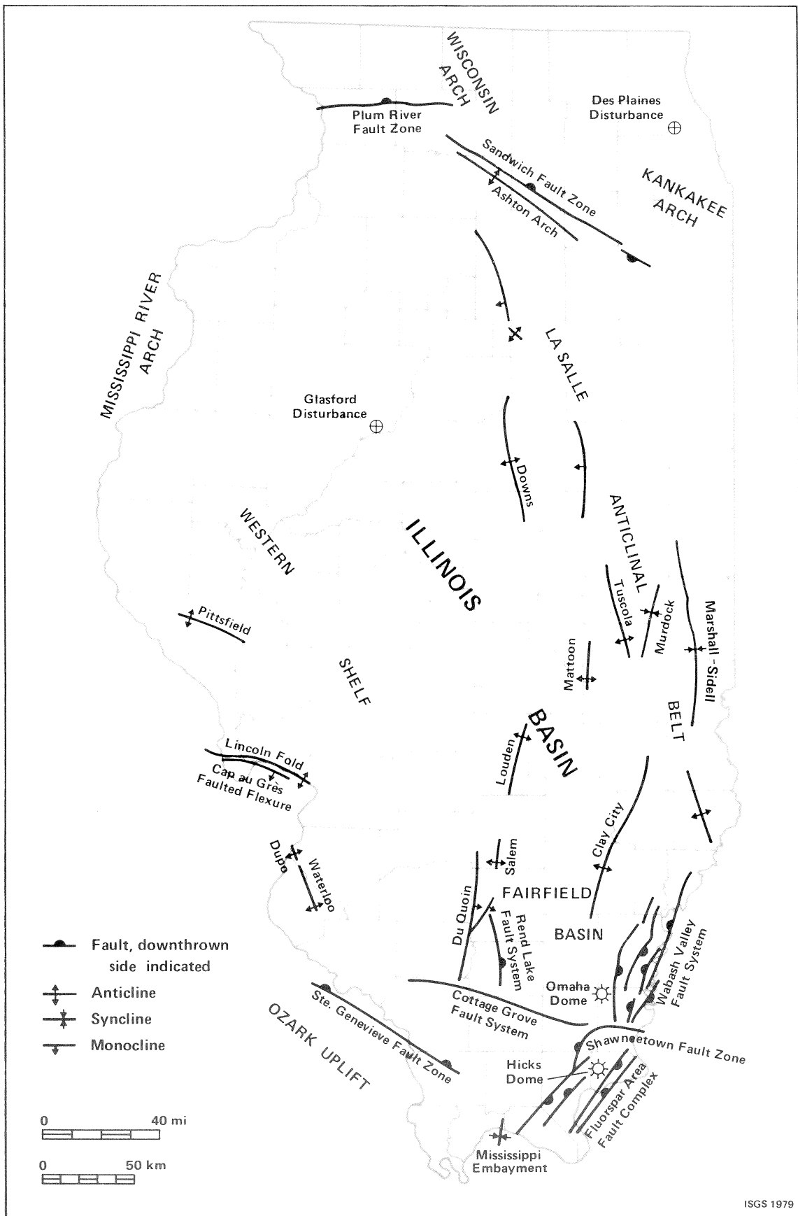
Figure 1. Major geologic structures of Illinois, compiled by Janis D. Treworgy, December 1979.
