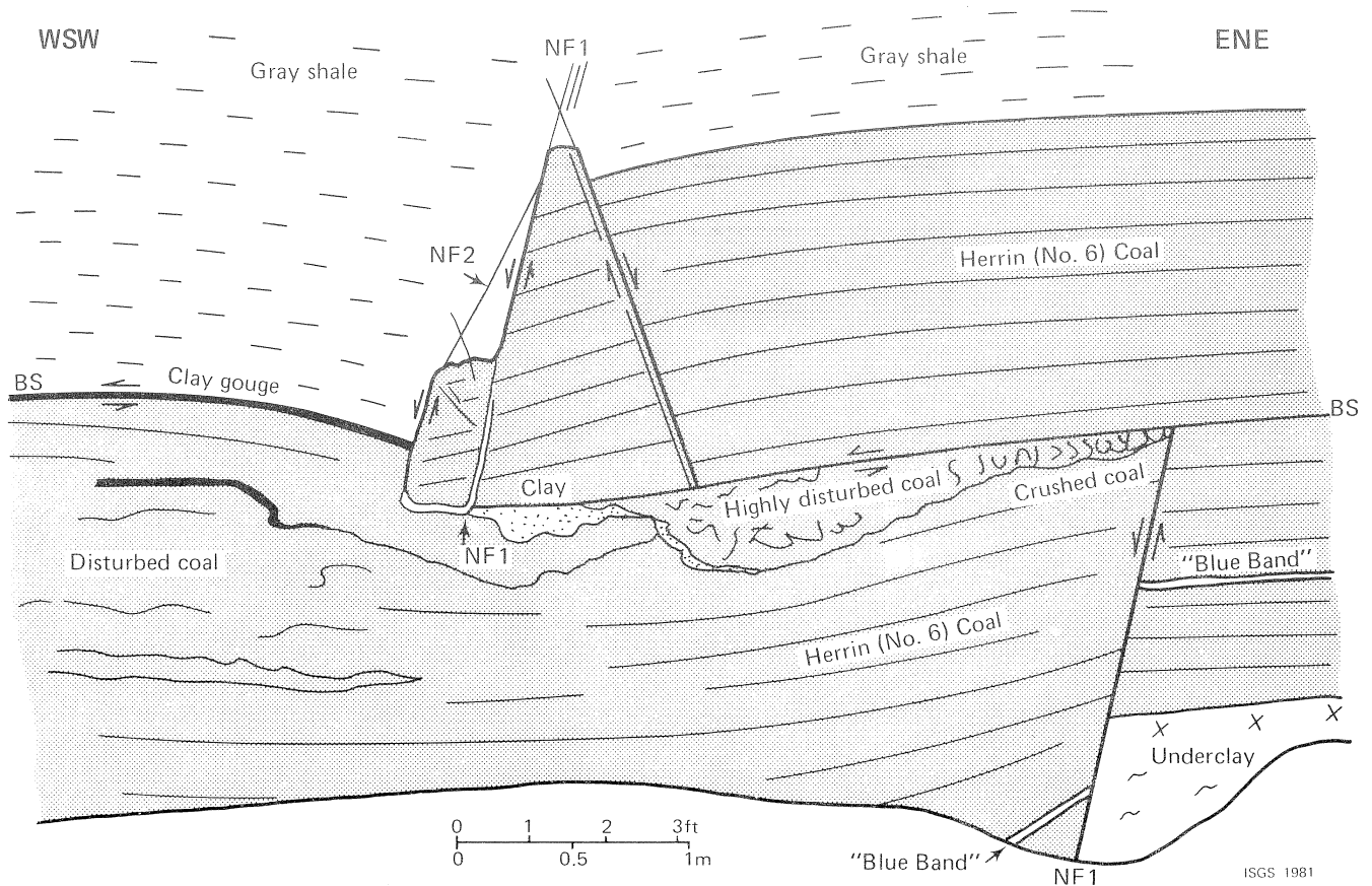
Figure 55. Vertical normal fault (NF1) offset by shearing parallel to bedding (BS). NF1 has about 3 feet (1 m) displacement and has been offset 10.6 feet (3.1 m) along BS. The upper block has moved from left to right. Shearing took place within the coal to the right of the normal fault and at the coal-roof contact to the left of the fault. The horizontal shear plane (BS) has itself been offset about 0.5 feet (0.15 m) by later movement on another normal fault (NF2).
