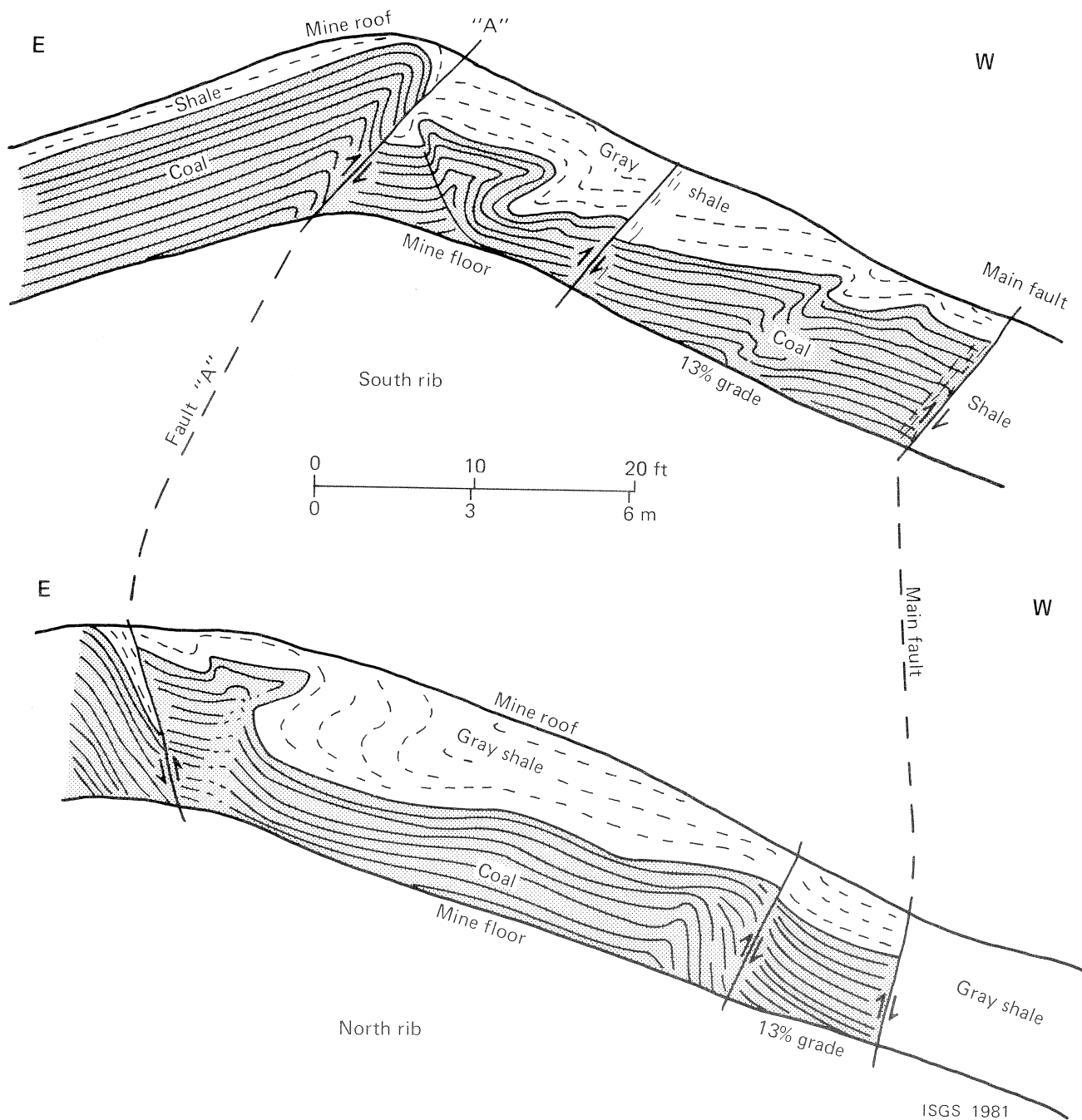
Figure 11. Faults in Old Ben Coal Co. Mine No. 17. Two sketches of the same fault zone on opposite sides of a mine entry. The zone trends southeast ( 150^\circ ) overall and the southwest side is downthrown about 28 feet (8.5 m). The main fault has consistent dip but Fault "A" dips to the east on the south rib (upper sketch) and to the west on the north rib (lower sketch). Fault "A" is a reverse fault on both sides of the entry. In the lower sketch note that the coal east of the fault is folded opposite the direction expected for drag. The geometry of Fault "A" virtually requires a component of strike-slip movement. (Modified from Cady, 1916.)
