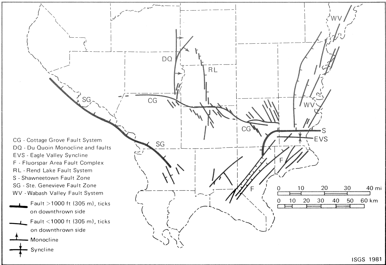
Figure 2. Major fault systems of southern Illinois.
