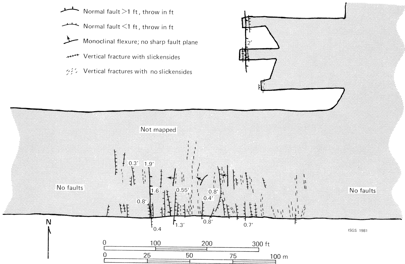
Figure 27. Faults in Study Area 2, Sahara Coal Co. Mine No. 21. Faults are trending nearly north-south and their throw decreases southward. About 1,000 feet (305 m) north of here, faults with up to 10 feet (3.1 m) displacement were encountered.
