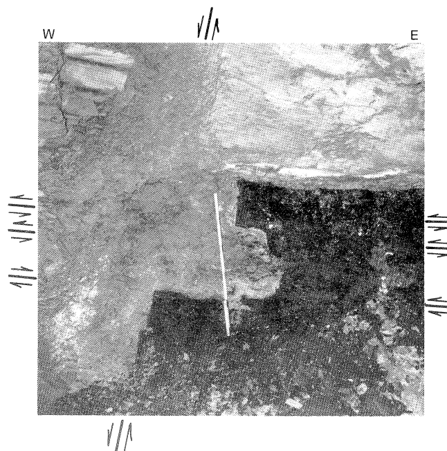
Figure 54. Fault "B" offset by multiple bedding-plane faults at location G, figure 49. Inconsistent direction of movement on horizontal faults has created a series of steps and overhangs. Ruler is 2 feet (0.6 m) long.
