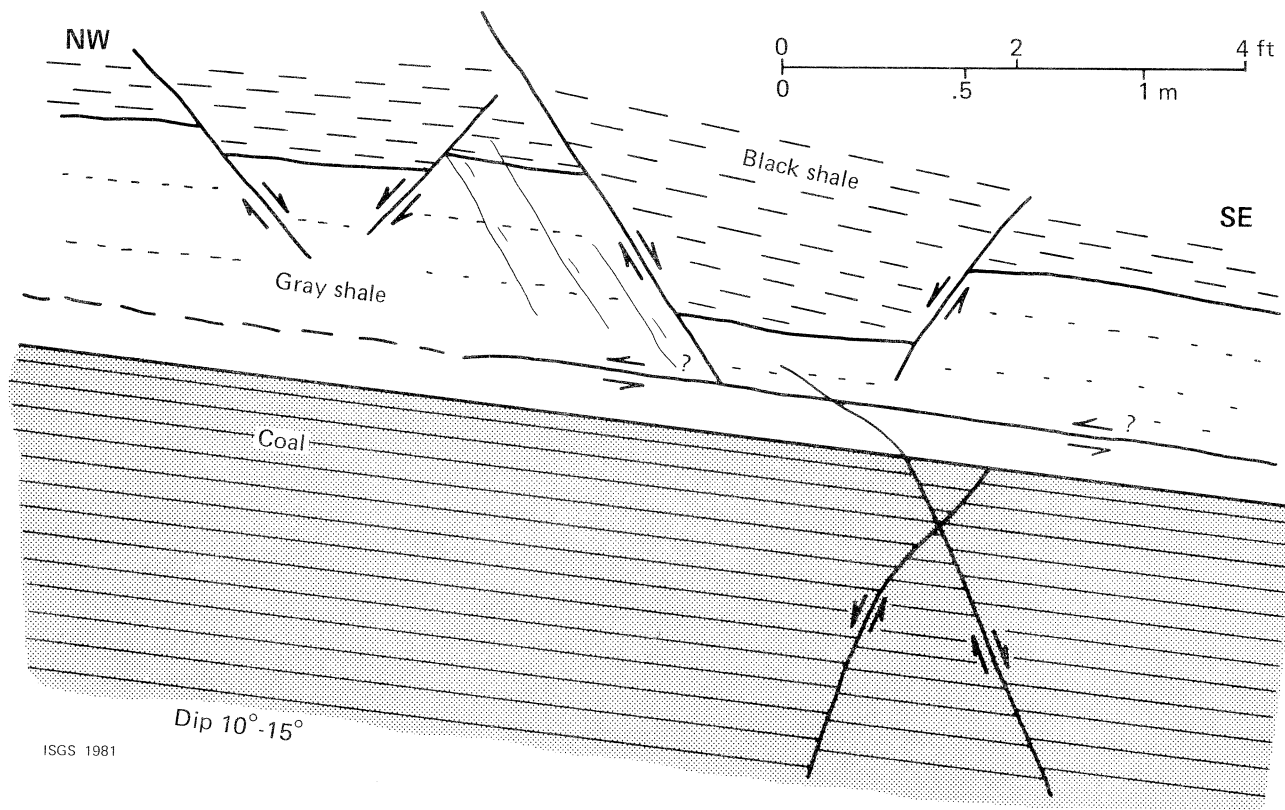
Figure 30. Slippage parallel to bedding at Location A in Study Area 3. Here the horizontal movement has taken place along a discrete shear plane in the Energy Shale. Normal faults are truncated and offset by the bedding-plane fault. The strata above the bedding-plane fault are believed to have moved updip to the northwest, but this could not be positively determined.
