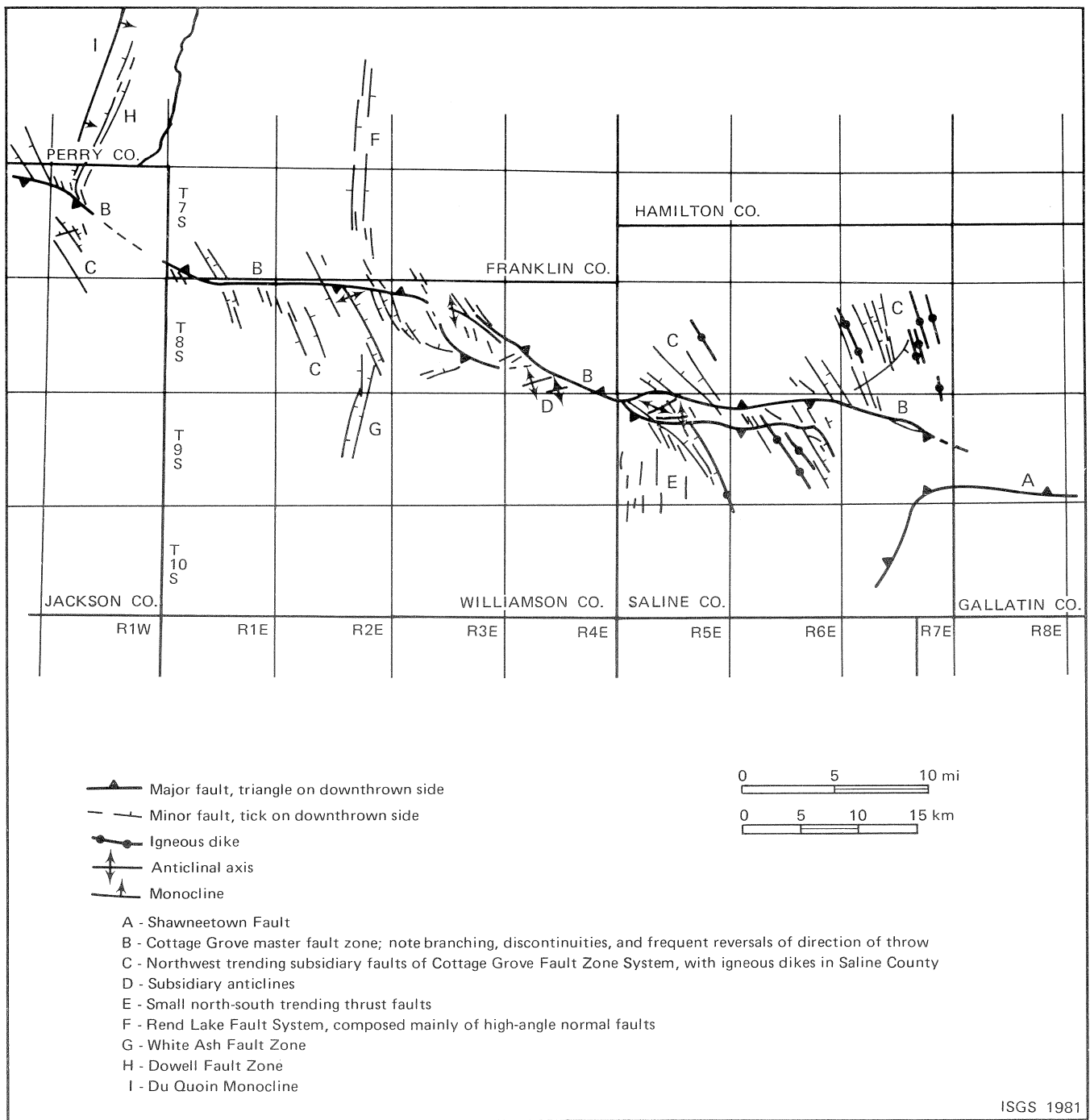
Figure 4. Cottage Grove Fault System and associated structures.
