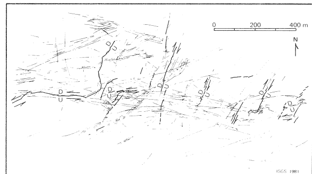
Figure 20. Pattern of ground fractures near eastern end of Dasht-e Bayaz fracture zone. The "master fault" becomes discontinuous, and most of the stress has been relieved through right-lateral slippage along NNE-trending conjugate faults. While the Cottage Grove Fault System contains no direct analogies, small conjugate strike-slip faults have been observed in coal mines (see fig. 51). Reprinted by permission of the Geological Society of America and Tchalenko and Ambraseys, 1970.)
