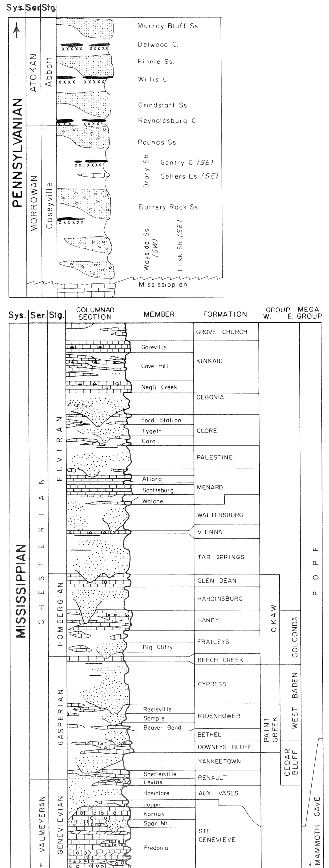
Figure 3. Generalized stratigraphic section of bedrock units along Cottage Grove Fault System. Units below Ste. Genevieve Limestone are rarely penetrated by drilling and are poorly known. Pennsylvanian section (after Willman et al., 1975); Mississippian section (after Swann, 1963).
