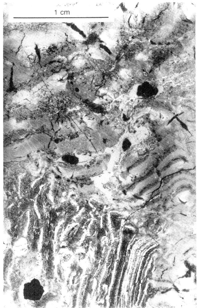
Figure 8 Negative print of thin section of a nodular paleosol from upper Fraileys/Big Clifty in Caldwell County, Kentucky. Note laminated intraclasts, brecciation, and desiccation cracks.
