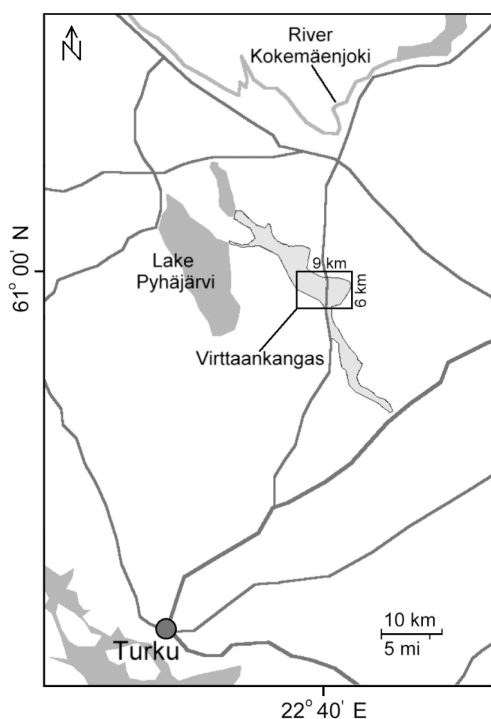
Figure 1 Shaded areas in and outside the Virttaankangas study area (top) represent the largest esker complexes in southwestern Finland.
