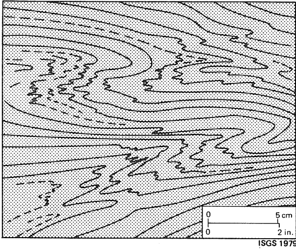
Figure 30. Small irregular (disharmonic) recumbent folds (soft-sediment deformation) in Herrin (No. 6) Coal, often found in association with gray shale rolls in the coal, but also found independently in coal. Location: "Quality Circle," southern Illinois, mine B.
