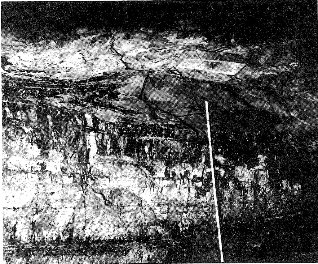
Figure 33. Roll of medium-gray shale of the Energy Shale intruded into top layers of Herrin (No. 6) Coal. Toe (at the left) splits folded coal strata into several stringers. Tail has been truncated by compactional normal fault (at the right). The rod is about 4 feet (1.2 m) long. Location: "Quality Circle."
