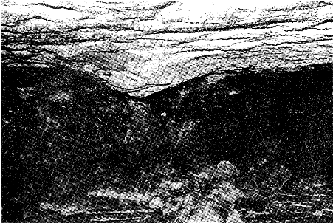
Figure 86. Large limestone "boss" above Herrin (No. 6) Coal has deformed and truncated the top beds of the coal seam. Anna Shale is absent, and the Brereton Limestone ("boss") directly overlies the coal. Location: west-central Illinois, mine S.
