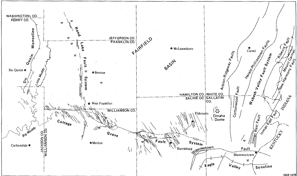
Figure 59. Major fault systems and structures in southern Illinois. (After Stonehouse and Wilson, 1955.)
