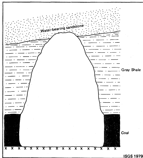
Figure 160. Wet zones in Energy Shale. Where seepage in the roof is locally encountered, large arched falls are common. The low shale durability of the gray shale in wet conditions can decrease roof support by bolts considerably. Both mechanical anchors and resin bolts have locally proved ineffective in areas of abundant seepage. Bolts fall with the rock.
