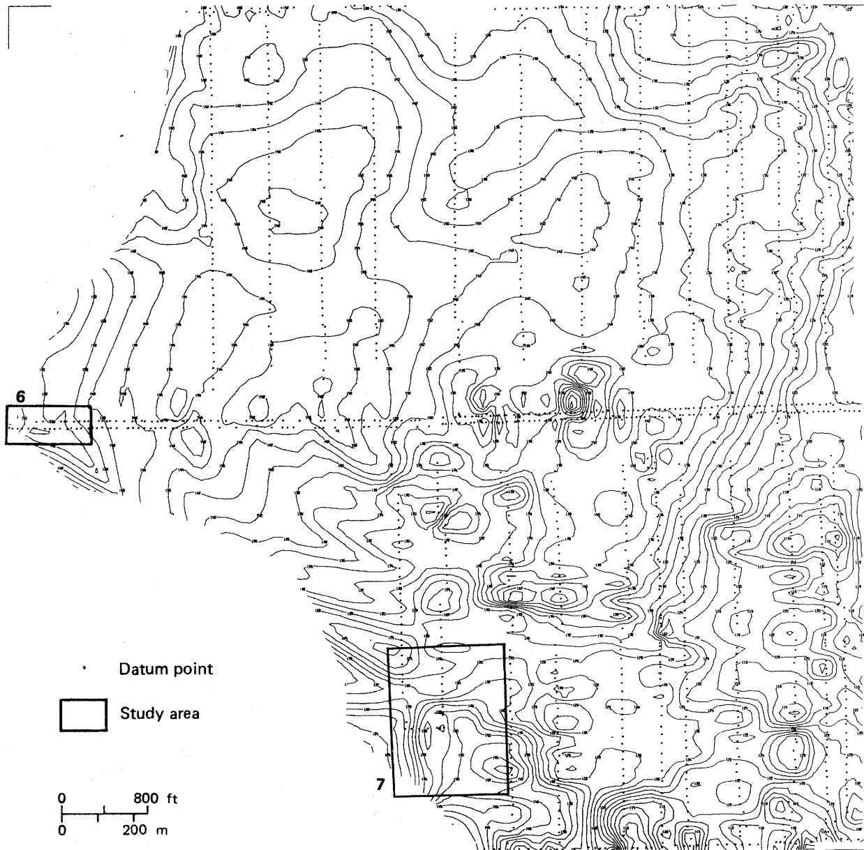
Figure 144. Computer-generated map of the top of the Herrin (No. 6) Coal at mine C, study areas 6 and 7. For the more regional setting, see figure 149. Structural anomalies of the top of the coal reflect anomalies in the roof strata composed mainly of laminated siltstone and sandstone, which locally impose severe problems for roof control. Contour interval: two feet; grid size: 100 feet.
