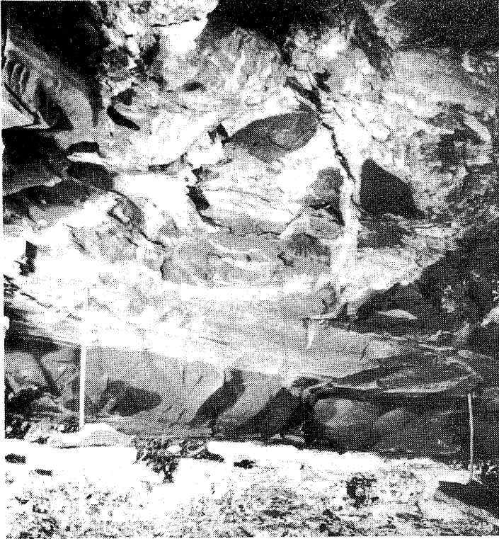
Figure 81. Unusual roof sequence above the Herrin (No. 6) Coal up into the Lawson Shale. Soft black shale overlying the coal (which is rock dusted); sharp contact to soft, medium-dark-gray shale, which is itself subjacent to an intensively altered very soft, greenish, medium- to light-gray shale with syneresis cracks. There is no proof whether the black shale is of the Anna Shale or of the lower portion of the Lawson Shale. Location; mine F in east-central Illinois.
