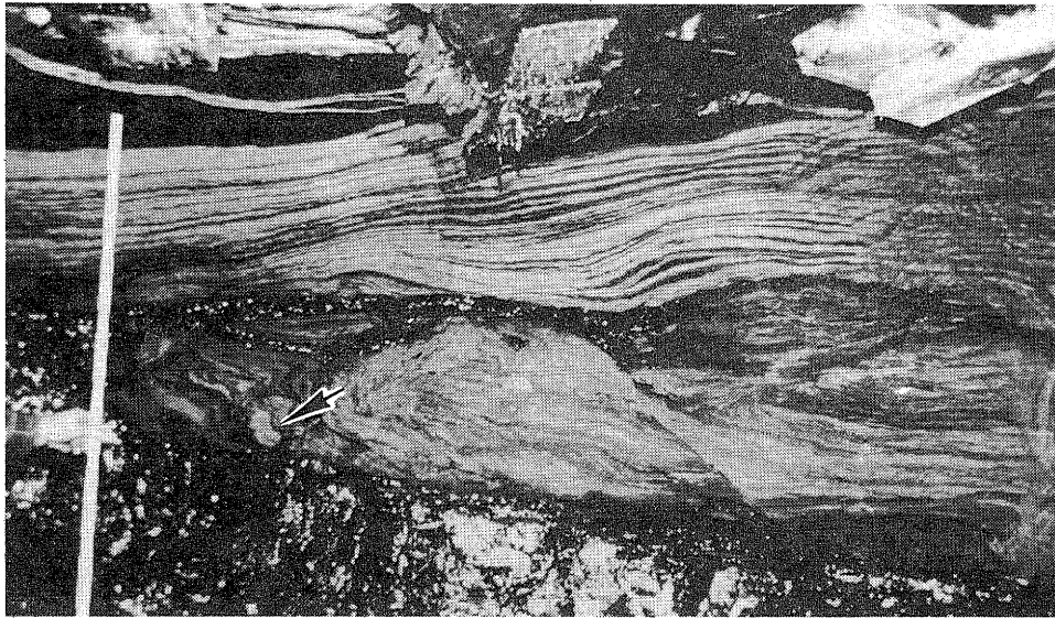
Figure 38. Roll in planar-bedded siltstone and sandstone of the Energy Shale Member. Near the toe of the roll (arrow), recumbent soft-sediment folds and low-angle shear planes are visible. These features suggest that the silt and sand filling the roll intruded from right to left between the layers of peat. (Note the coal "rider" originating at the toe and extending almost entirely over the roll.) The large low-angle slips at the tail of the rolls may have formed later by differential compaction.
