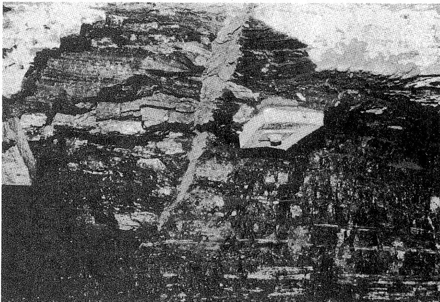
Figure 44. Small clay dike associated with even smaller clay-dike faults under gray shale roof. Clay dikes under gray shale roof are rare. False drag of the bedding is found in the immediate vicinity of the faults. Location: southern Illinois, "Quality Circle," mine B.
