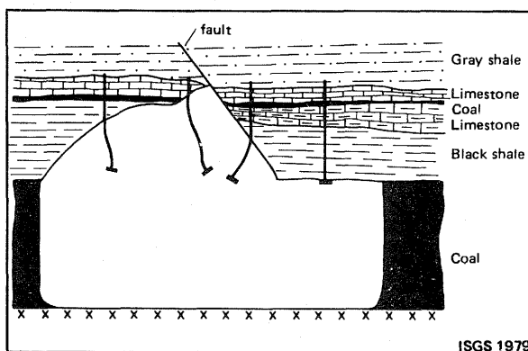
Figure 162. Black shale or "draw slate." Numerous falls occur, and their number is proportional to the number of faults, and slicksided surfaces. Where the Brereton is thin or absent, roof strata up to the next thick limestone will usually fall. If falls do not stop at the second (Conant) limestone, the Lawson Shale up to the Bankston Fork Limestone (6 to 10 feet above the coal) will usually fall.
