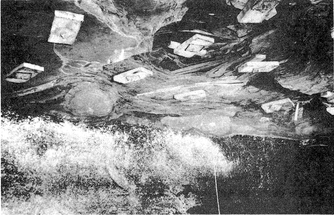
Figure 26. Concretions in gray shale roof usually are not as spherical as those in the Anna Shale. These concretions in combination with planar-bedded silty shales and siltstones are a hazard to miners. Note the thin gray shale of the Energy Shale underneath black Anna Shale, above the Herrin (No. 6) Coal. Location: mine E, southwestern Illinois.
