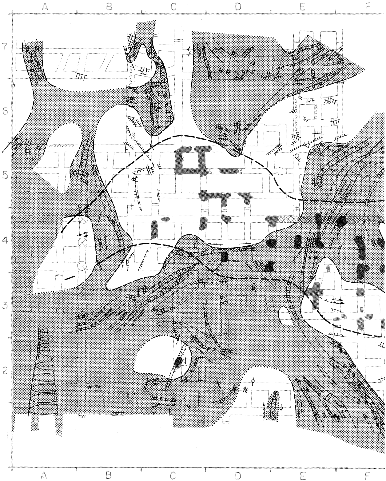
Figure 140. Distribution of soft-sediment rolls associated with minor faults in relation to the lithology of the immediate roof and roof falls of Herrin (No. 6) Coal in study area 5 of mine B. The map displays the close interdependence of soft-sediment structural features, mainly rolls and slips, with distribution and lateral boundaries of the Energy Shale roof strata. Although the immediate roof in areas of medium-gray shale with rolls and slips commonly is very rough and irregular, the roof falls are more abundant in areas of dark-gray shale. Roof falls in areas of medium-gray shale occur mainly within the shear body.
