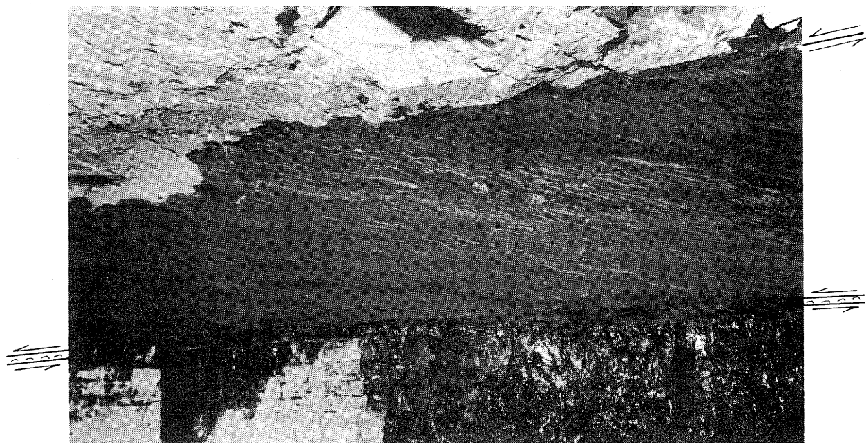
Figure 47. Finely laminated silty shale with numerous small, narrowly spaced, low-angle normal faults in the "shear body." Two major shear surfaces border the sheared block. One major shear surface is almost horizontal and is oriented parallel to the bedding. It forms the immediate coal-roof contact, but also truncates the inclined laminations of the silty shale. The coal itself is not visibly affected by the deformation. The second major shear surface runs about parallel to the many small faults in the laminated shale just below the rock-dusted (white) portion of the roof. Location: southern Illinois, "Quality Circle," mine B.
