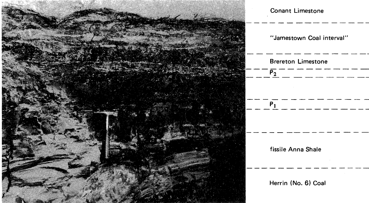
Figure 65. Section of immediate roof strata, black shale-limestone roof type in mine A (west-central Illinois). The Conant Limestone (top of photo) is underlain by streaks of Jamestown Coal, with freshwater limestones and some lenses of Brereton Limestone, which in this section is very lenticular and discontinuous. Anna Shale can be subdivided into three lithologic subunits: (1) poorly bedded, strongly mottled, weak, very dark gray shale with upper band of phosphatic nodules ( P_2 ), (2) weak, poorly bedded, less mottled, very dark gray shale with lower band of phosphatic nodules ( P_1 ), and (3) black fissile ("slaty") shale with concretion. The Herrin (No. 6) Coal is lowermost.
