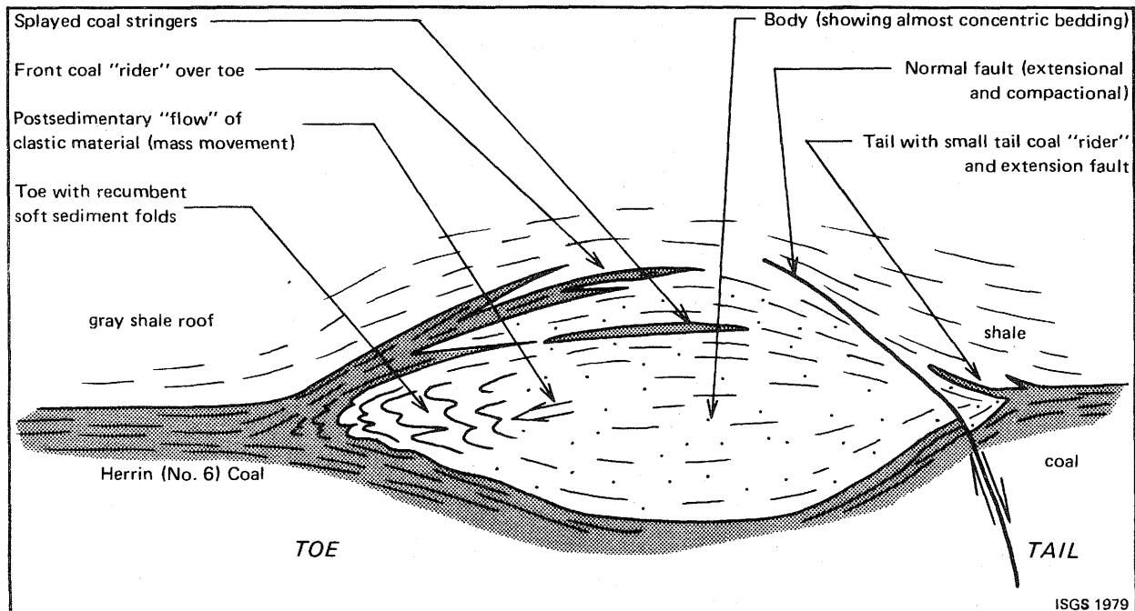
Figure 29. Sketch of typical roll (soft-sediment protrusion of clastic materials into surrounding sediments—coal, shales, siltstones, and sandstones).
