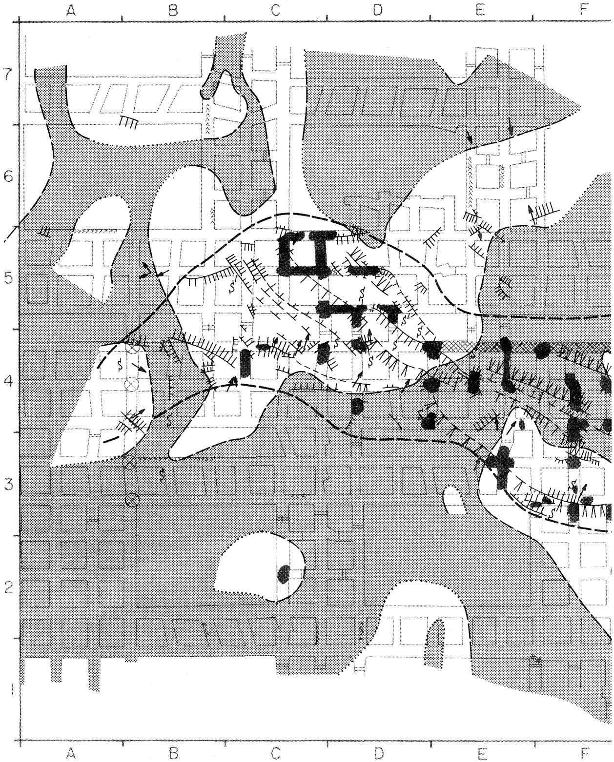
Figure 141. Outline and major shear structures of the shear body in study area 5 of mine B. Roof falls have occurred most often in the area of the shear body and to a lesser degree under dark-gray shale in the immediate vicinity of the shear body. Deformational features older than the shear body have not been drawn on this map, but can be compared in their interrelationship to lithologic differences in figure 140. The shear body is not restricted to a particular lithology, but affects dark-gray shale and medium-gray shale and, locally, the top of the Herrin (No. 6) Coal as well.
