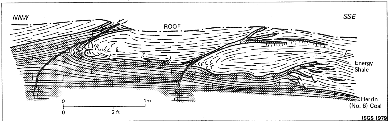
Figure 34. Soft-sediment deformation of Energy Shale protruding from the roof and producing rolls. Note the riding coal stringers that have been split off from the seam, the folded toes of the rolls and the coal in front of it, and the low-angle normal faults that steepen downward and dissipate into the coal as "goat beard." Location: "Quality Circle," southern Illinois, mine B.
