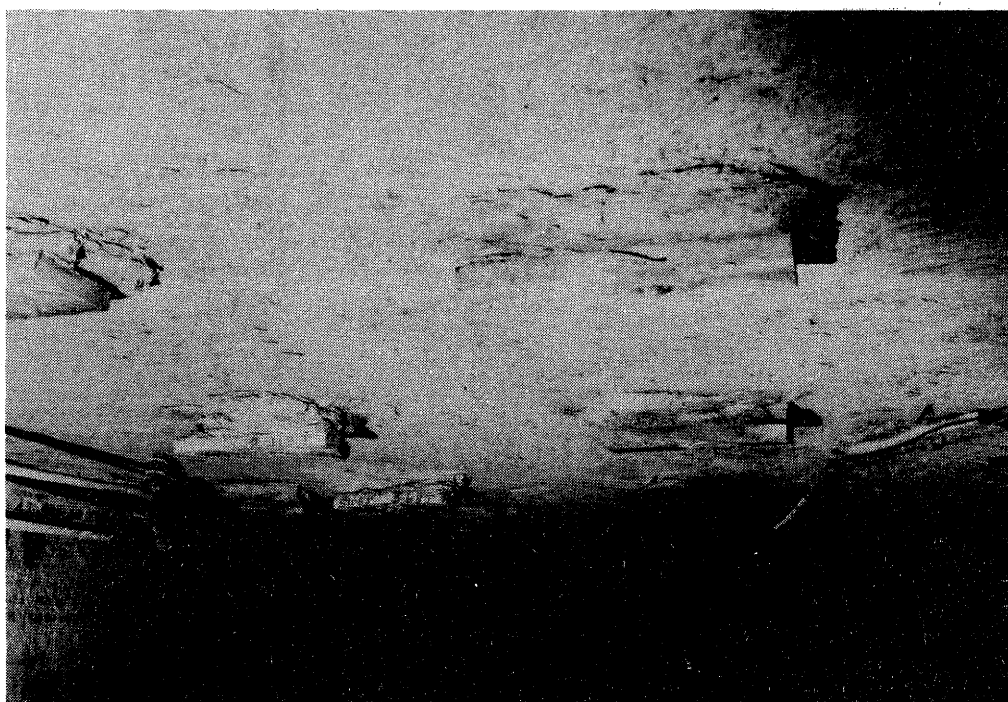
Figure 72. Limestone of the Brereton forms stable roof. About the lowest 3 inches (7 to 10 cm) of soft flaky "clod" have fallen, except above the header boards. Location: mine A, west-central Illinois.
