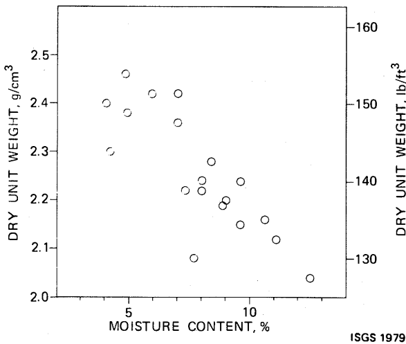
Figure 166. Moisture-density relation in shales and underclays of the Carbondale Formation, Pennsylvanian System, in the Illinois Basin Coal Field. Sample depth, about 300 feet (91 m). Data from Ganow, 1975.
