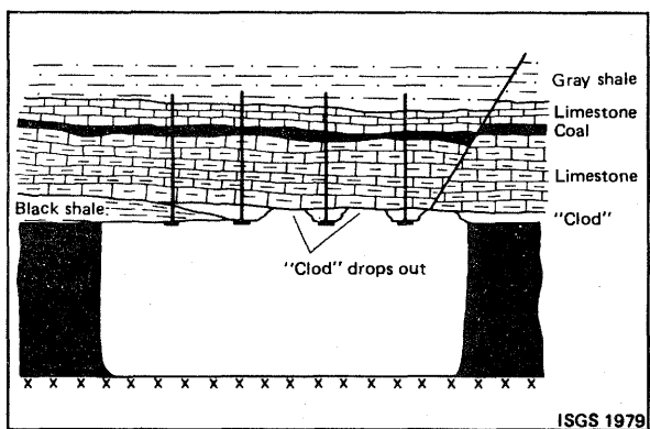
Figure 161. Limestone roof. Best roof conditions are found where the Brereton Limestone is greater than 1.5 to 2.0 feet (0.4 to 0.6 m) in thickness. Bolts are probably not supporting the roof but are merely inhibiting slabbing of the "clod." The crumbling and slaking quality of the "clod" in a number of mines led to unnecessary cribbing.
