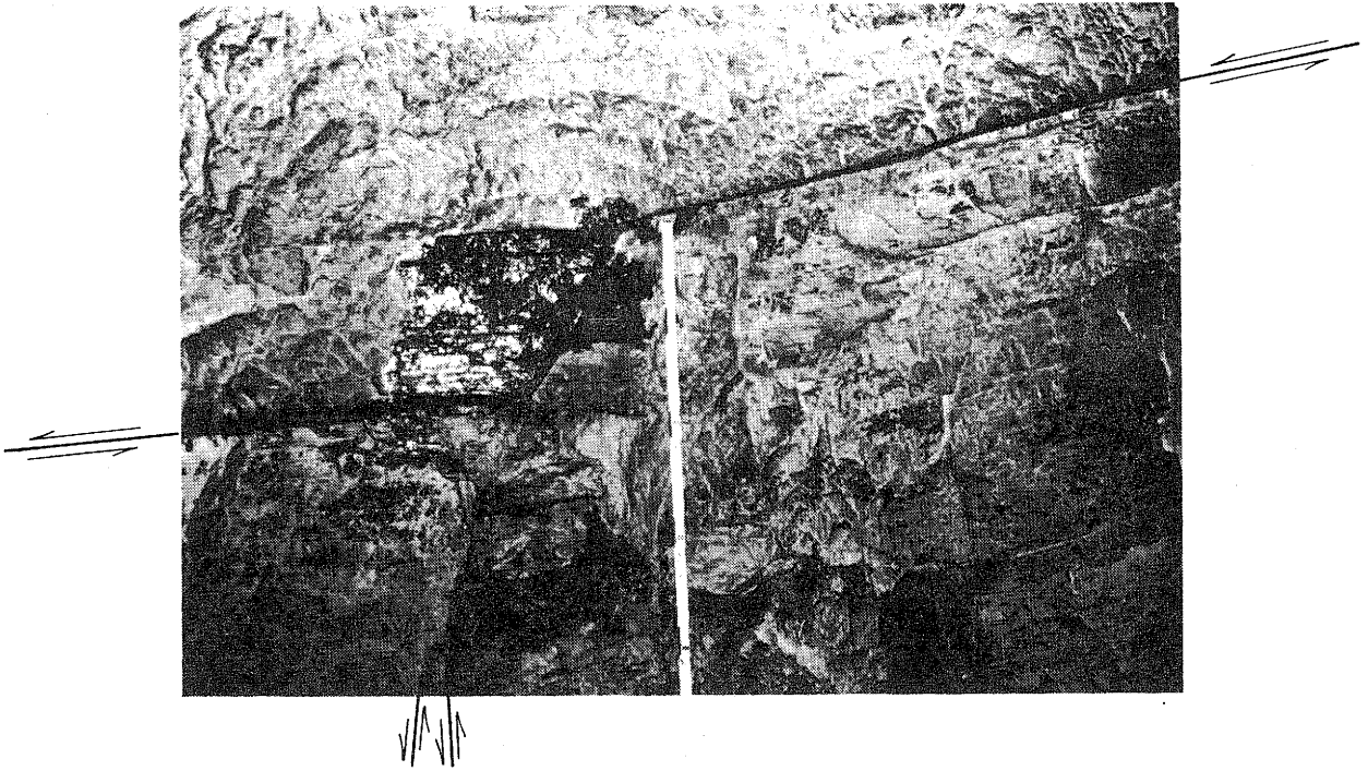
Figure 46. Shear plane parallel to bedding in Herrin (No. 6) Coal appears to have offset a high-angle normal fault and later to have been offset itself along the lower branch of the same high-angle normal fault. Location: southern Illinois, "Quality Circle," mine C.
