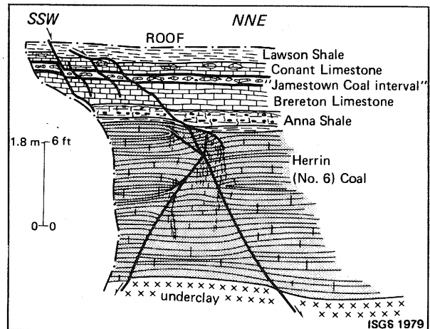
Figure 94. Clay-dike faults dissecting the Herrin (No. 6) Coal and associated rock strata. The faults result not from vertical movements, but mainly from horizontal extension of the strata, as indicated by collapsed graben-like structures in the upper coal benches and rebound horst-like structures in the underclay and lowest coal benches. Note the convergence of the coal bedding in places, the en echelon extension fractures ("goat beards") and the splitting and downward steepening of the faults in the coal seam. Location: mine A, west-central Illinois.
