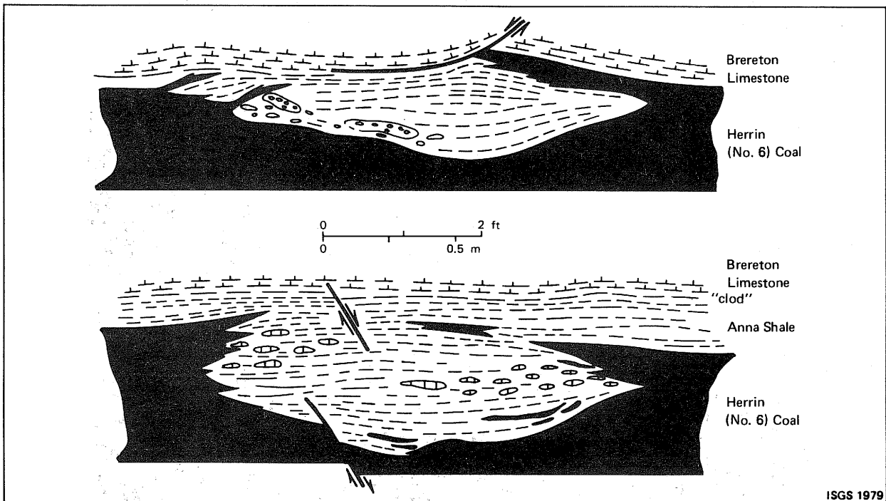
Figure 74. "Washouts," lenses of impure black slaty shale with abundant coal stringers and phosphatic lenses, contain irregular nodules and pockets of brecciated brown limestone in brown shaly matrix. These features are small and uncommon within the top layers of the coal seam below black shale-limestone roof. They are similar to rolls found under gray-shale roof. Location: mine A, west-central Illinois.
