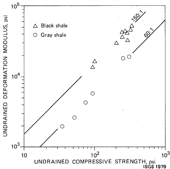
Figure 171. Comparison of deformation modulus and compressive strength, both undrained, of shales from the Caseyville Formation, Pennsylvanian System, in the Illinois Basin Coal Field. Data from Hendron et al., 1970.
