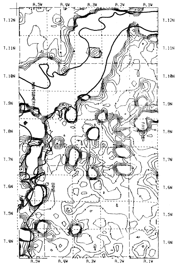
Figure 156. Thickness trends of the interval from the Herrin (No. 6) Coal Member to the first thick limestone bed ( > 2 feet) in Bond and Montgomery Counties. Contour interval: three feet; highest contour allowed: 15 feet. Areas having \geq 2 miles between data points: 7N-1W, 6N-1W, 5N-1W, 4N-1W, 11N-4W, 11N-3W, 10N-5W. Greater data-point density was used to outline areas of thin, split, or missing coal.
