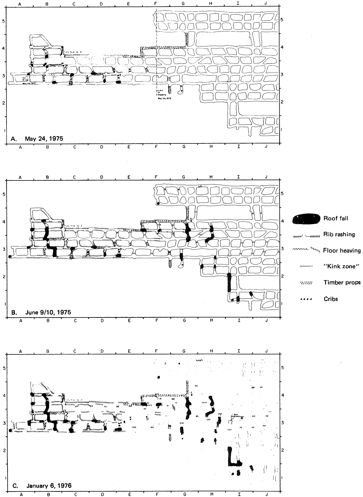
Figure 146. Occurrence and development of roof falls in study area 6 of mine C as mapped during three different periods. Although excavation did not continue, the roof continued to fall for more than half a year.
