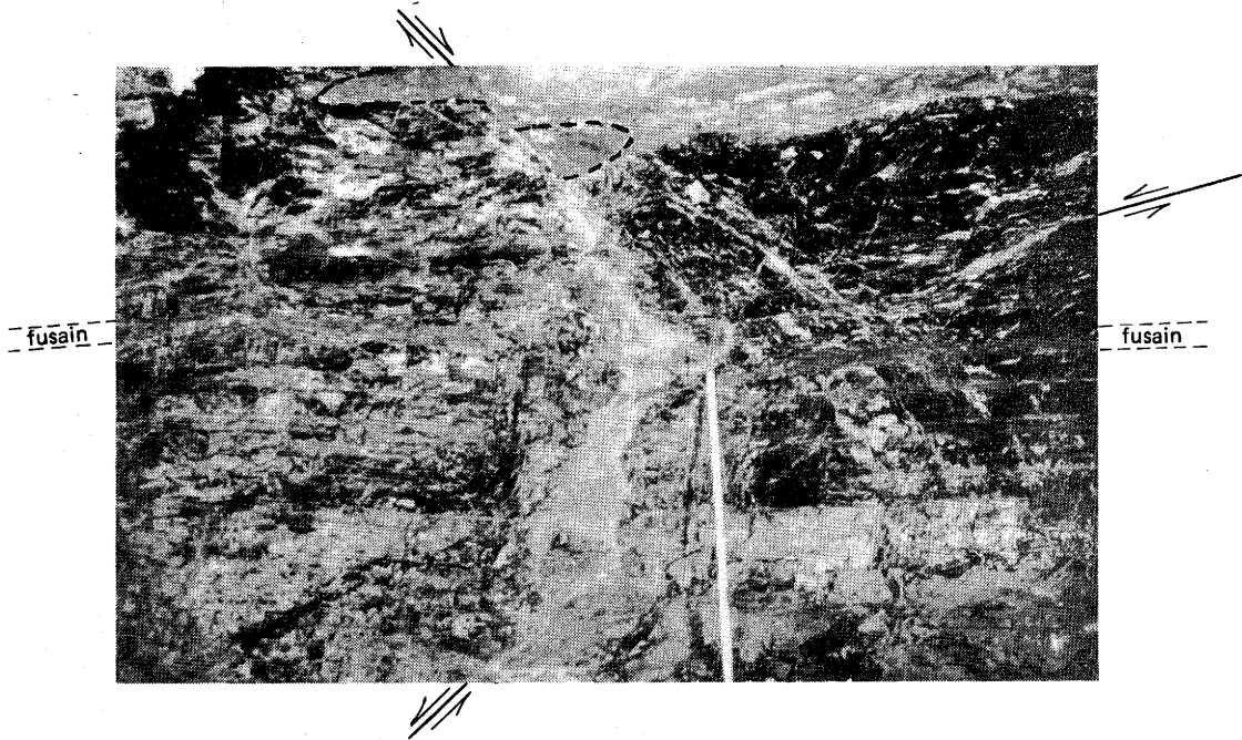
Figure 110. Complex clay dike in the Herrin (No. 6) Coal. Roof is Brereton Limestone which is displaced downward to the east. Fusain layer in the center of the coal seam is bent downward east of clay dike, fractured within the clay dike, and offset immediately west of the dike. Note the associated small low-angle clay dike faults and the numerous extension fractures and "goat beards," and the coal fragments in the clay matrix. Location: study area 1, mine A, west-central Illinois.
