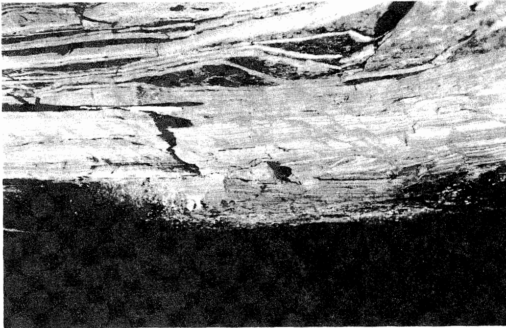
Figure 19. Roof fall in planar-bedded laminated siltstone of the Energy Shale Member. Many bedding surfaces are coated with coalified plant debris and mica. The diagonal (inclined 45°) dark stripes in the lower rock layers probably are water- or gas-escape structures. Location: east-central Illinois, mine D.
