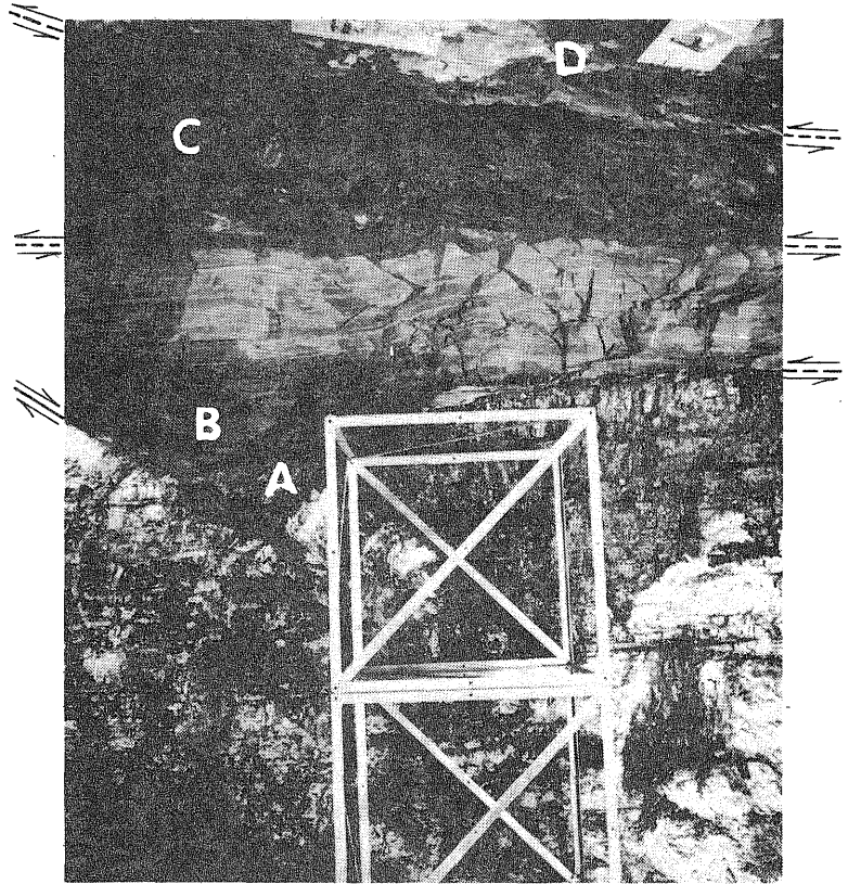
Figure 52. Nearly horizontal shear zone of a set of shear surfaces enclosing dragged, folded, and sheared dark-gray shale; main shear movement of each upper shear bed is toward the left and has truncated the top of a major roll of silty, medium-gray shale. This truncation indicates that formation of the shear body continues after or even postdates formation of rolls; however, small low-angle antithetic faults penetrate the shear zone of dark-gray shale and remnant of roll, so these postdate both roll and shear zone. Section from bottom of photo to top: (A) coal slightly deformed by fault in roll (left side of photo), (B) laminated silty shale within the roll, (C) folded, sheared, and intensively contorted dark-gray shale in shear zone, and (D) greenish claystone of main shear body. Location: southern Illinois, "Quality Circle," study area 5, mine B.
