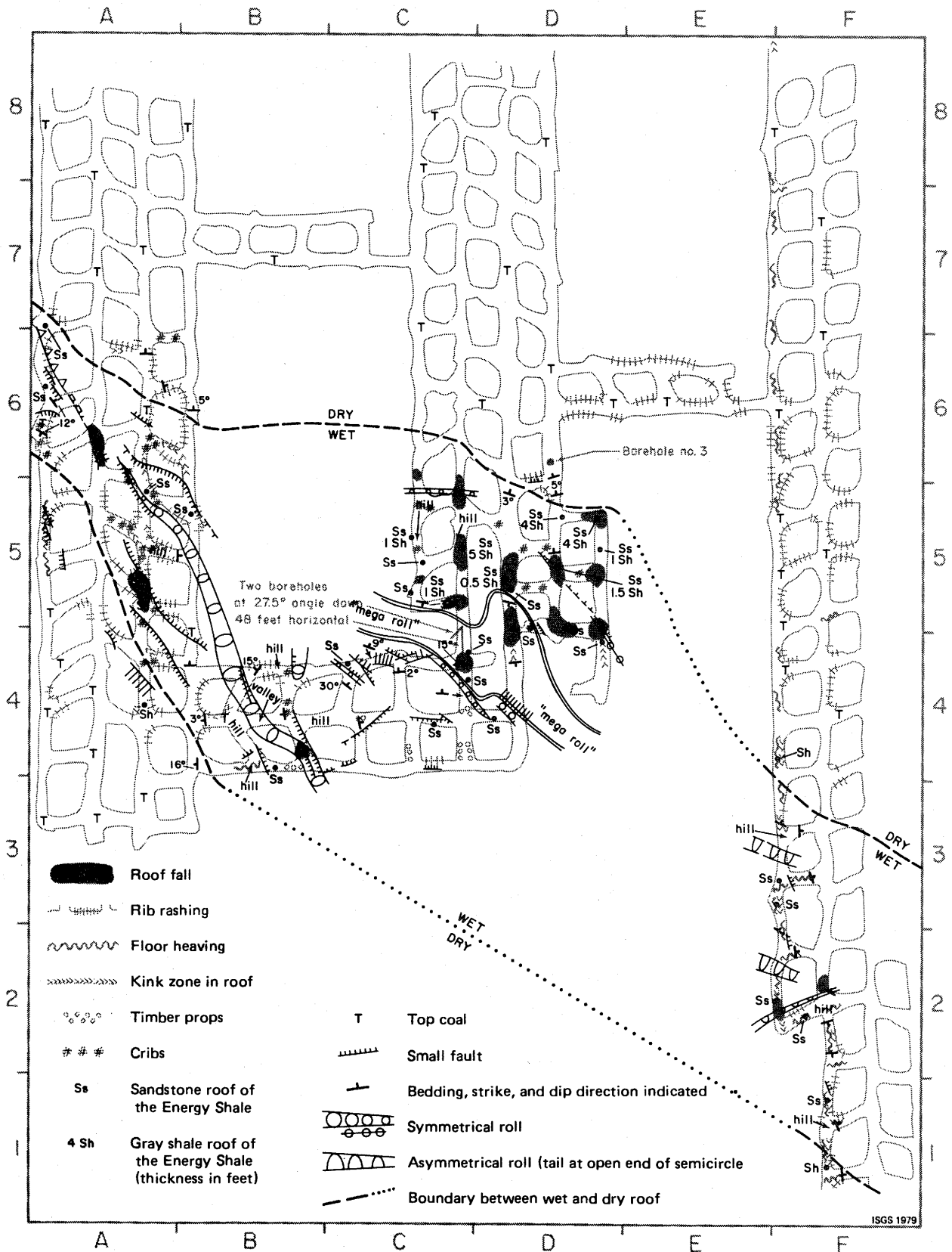
Figure 148. Lithology, rolls, and fault structures of the Herrin (No. 6) Coal and its immediate roof strata, and the distribution of roof falls and other induced instabilities and additional roof support in the area below siltstone and sandstone with water seepage. Study area 7, mine C.
