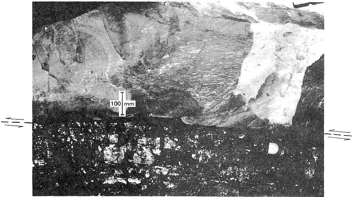
Figure 53. Microfaulted laminated silty shale and siltstone. Low-angle and high-angle shear planes are adjacent and are of a single deformational action. The microfault pattern resembles the lower portion of seismites described by Seilacher (1969). Mass movement in general is downward, and each lower portion has moved laterally toward the south (left in photo). Major shear plane is subparallel to bedding just above coal. Coal itself is affected only at very top. Location: southern Illinois, "Quality Circle," study area 5, mine B.
