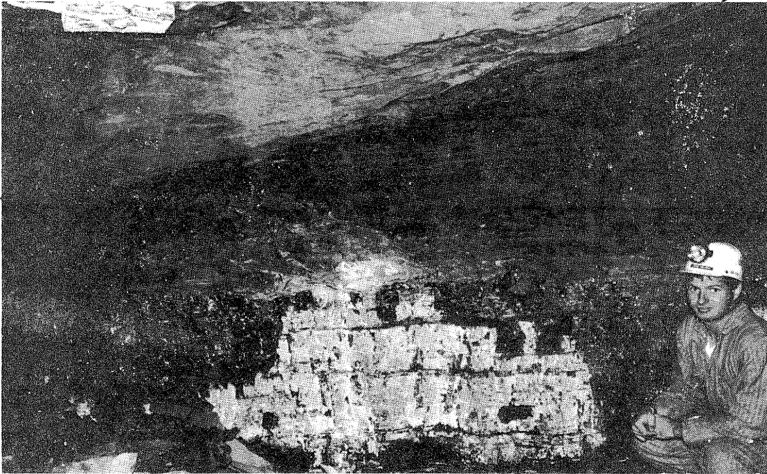
Figure 48. Almost undisturbed Herrin (No. 6) Coal and some beds of finely laminated silty shale truncated by a northward-dipping (to the left) set of major shear surfaces and overlain by the shear body. Location: southern Illinois, "Quality Circle," mine B.
