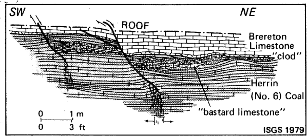
Figure 101. Low-angle normal faults (clay-dike). Faults displace Brereton Limestone and top of Herrin (No. 6) Coal, steepen downward in the coal, and dissipate in form of numerous echelon extension fractures. In places coal shows false drag. Horizontal extension is achieved by dip slip on faults in the Anna Shale and top coal and mainly by the extension fractures ("goat beards") in the coal seam. Note the displacement of "bastard limestone." Location: mine A, west-central Illinois.
