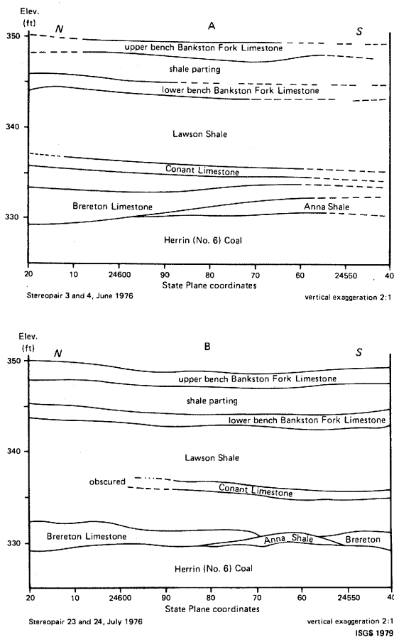
Figure 64. Cross sections from photostereopairs from close-range photogrammetric mapping (see fig. 63) show the position and variation in thickness of the stratigraphic members above the Herrin (No. 6) Coal and their interrelationship. As the highwall advanced, stereopairs were taken repeatedly with the intention of interpolating from section to section to produce a three-dimensional map of the rock bodies. A is from a photo taken in mid-June 1976; B is from a photo taken in July 1976. Location: highwall of mine E in south-western Illinois.
