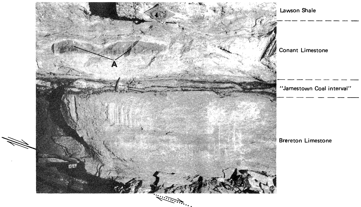
Figure 78. Jamestown Coal between well-developed Brereton and Conant Limestones. The "Jamestown Coal interval" is reduced to a few thin partings of dark, very carbonaceous shales and nodular irregular limestone lenses. Note the dark-brown dolomitic concretionary lenses (A), which are characteristic of the Conant Limestone. The Lawson Shale (top of photo) is exceptionally thin (2 feet; 0.6 m) at this location and is intensively mottled. Location: mine A, west-central Illinois.
