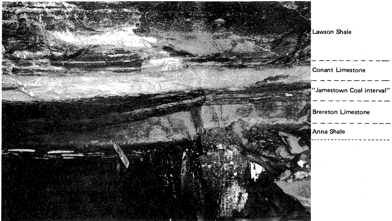
Figure 73. Wedging relationship of roof rock layers; both the Anna Shale and the Brereton Limestone pinch out (toward left side of photo). The "Jamestown Coal interval" has thin coal streaks and contributes to bedding separation. The overlying Conant Limestone is too thin to bridge stresses from one pillar to the next. The Lawson Shale is soft and mottled and contains numerous low-angle shear planes and syneresis cracks. Location: mine A, west-central Illinois.
