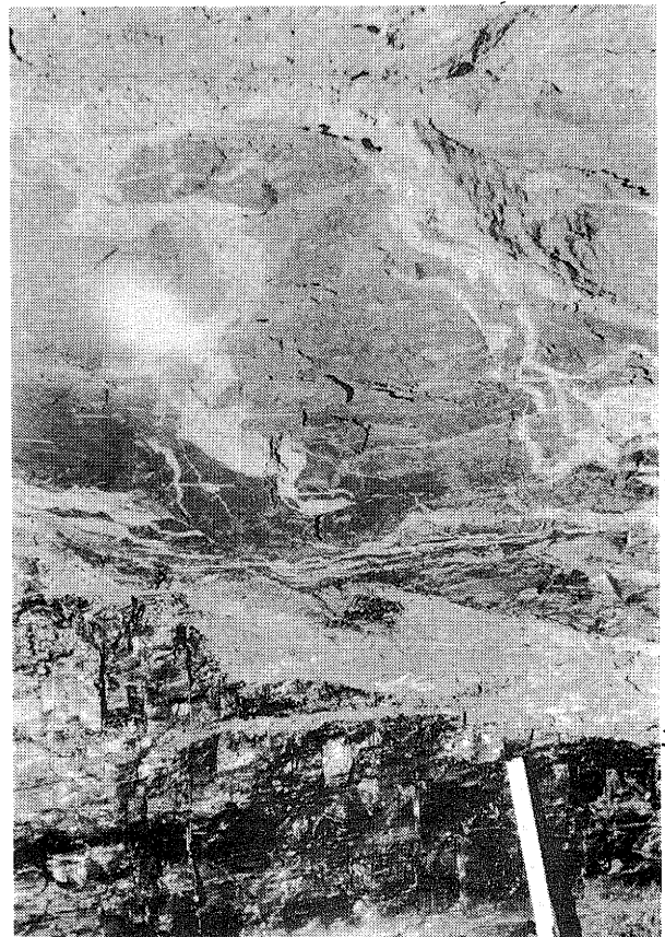
Figure 115. Very low angle clay dike along clay-dike fault which truncates and displaces Herrin (No. 6) Coal and Anna Shale. Anna Shale is intensely altered and is cut by numerous small irregular clay dikes and clay sills. Note angular interface of the coal and the clay dike and coal fragments in clay dike. Location: mine A, west-central Illinois.
