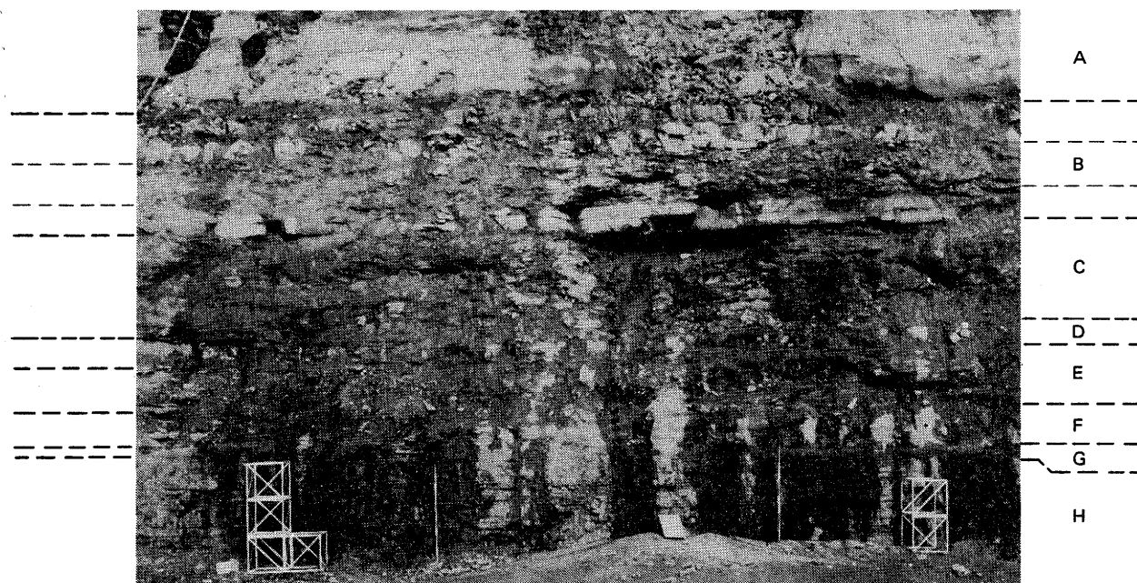
Figure 63. Cross section in black shale-limestone roof: (A) interval of the Piasa Limestone Member and the unnamed gray, green, ocher, and varigated shales below, (B) Bankston Fork, with two limestone horizons, (C) greenish gray mottled and dark gray Lawson Shale, (D) Conant Limestone, (E) shales, argillaceous limestones, dark-gray carbonaceous shales ("Jamestown Coal interval"), (F) Brereton Limestone (lenticular), (G) Anna Shale (lenticular), and (H) Herrin (No. 6) Coal. The Bankston Fork and the Conant Limestones are fairly continuous and regular in thickness, whereas the Anna Shale and Brereton Limestone are lenticular, and wedge. Above the left aluminum frame (control in photogrammetric mapping), the Brereton Limestone has pinched out on both sides above an Anna Shale lens. Location: highwall of mine E in southwestern Illinois.
