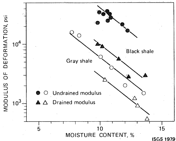
Figure 169. Comparison of deformation modulus and moisture content. Laboratory tests with samples of shales of the Caseyville Formation, Pennsylvanian System, in the Illinois Basin Coal Field, taken from foundation borings; approximate depths, 25 to 55 feet (7.6 to 16.7 m). Data from Hendron et al., 1970.
