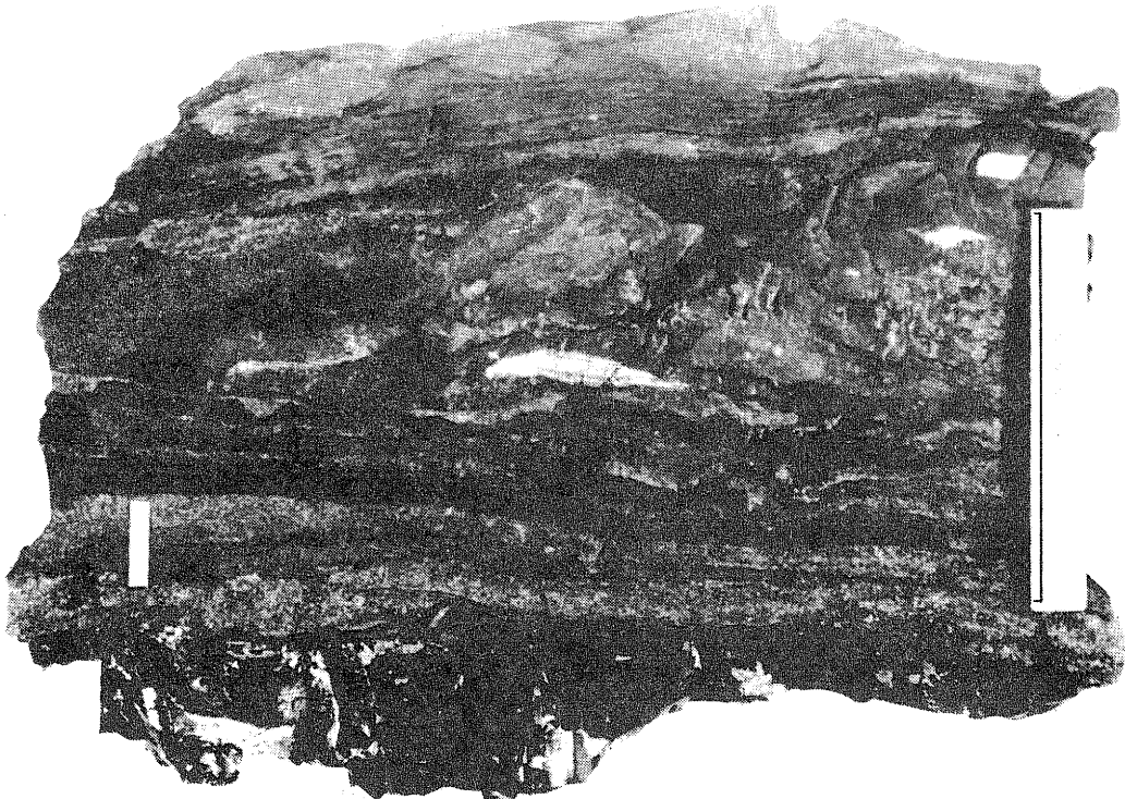
Figure 27. Syndimentary small slump and load structures of coarse-grained clastic sediments in otherwise fine- to medium-grained argillaceous limestone. In places, they not only cause excessive wear on mining tools but are prone to fall out of the roof. Scale (at right side): 15 cm. Location: mine H, "Quality Circle," southern Illinois.
