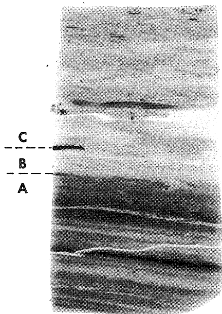
Figure 174. Radiograph of a black to dark-gray shale. (A) well-bedded fissile portion, (B) gradational contact, and (C) poorly bedded portion. Anna Shale from Clinton County (scale=1:1).
