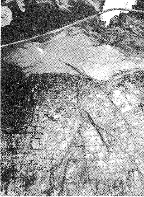
Figure 43. Gray shale roll sheared into several blocks. Shear plane pattern of high-angle synthetic and antithetic faults in Herrin (No. 6) Coal, which steepen downward, resembles clay-dike faults as found under black shale-limestone roof. Location: southern Illinois, "Quality Circle," mine C.
