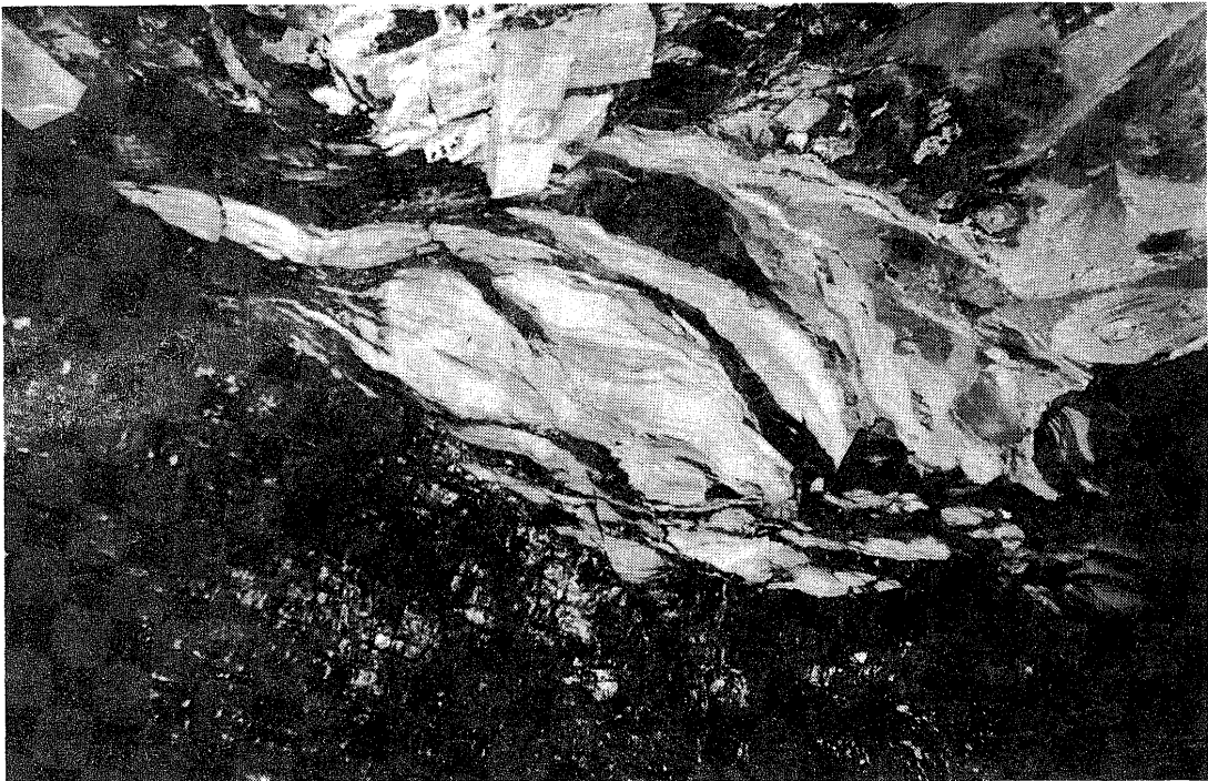
Figure 37. Large roll: Protrusion of clastic material of the Energy Shale, mainly siltstone and sandstone, from the roof into top of the Herrin (No. 6) Coal, probably penecontemporaneous to sedimentation in the Walshville channel. Rolls of this type are abundant in the "Quality Circle" area of mines C and O in southern Illinois and also have been recognized in east-central Illinois in mines D and G. Note the downward dipping of the bedding and the split of the coal strata, forming coal riders and the irregular pattern of shear planes and small normal faults, which result from differential compaction. The siltstone laminations and layers are unconformable in the main body of the roll.
