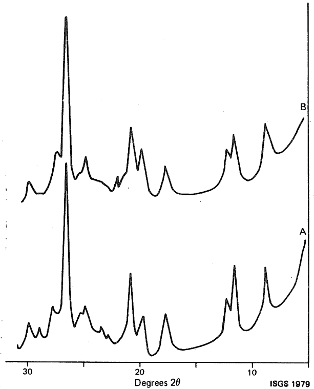
Figure 15. Diffractograms of a claystone in which sections of rock were cut parallel to bedding (A) and perpendicular to the bedding (B). The diffraction peaks in both sections are of about equal height, indicating randomly oriented clay crystals. (Sample: gray shale [mudstone] from Edgar County.)
