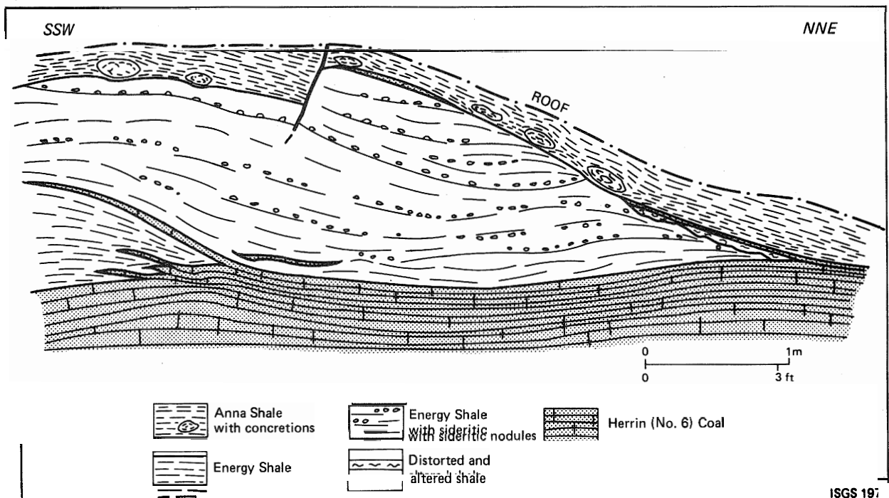
Figure 23. Small lens of Energy Shale from transitional area of gray shale to black shale-limestone roof types. The configuration resembles slump structures and rolls described later in this chapter. Note also the coal stringers in and above the lens. Bedding of Energy Shale and Anna Shale appears to be unconformable. Small normal fault, probably resulting from differential compaction, is lubricated with coal. Location: edge of "Quality Circle," southern Illinois, mine H.
