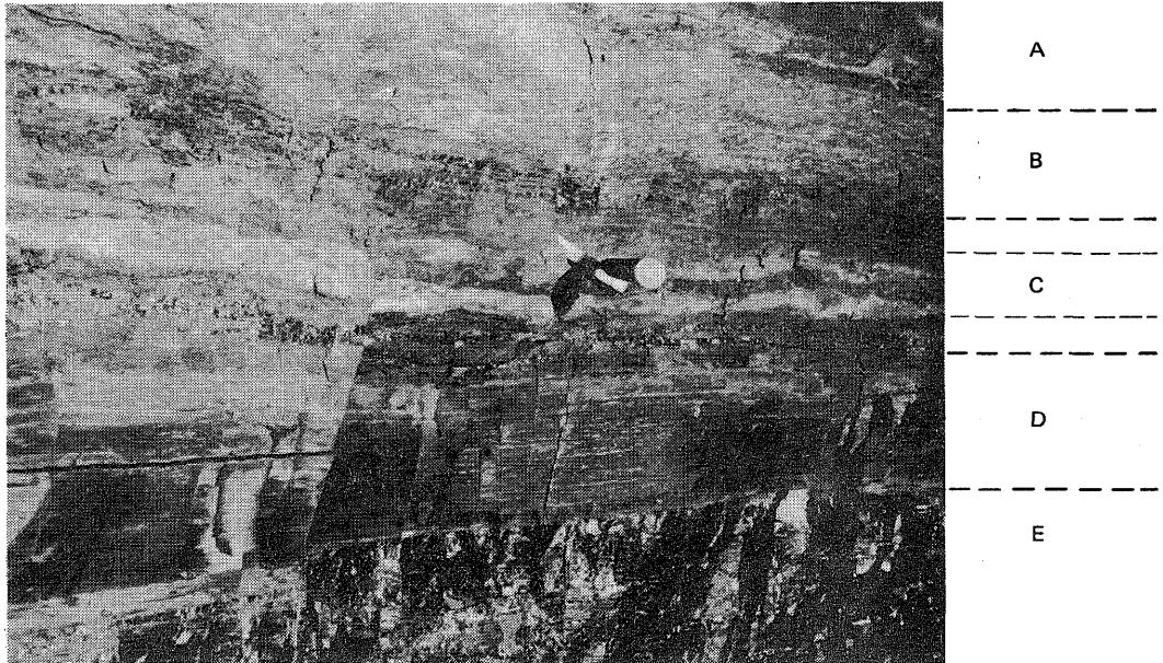
Figure 75. Jamestown Coal immediately above the Anna Shale. Stratigraphic section: (A) Lawson Shale, (B) Conant Limestone (here consisting of flaky calcareous shale), (C) "Jamestown Coal interval" (two layers of coal streaks separated by carbonaceous shales and nodular lenticular freshwater limestones), no Brereton Limestone, (D) Anna Shale (mainly lower fissile part), and (E) Herrin (No. 6) Coal. Black shale-limestone roof conditions of this type are prone to fail, commonly all the way up to the Bankston Fork Limestone, since no limestone is present in the succession or if present is not strong enough to bridge stresses from pillar to pillar. Location: mine A, west-central Illinois.
