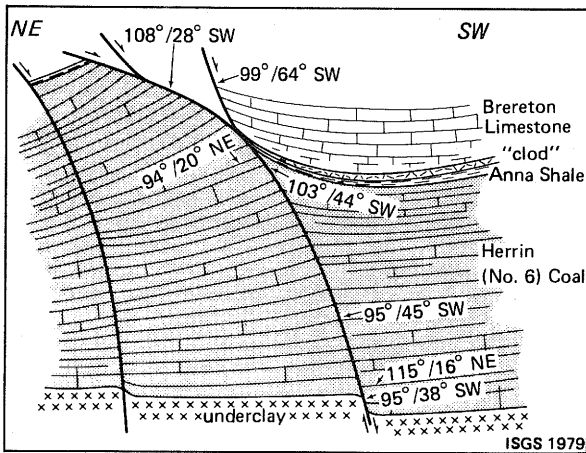
Figure 93. Clay-dike faults cutting through entire coal seam and displacing Breerton Limestone, Anna Shale, Herrin (No. 6) Coal, and underclay. Note normal drag and thinning of Anna Shale and Breerton Limestone strata and false drag in some places of coal. Location: mine A, west-central Illinois.
