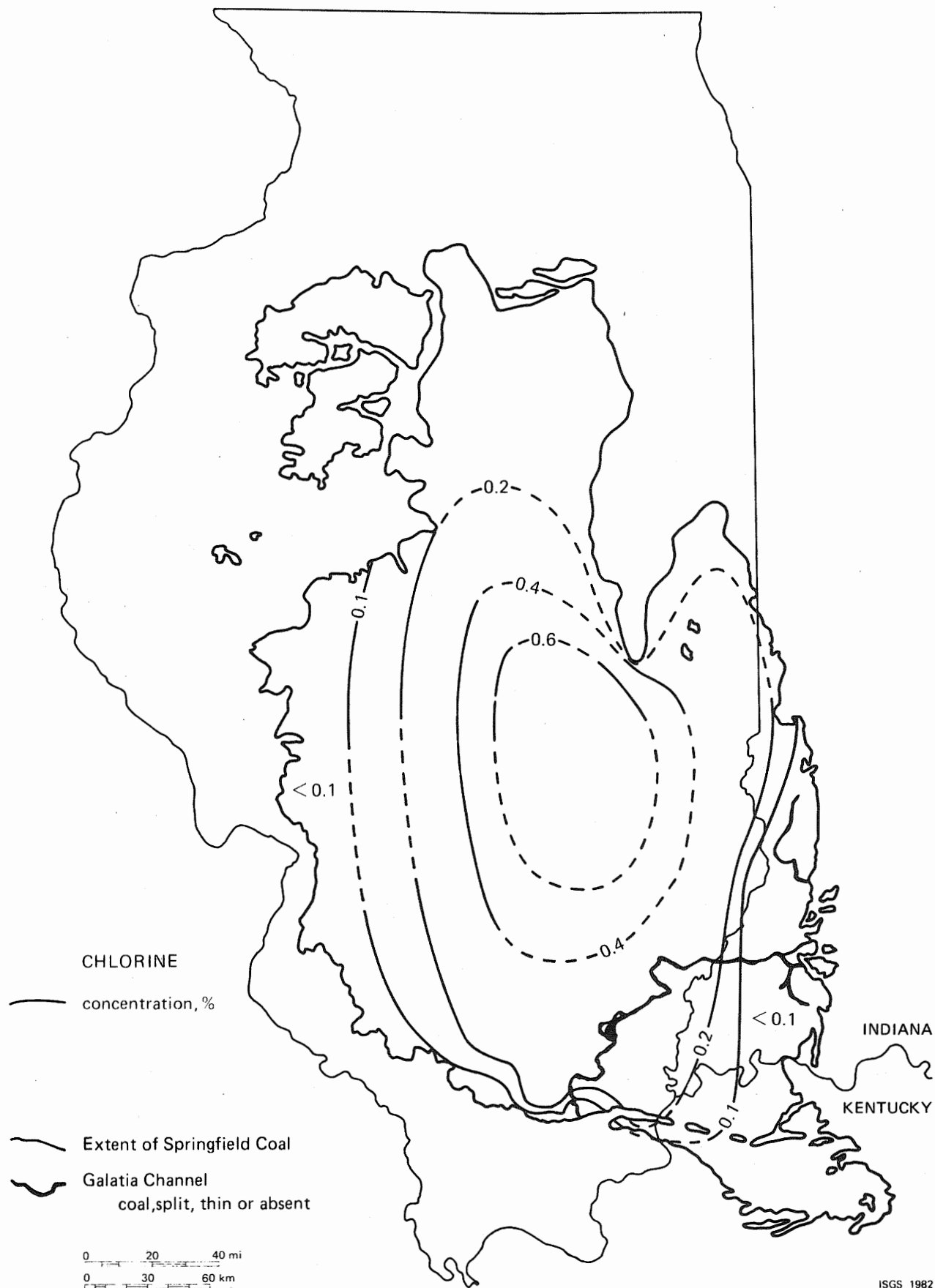
FIGURE VI-20. Areal distribution of chlorine in the Springfield Coal.
