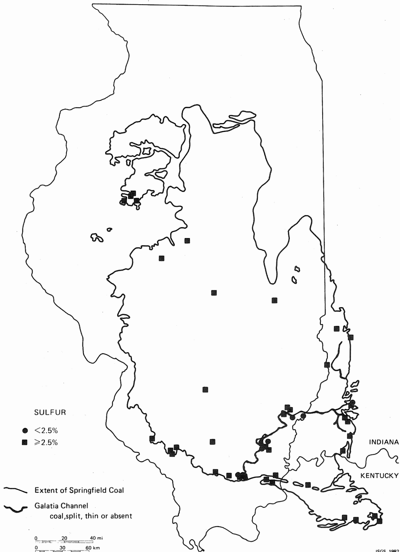
FIGURE VI-25. Areal distribution of sulfur in the Springfield Coal.
