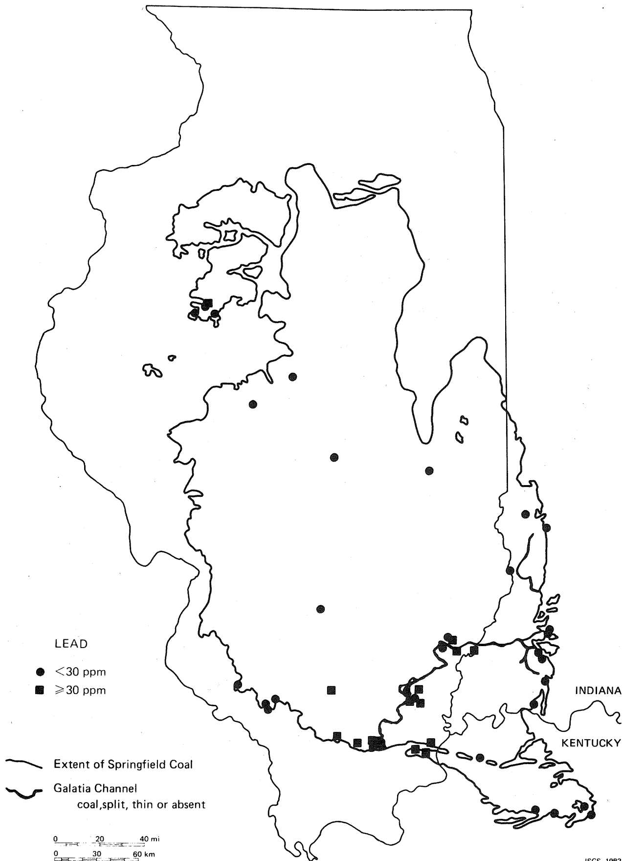
FIGURE VI-28. Areal distribution of lead in the Springfield Coal.
