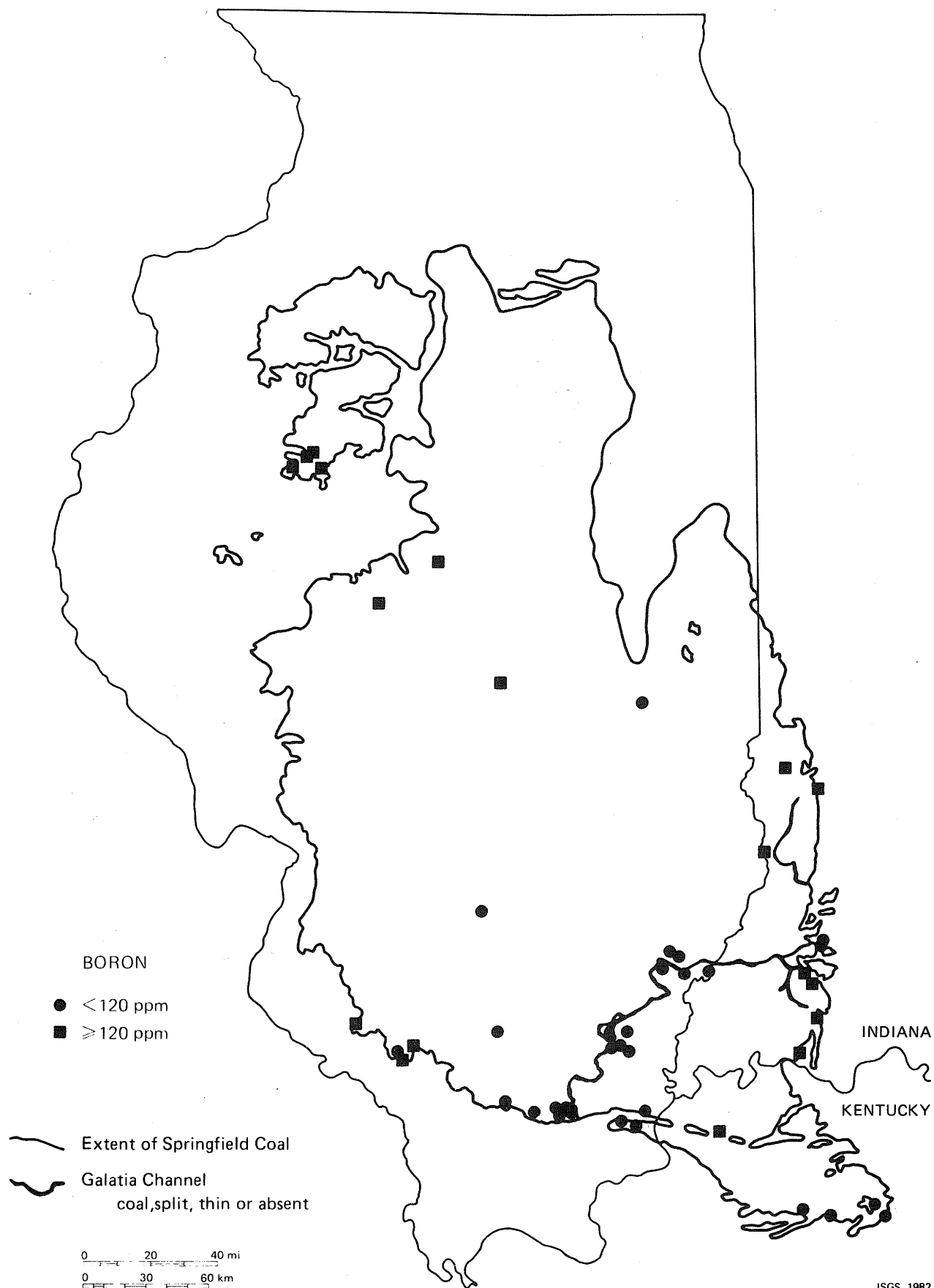
FIGURE VI-24. Areal distribution of boron in the Springfield Coal.
