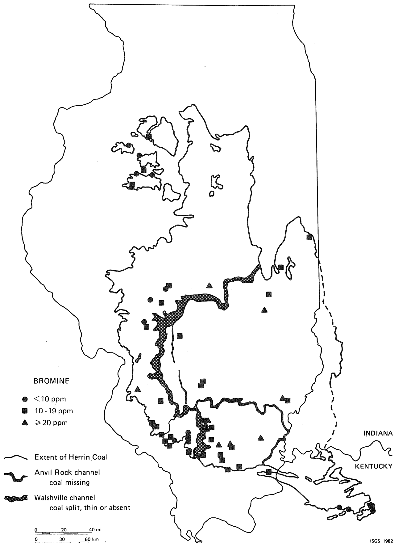
FIGURE VI-10. Areal distribution of bromine in the Herrin Coal.
