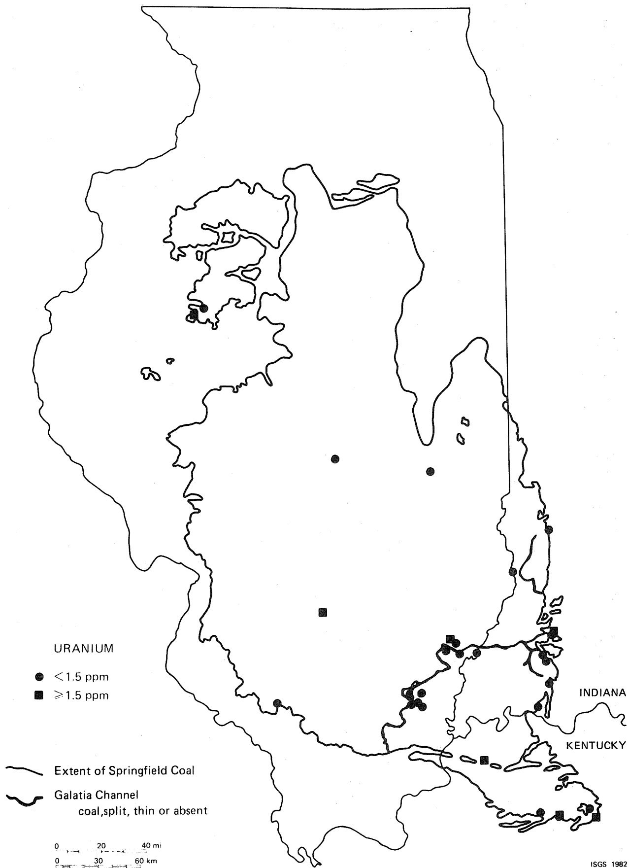
FIGURE VI-30. Areal distribution of uranium in the Springfield Coal.
