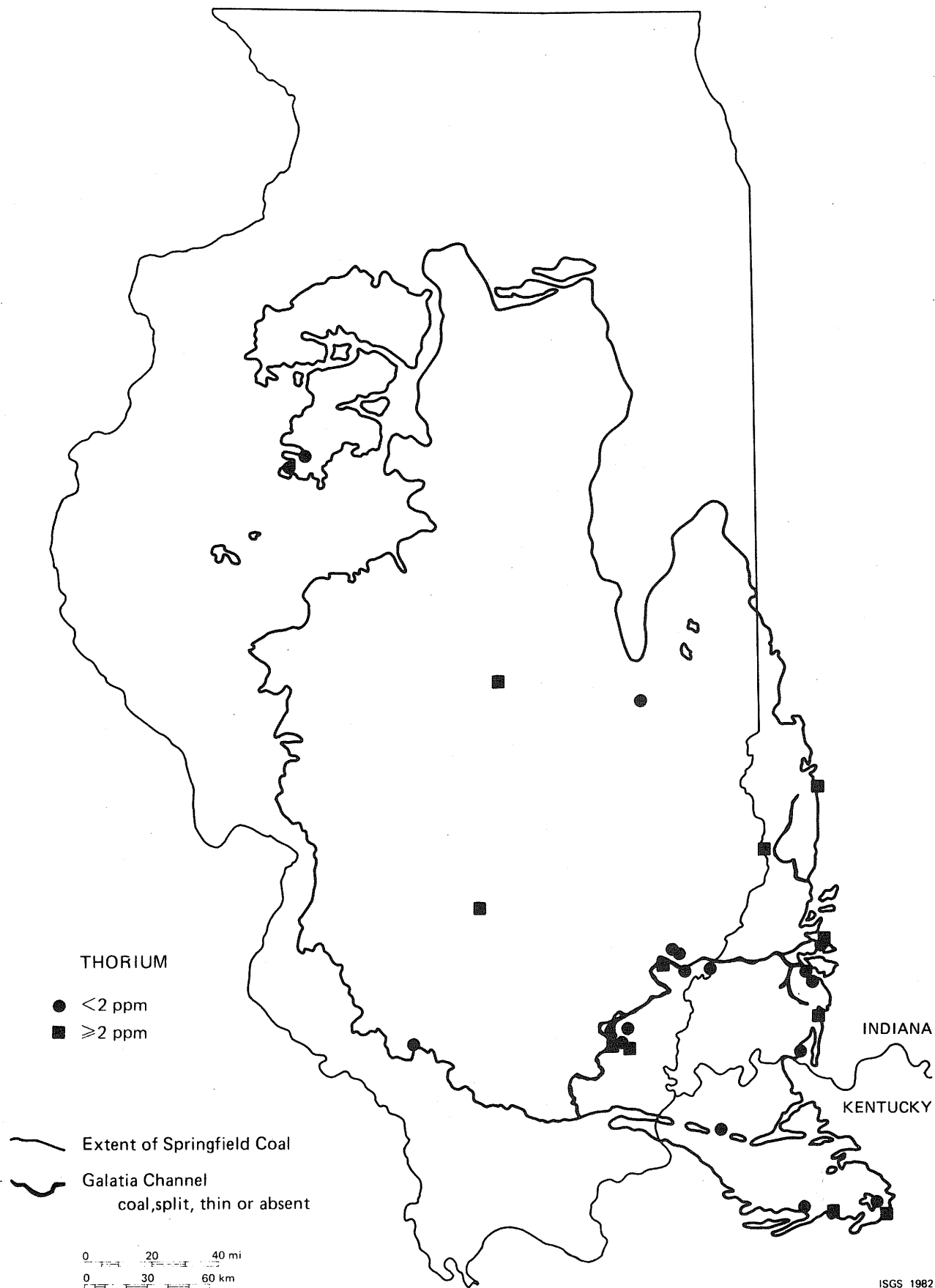
FIGURE VI-29. Areal distribution of thorium in the Springfield Coal.
