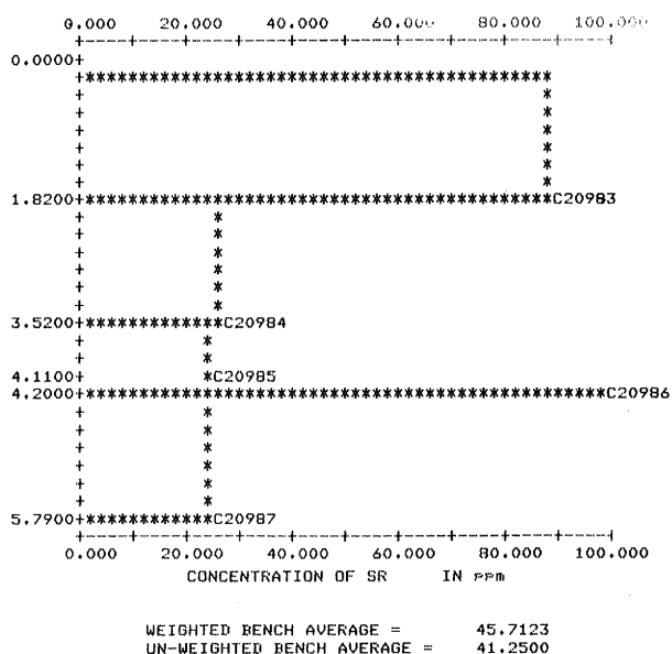
FIGURE VI-5. Bench set profiles for calcite, Ca, Mn, and Sr in bench set B9.
