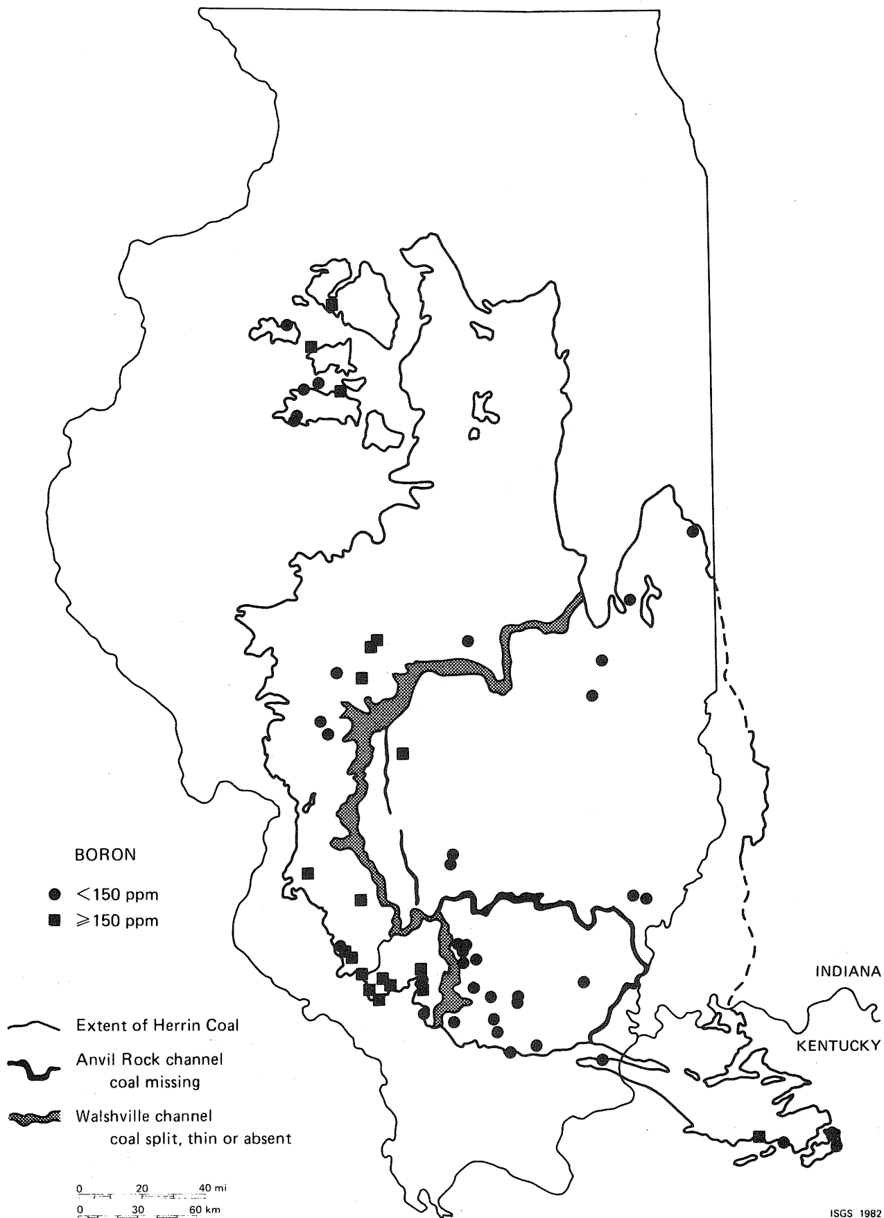
FIGURE VI-12. Areal distribution of boron in the Herrin Coal.
