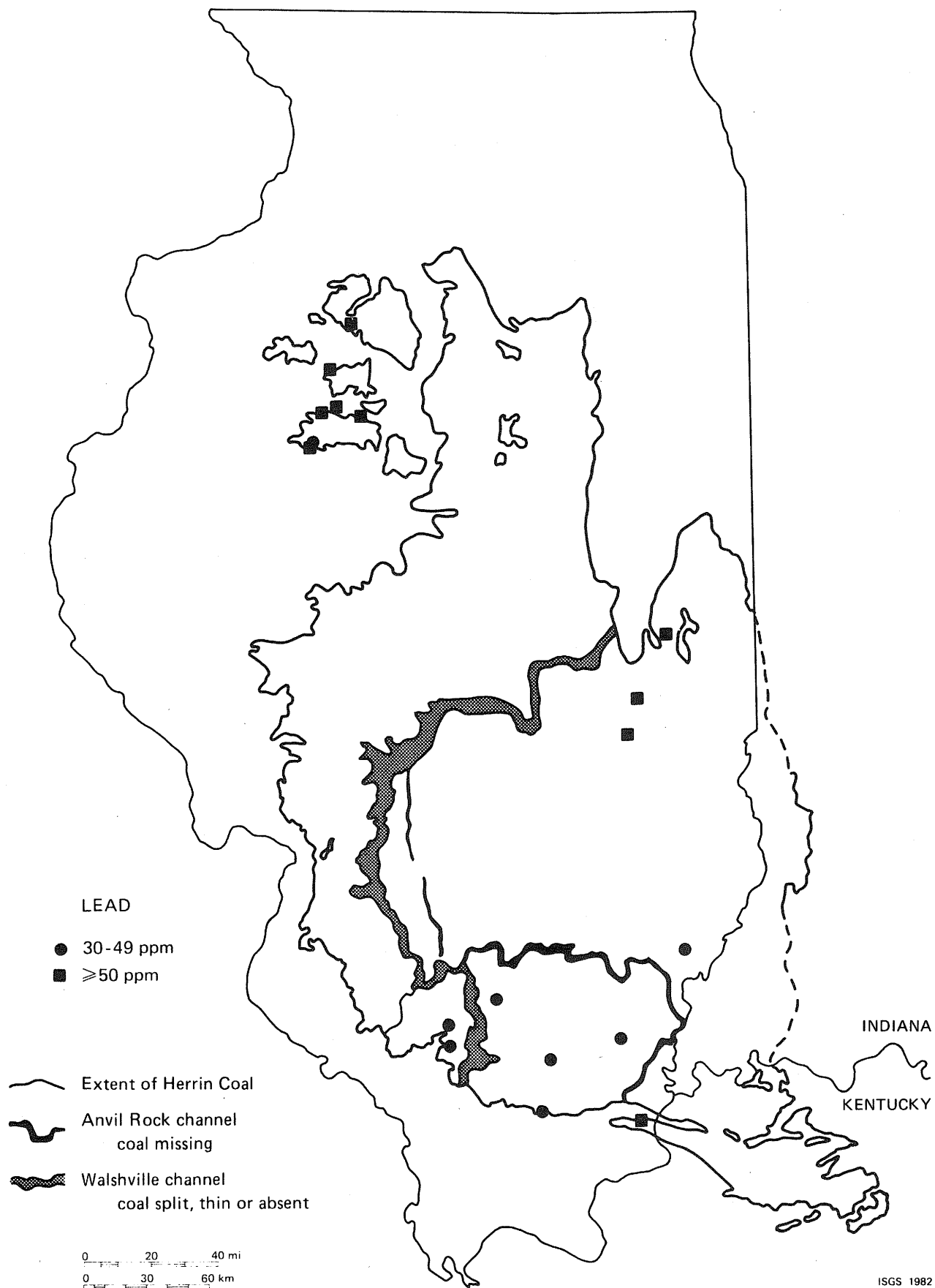
FIGURE VI-16. Areal distribution of lead in the Herrin Coal.
