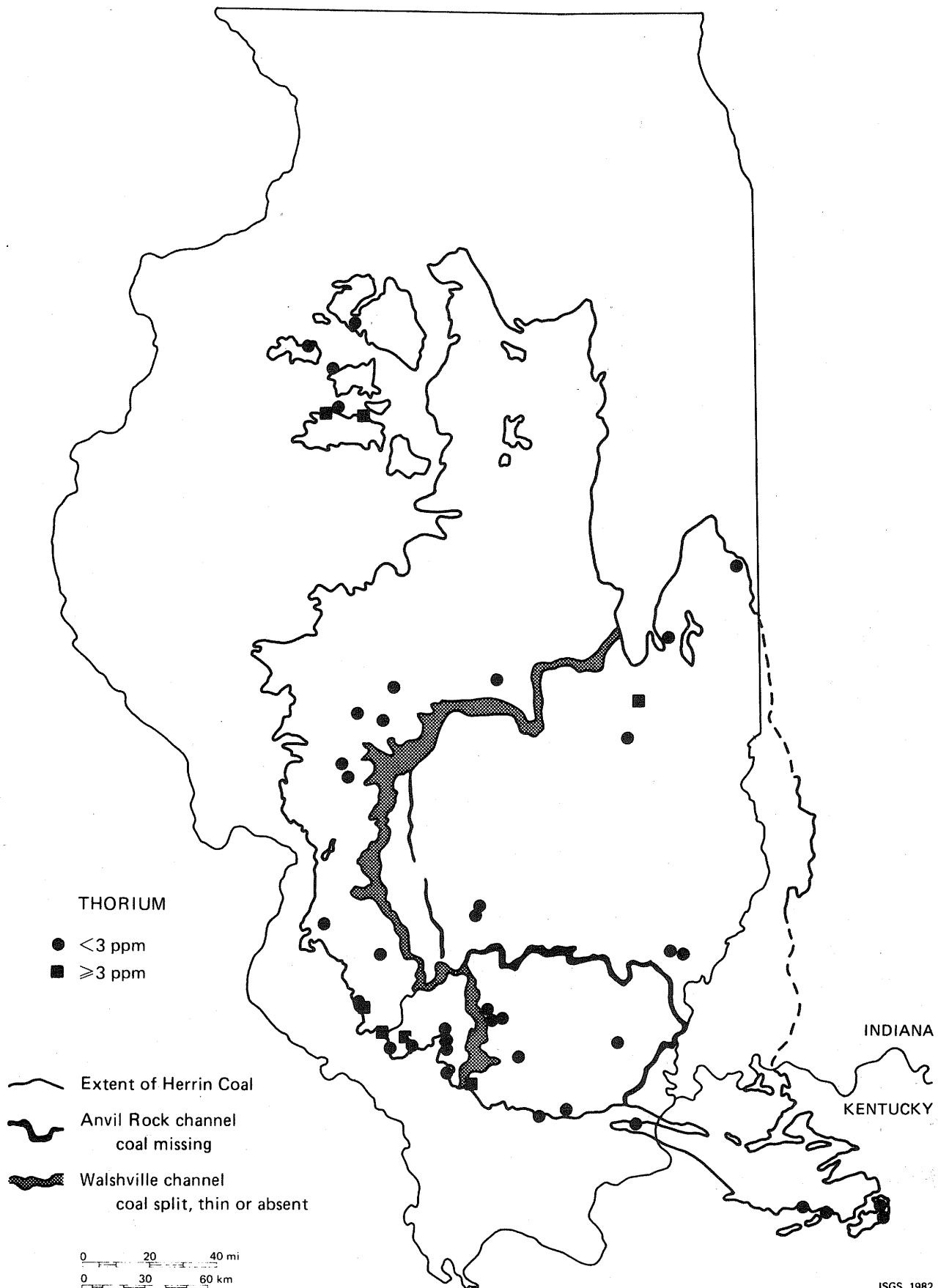
FIGURE VI-17. Areal distribution of thorium in the Herrin Coal.
