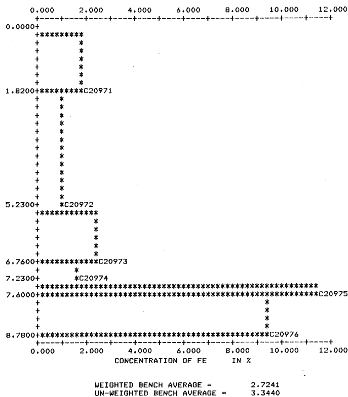
FIGURE VI-3. Bench set profiles for pyrite, Fe, As, and Pb from bench set B7.
