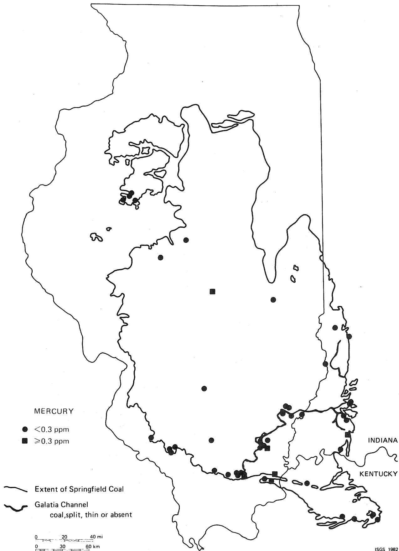
FIGURE VI-27. Areal distribution of mercury in the Springfield Coal.
