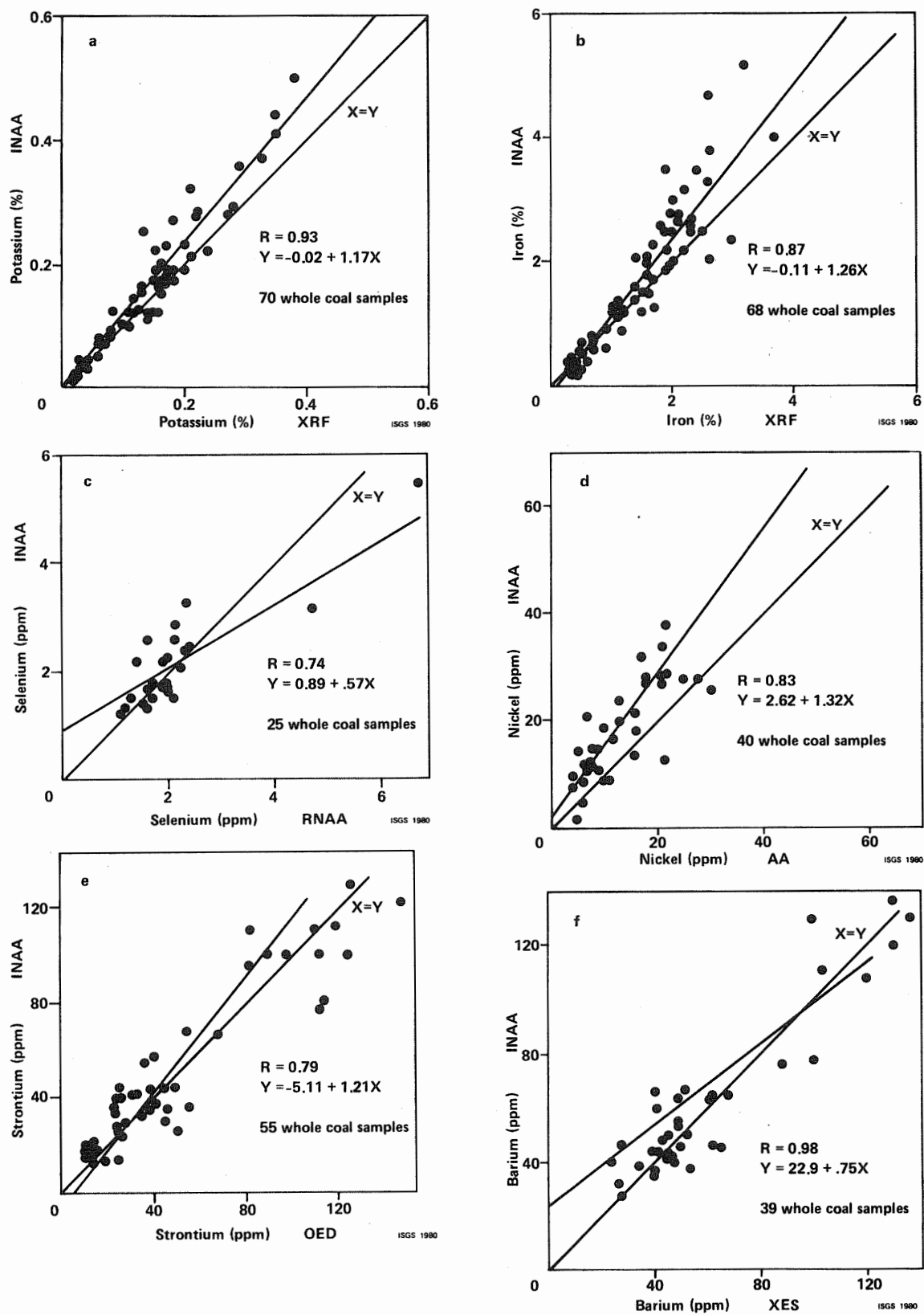
FIGURE III-3. Determinations of six elements in whole coals by two methods.
