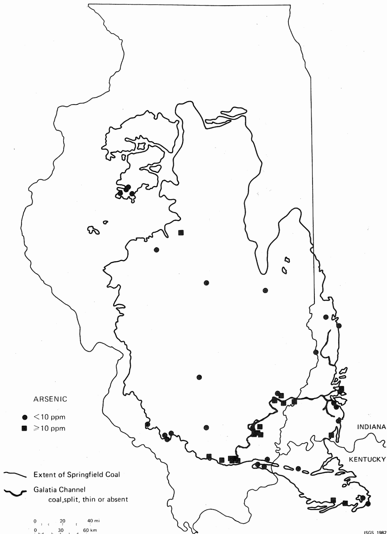
FIGURE VI-26. Areal distribution of arsenic in the Springfield Coal.
