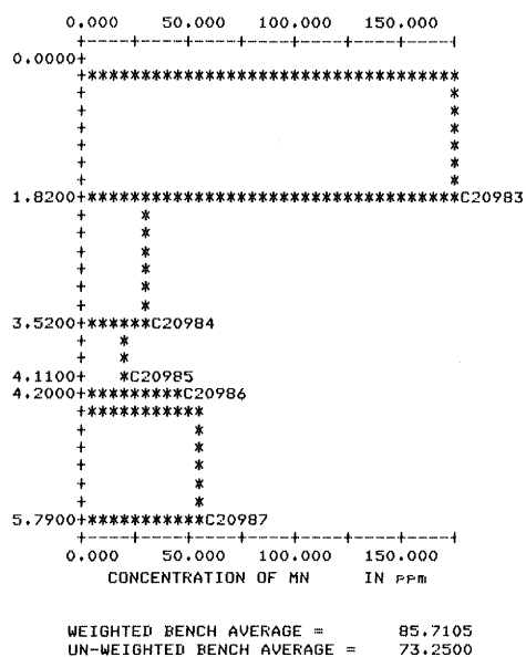
FIGURE VI-5. Bench set profiles for calcite, Ca, Mn, and Sr in bench set B9.
