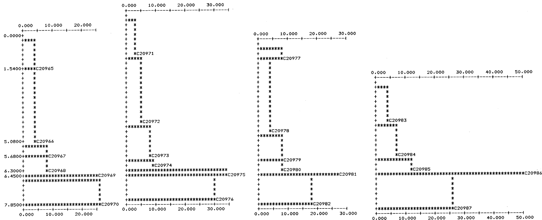
FIGURE VI-6. Bench set profiles for nickel (all bench sets).
