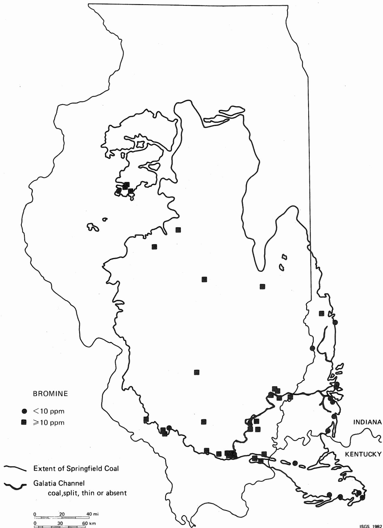
FIGURE VI-22. Areal distribution of bromine in the Springfield Coal.
