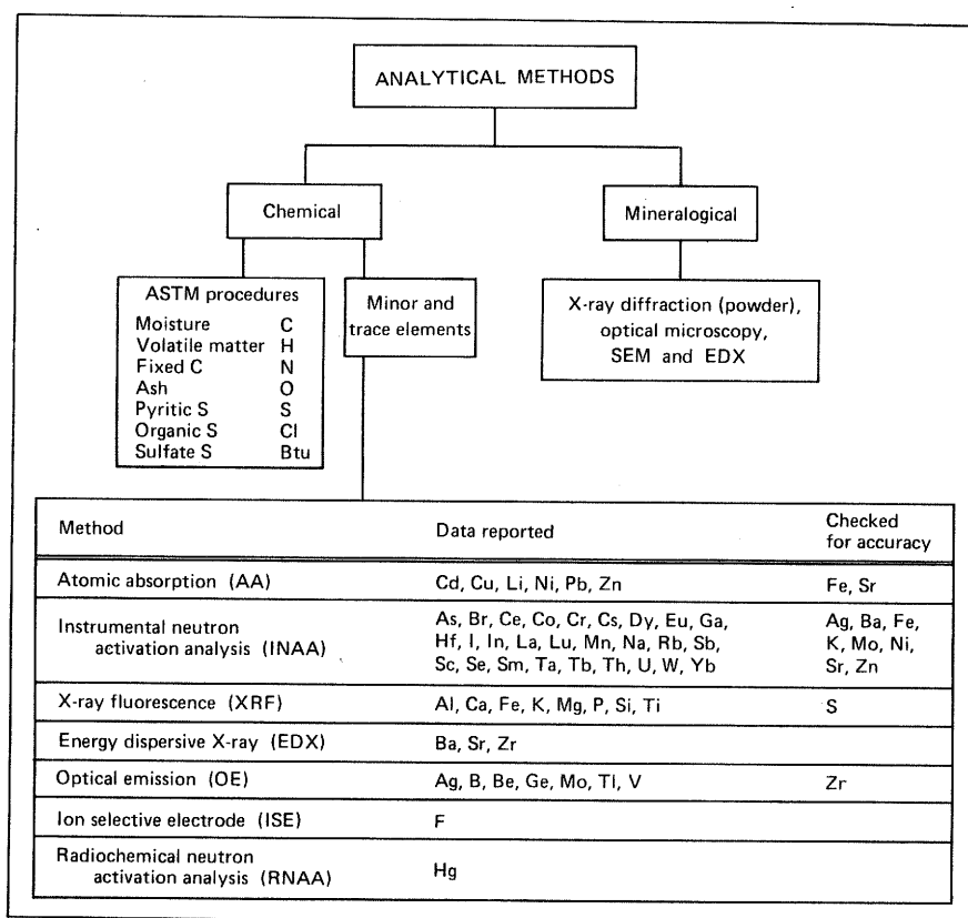
FIGURE III-2. Methods used for analyses of coal samples.
