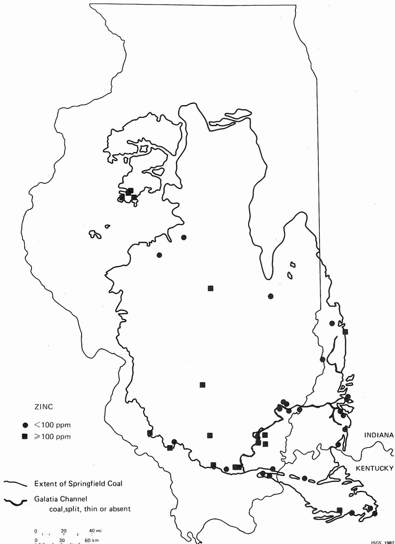
FIGURE VI-23. Areal distribution of zinc in the Springfield Coal.
