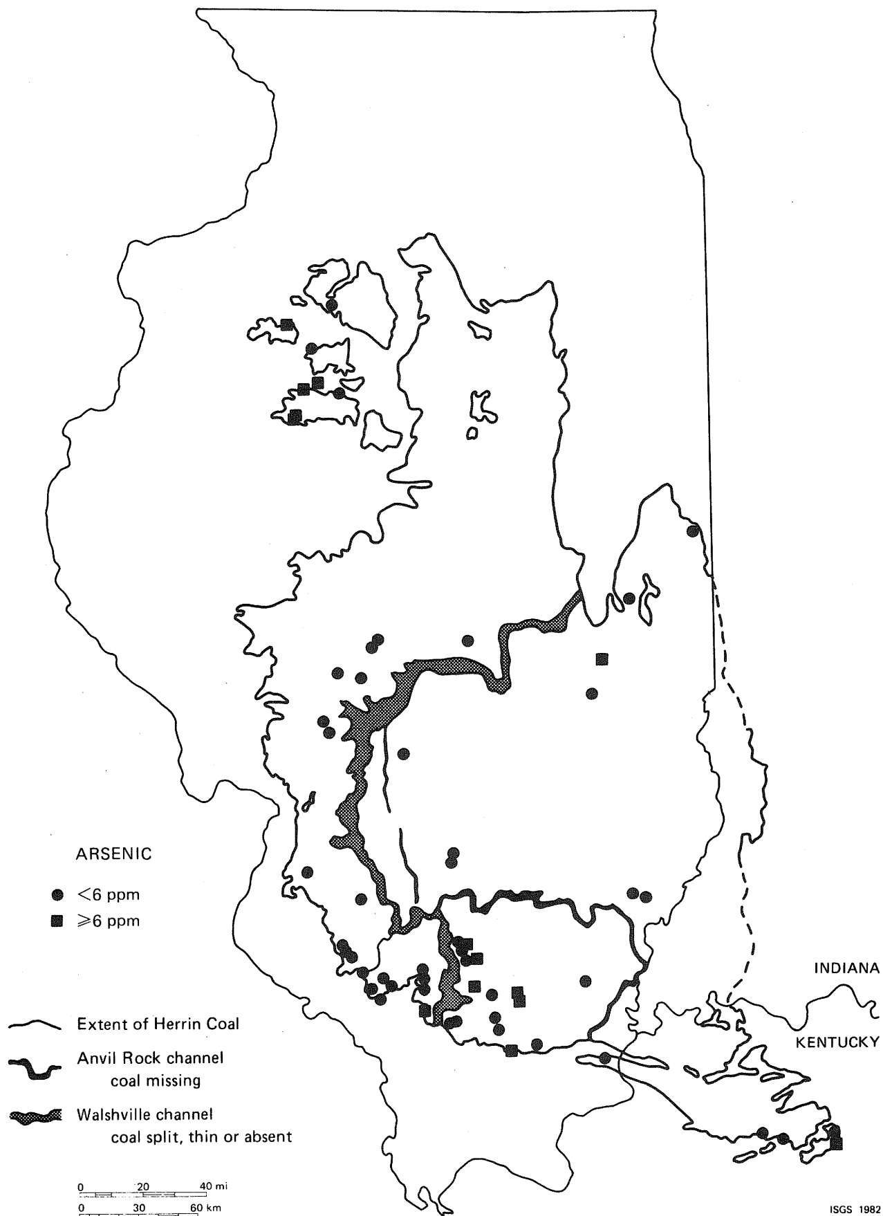
FIGURE VI-14. Areal distribution of arsenic in the Herrin Coal.
