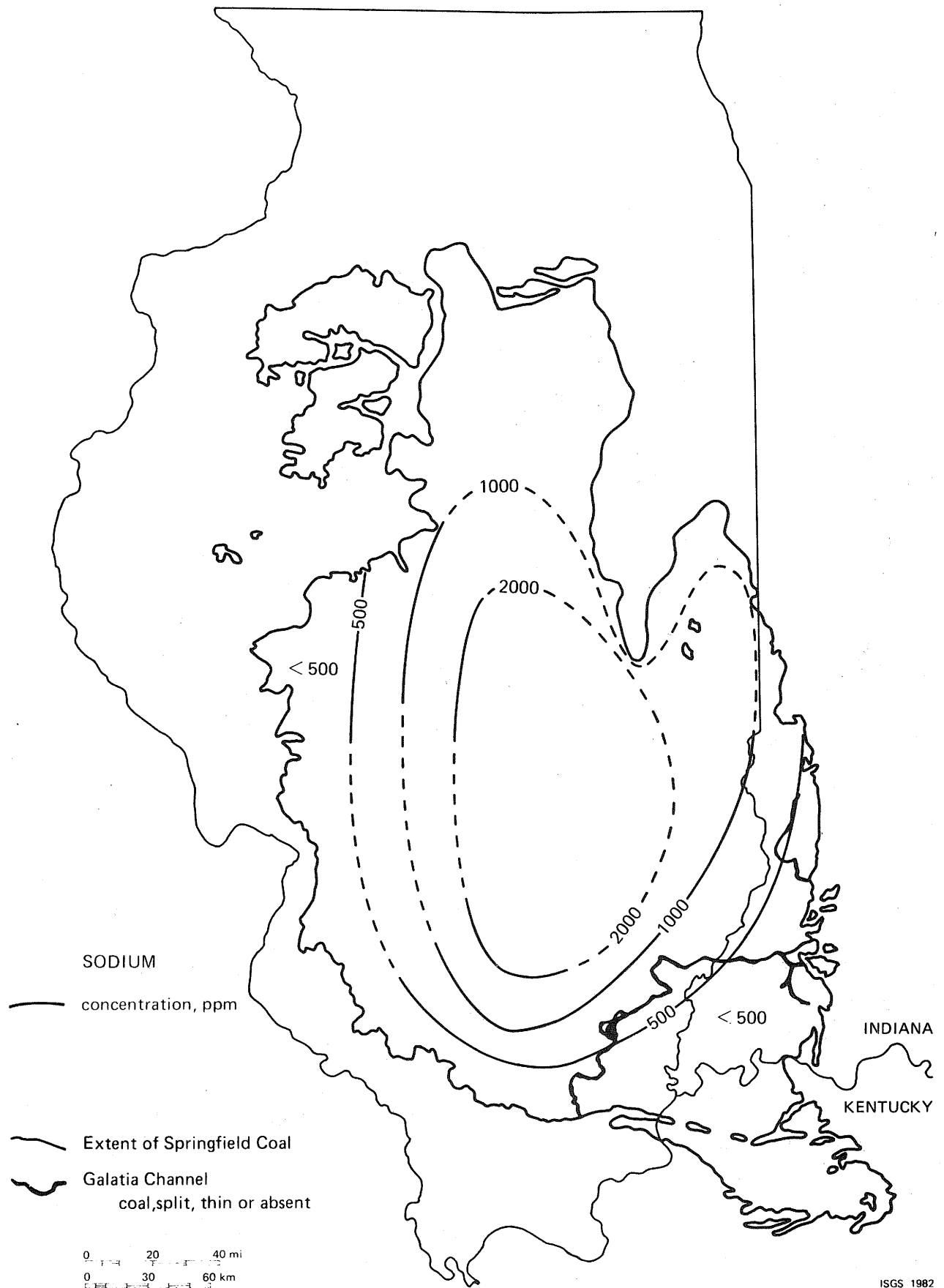
FIGURE VI-21. Areal distribution of sodium in the Springfield Coal.
