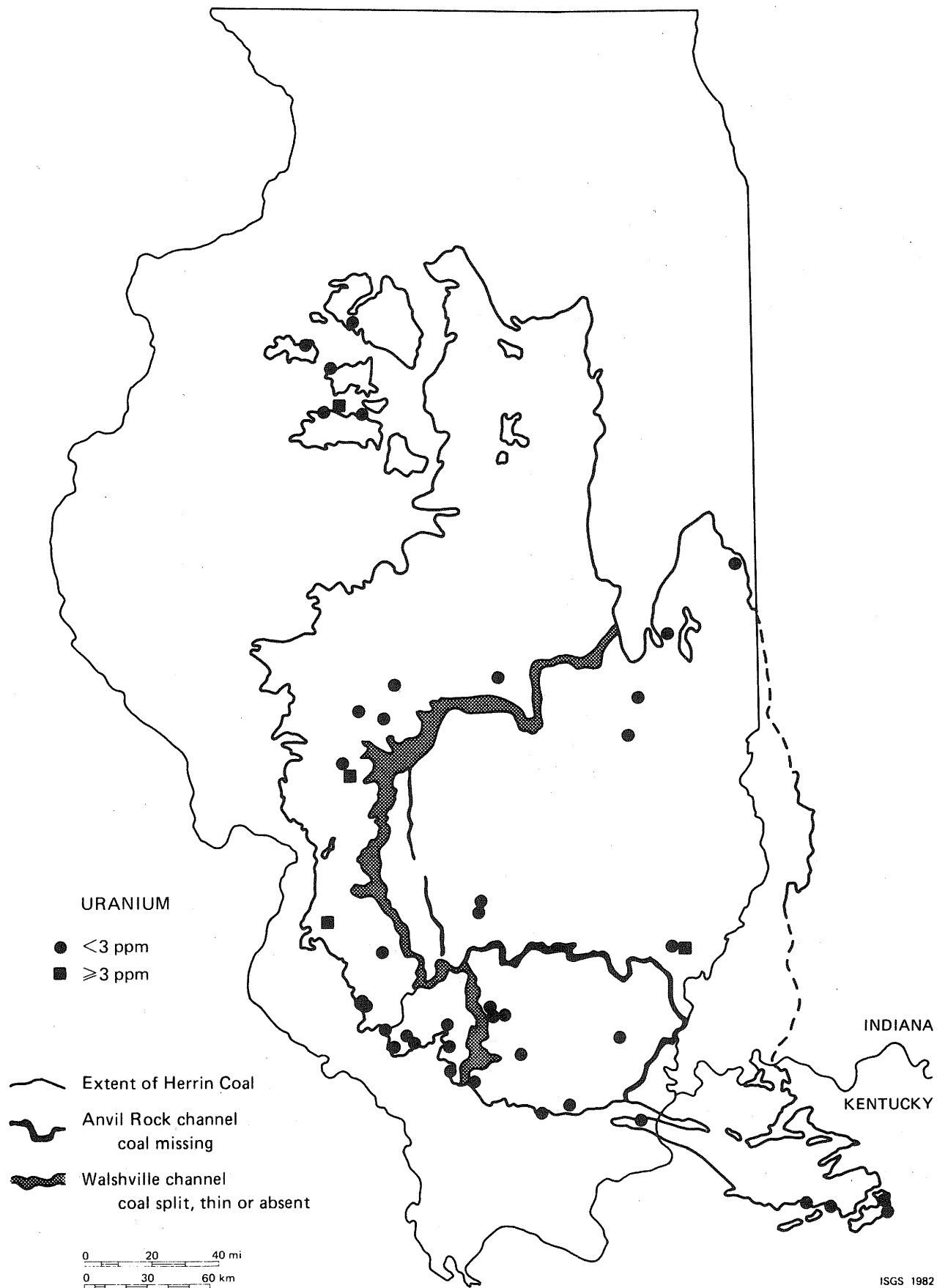
FIGURE VI-18. Areal distribution of uranium in the Herrin Coal.
