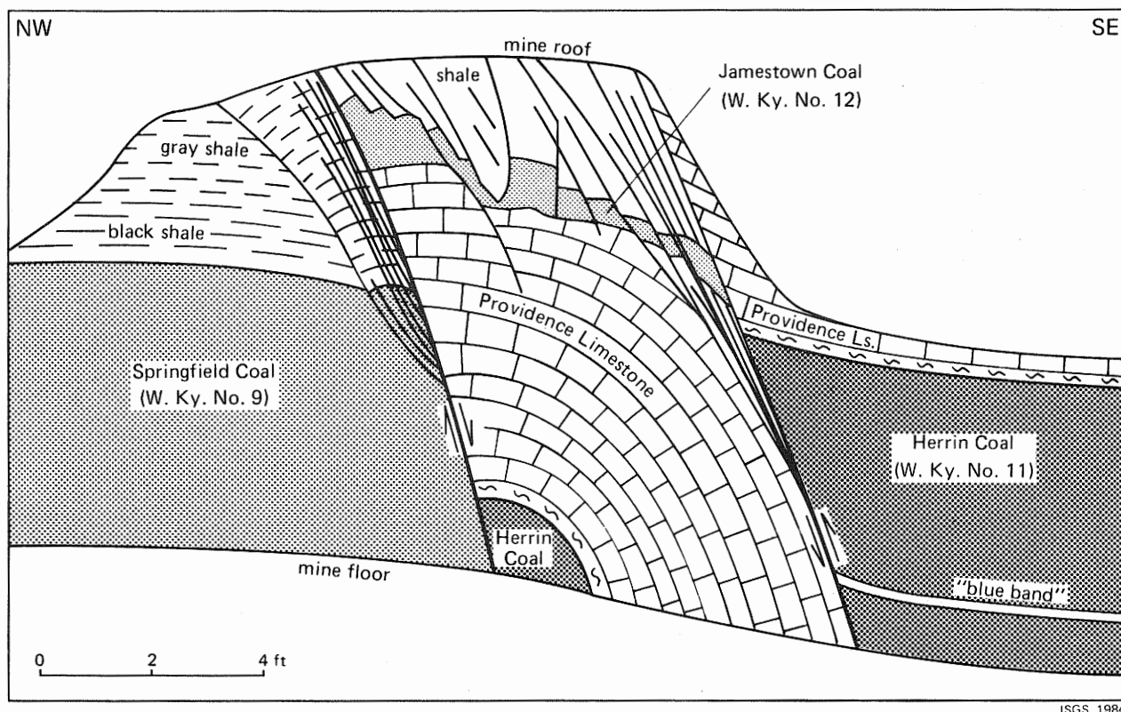
FIGURE 16. View of same fault as in figure 15, on an adjacent heading in the mine; here the structural situation is more complicated. Although the overall displacement is normal, the central slice of the fault zone is dropped below its level on either side of the zone, indicating reverse movement on the right-hand fault. Note the small reverse flexure in the Springfield Coal and overlying shales, left of center.
