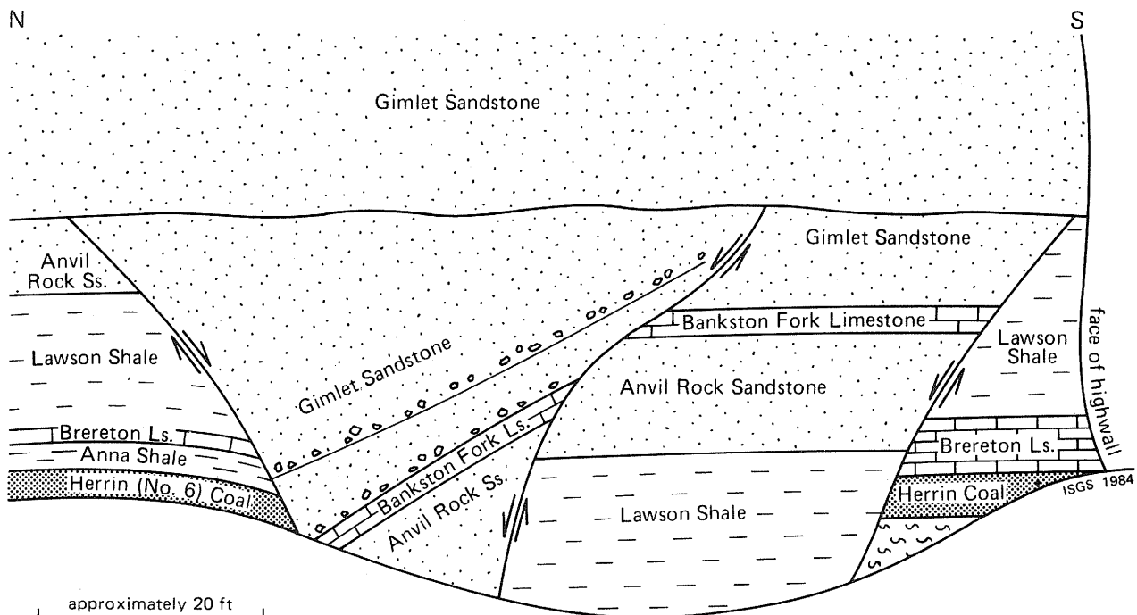
FIGURE 27. Paleosump in highwall of Peabody Coal Company's Eagle Surface Mine.
