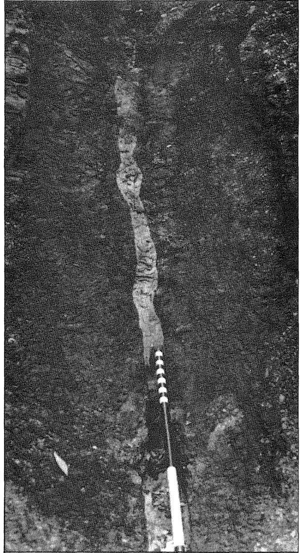
FIGURE 39. Left: Nearly vertical fault on strip mine highwall at north end of Colbert Hill, Rudement Quadrangle. East (left) side is downthrown 2 or 3 feet, but there are also indications of strike-slip movement on this peculiar fault. At top of highwall, weathered shale grades into residual soil; no Pleistocene sediments are present to indicate whether or not this fault was active in Quaternary time. Right: Closeup view of fault, showing sinuous zone of light gray soft clay gouge. Width and sinuosity of gouge zone on a fault of so little vertical displacement suggests a strike-slip component of movement.
