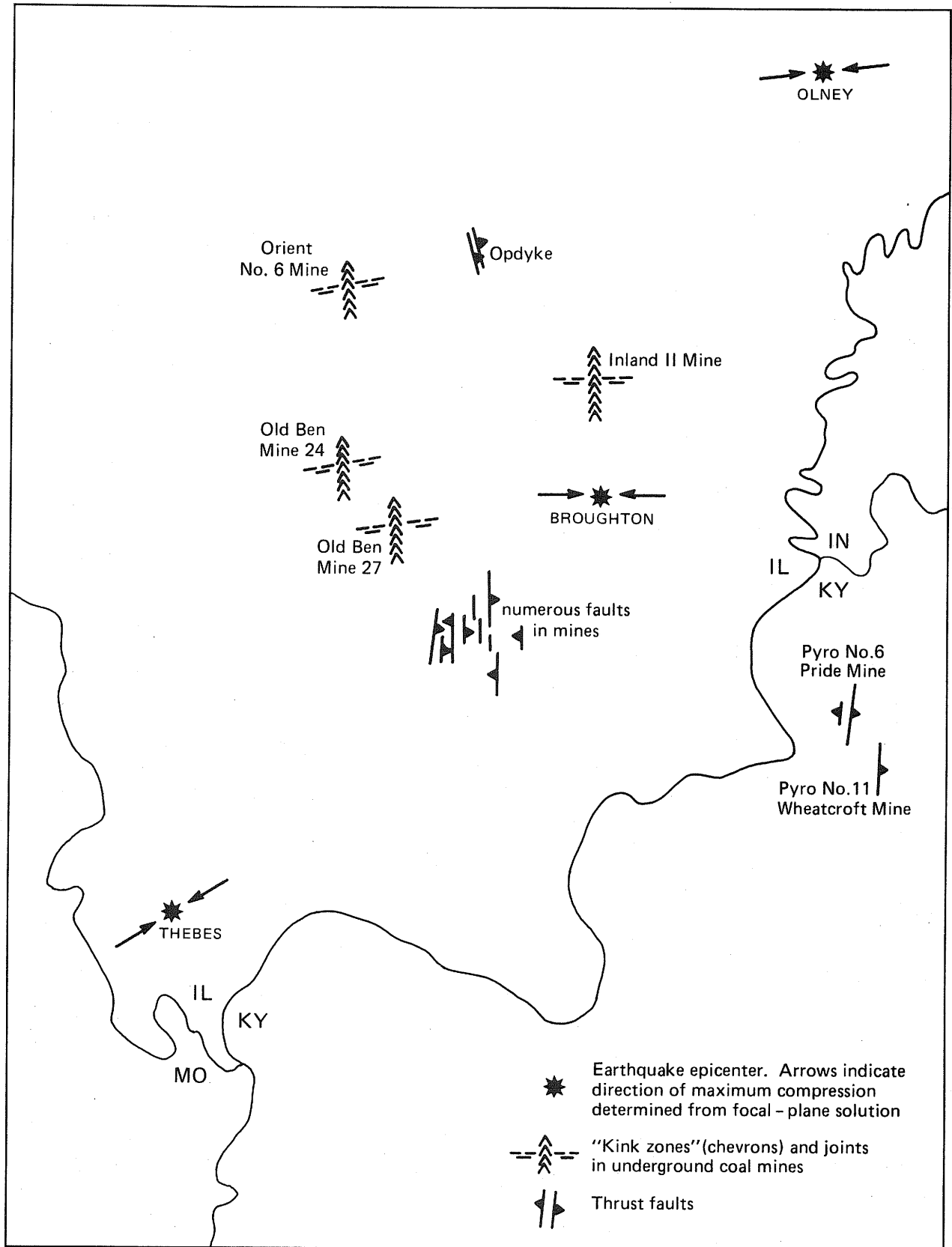
FIGURE 44. Features and measurements indicative of modern stress field.
