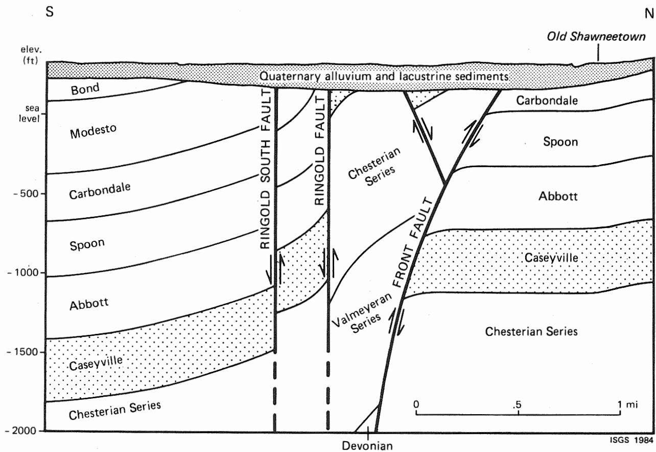
FIGURE 12. Cross section of Shawneetown Fault Zone just west of Ohio River (see section C-C', plate 1b).
