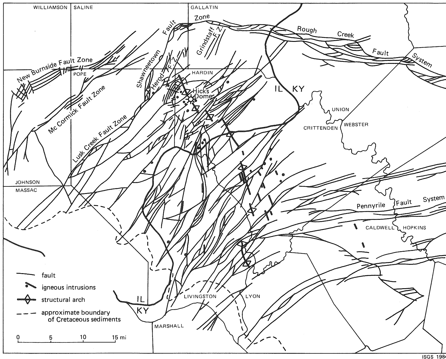
FIGURE 34. Fluorspar Area Fault Complex and associated structures (adapted from Trace, 1974; Schwalb and Potter, 1978; Treworgy, 1981; and Jacobson and Trask, 1983).
