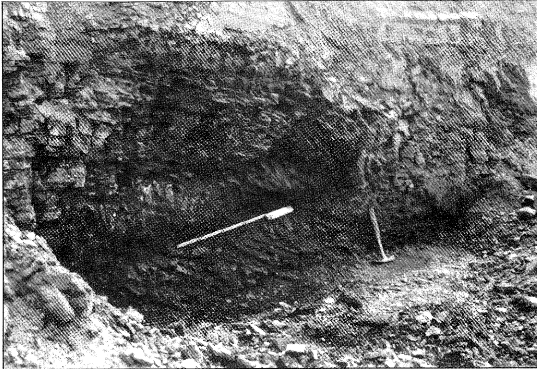
FIGURE 48. Thrust fault in Opdyke Coal at now-abandoned strip mine in southeastern Jefferson County, Illinois. This fault and a parallel asymmetrical anticline strike N 20 W and indicate compressional stress from the ENE and WSW.
