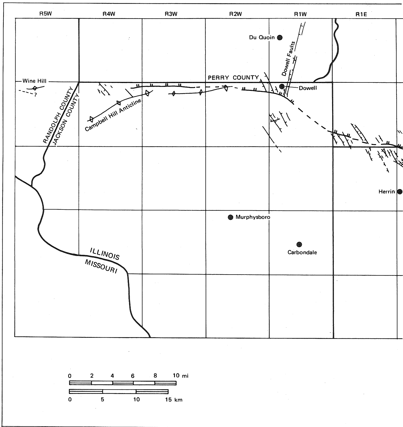
FIGURE 30. The Cottage Grove Fault System (from Nelson, 1981).
