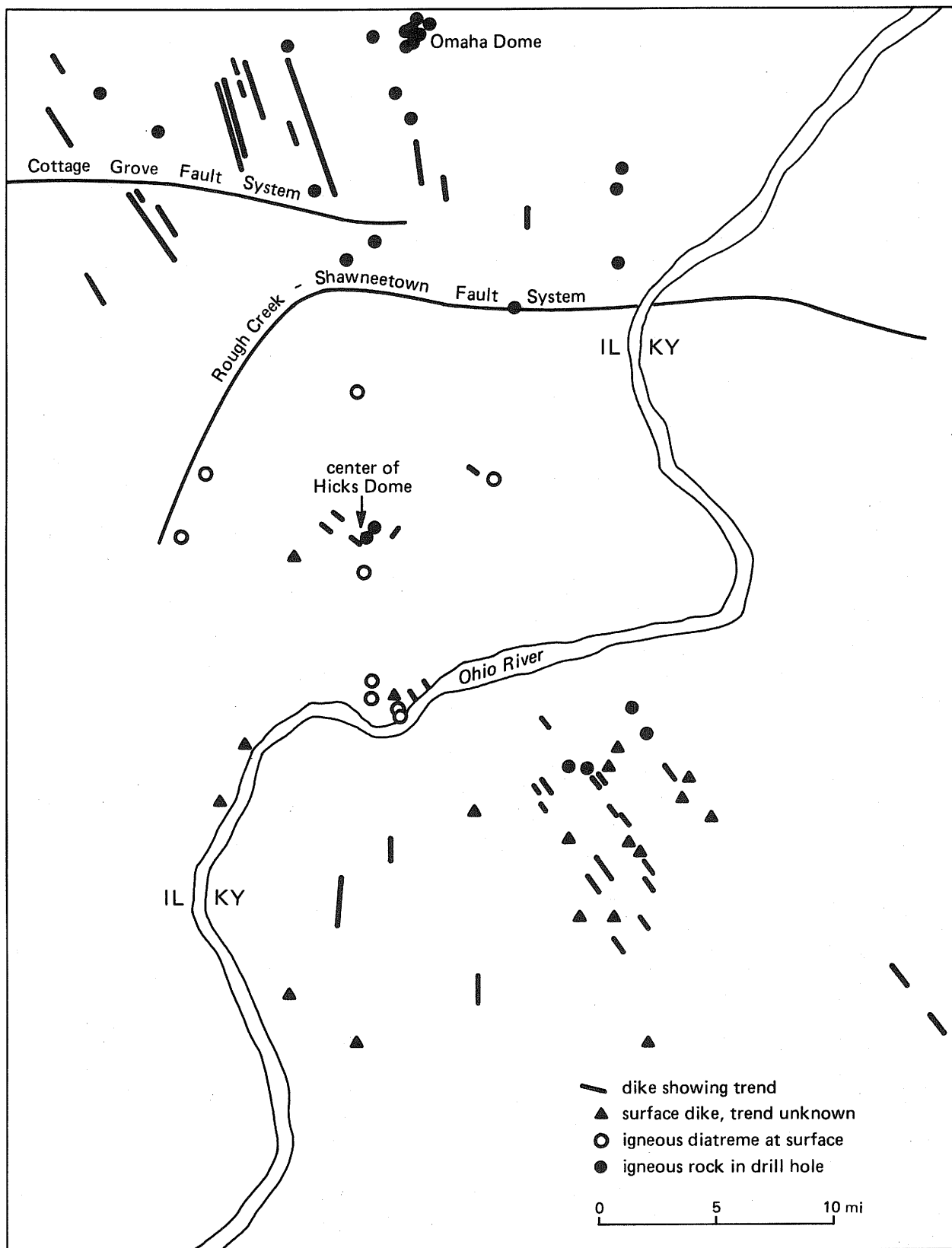
FIGURE 35. Igneous intrusions and diatremes in Illinois-Kentucky fluorspar district (modified from von Fresc, Hinze, and Braile, 1980).
