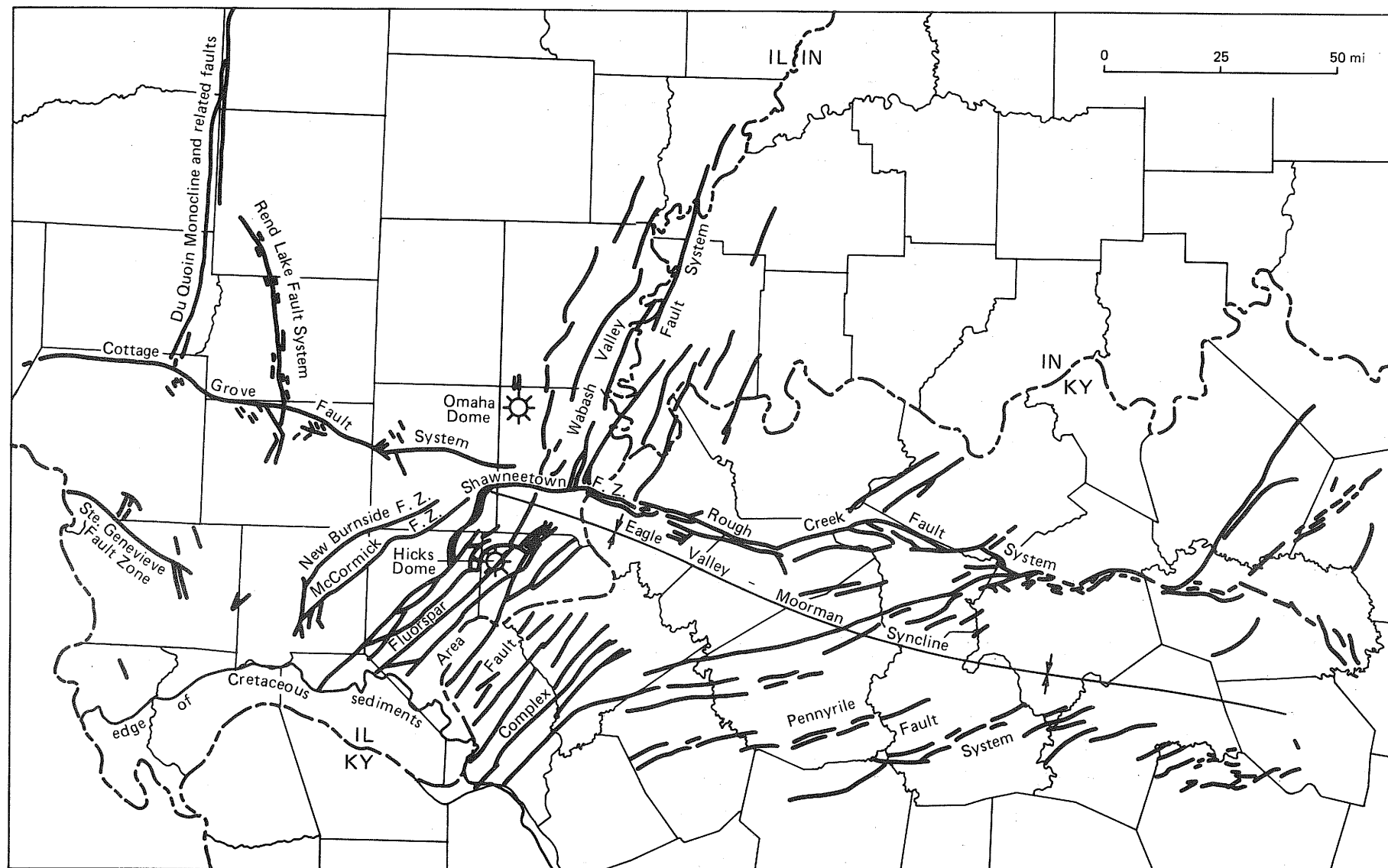
FIGURE 9. Structural features of southern Illinois, southwestern Indiana, and western Kentucky.
