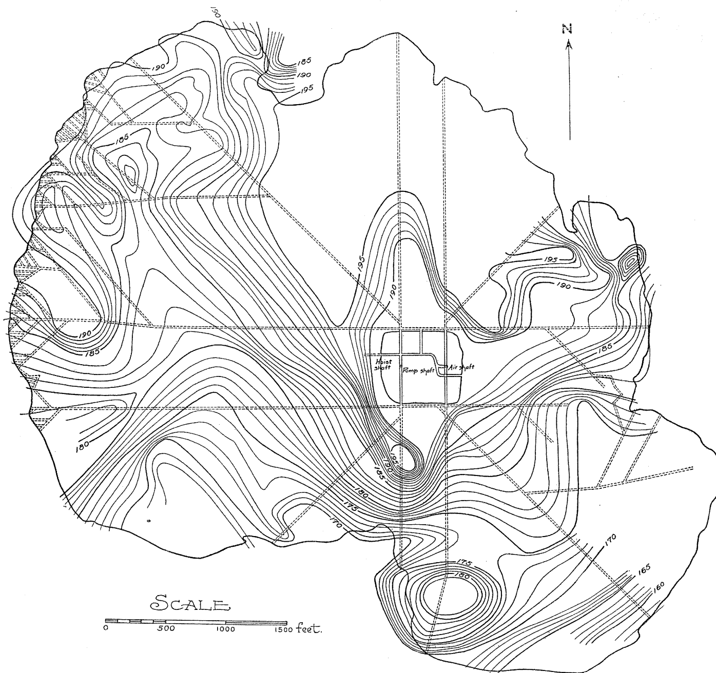
Contours on coal No. 2 in Ladd Mine (furnished by F. O. Chadwick, Engineer)
