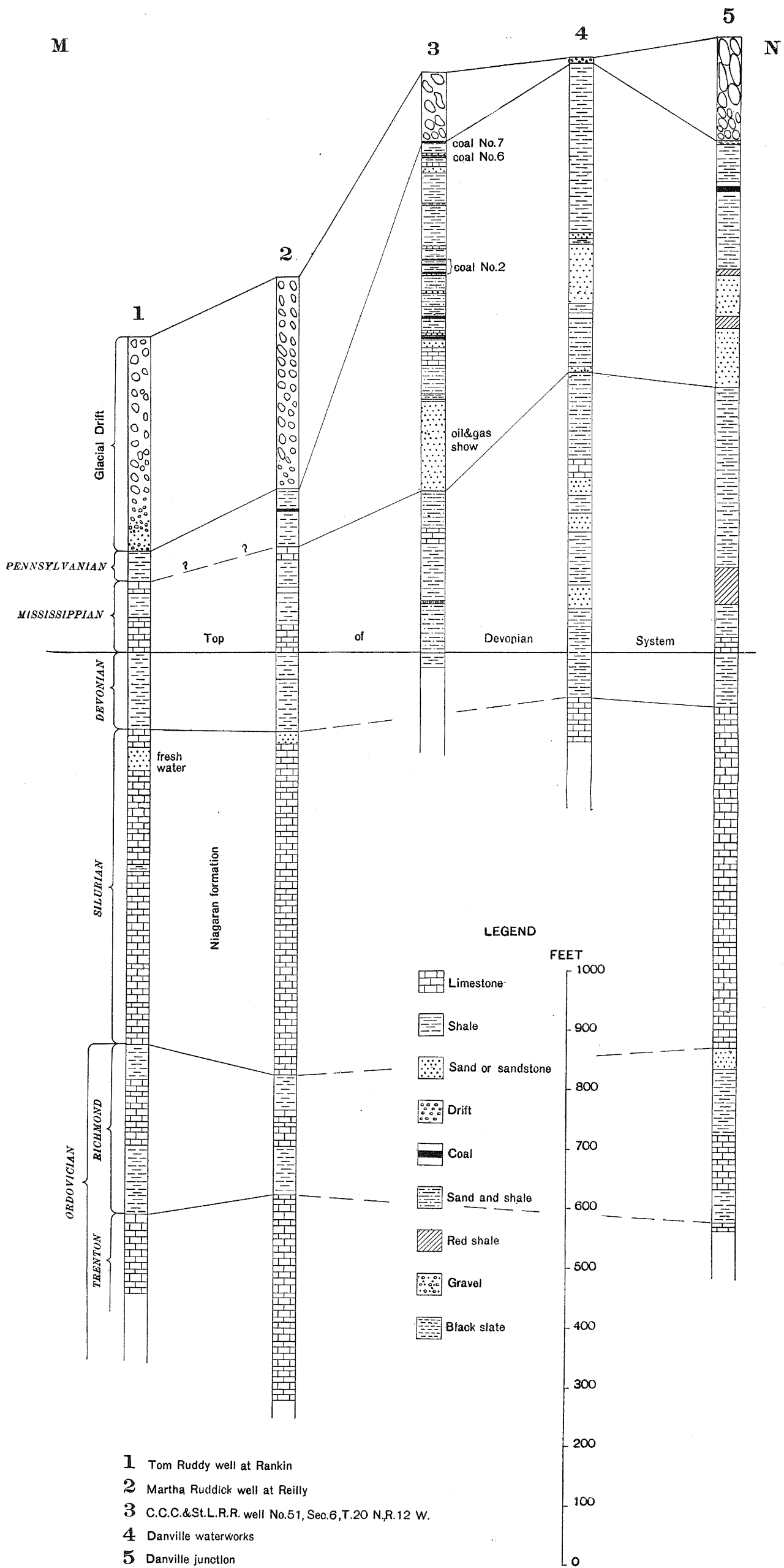
Cross-section MN showing characteristics of pre-Pennsylvanian rocks, north half of Vermilion County (For location see Plate II)
