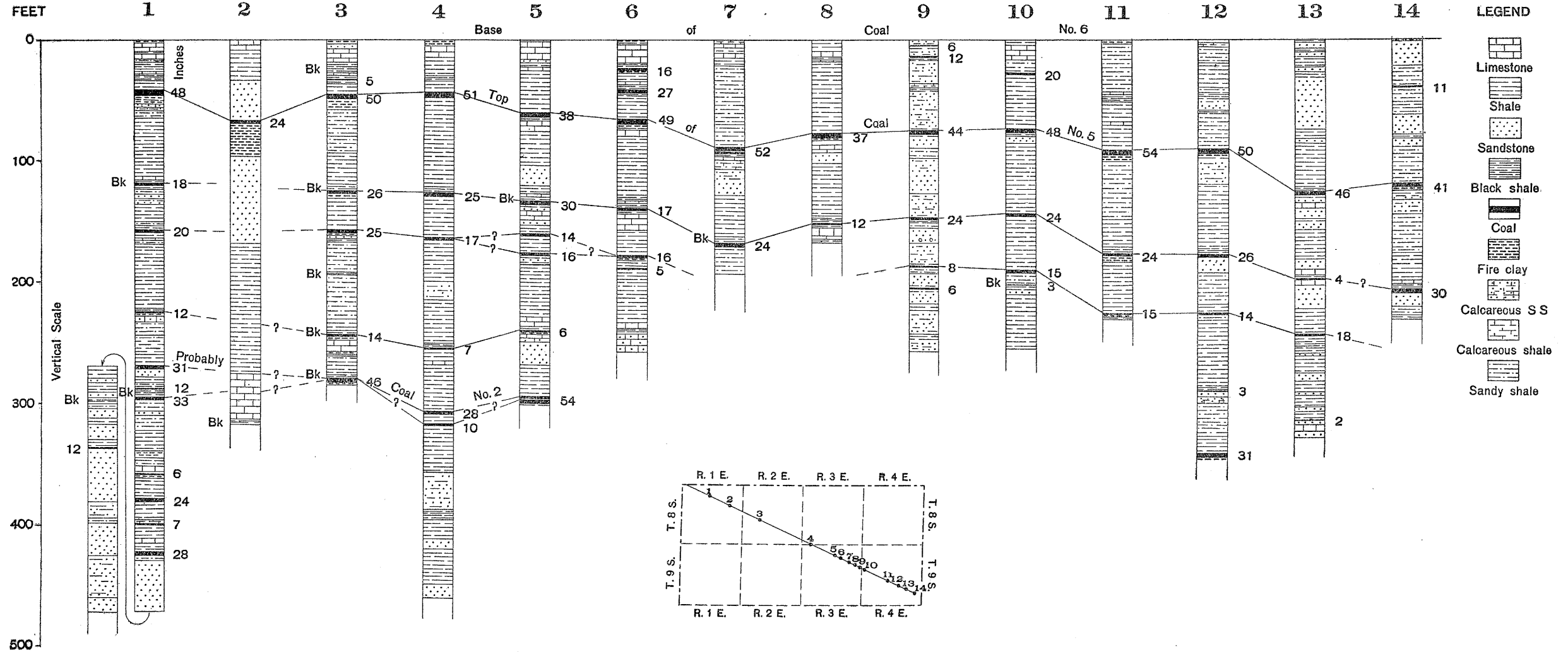
Series of graphic sections of borings showing the general character of the Carbondale and Pottsville formations in District VI.
