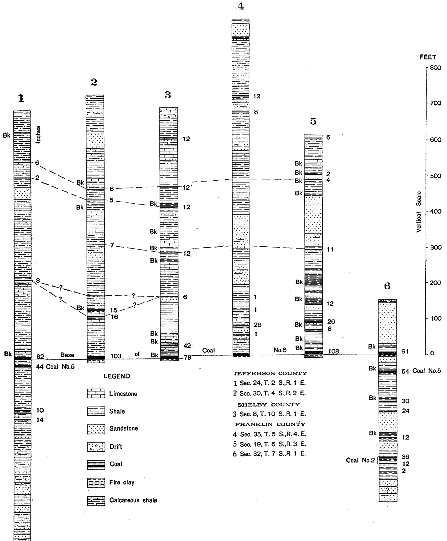
Graphic sections of borings showing the general character of the McLeansboro formation in District VI and Shelby County.
