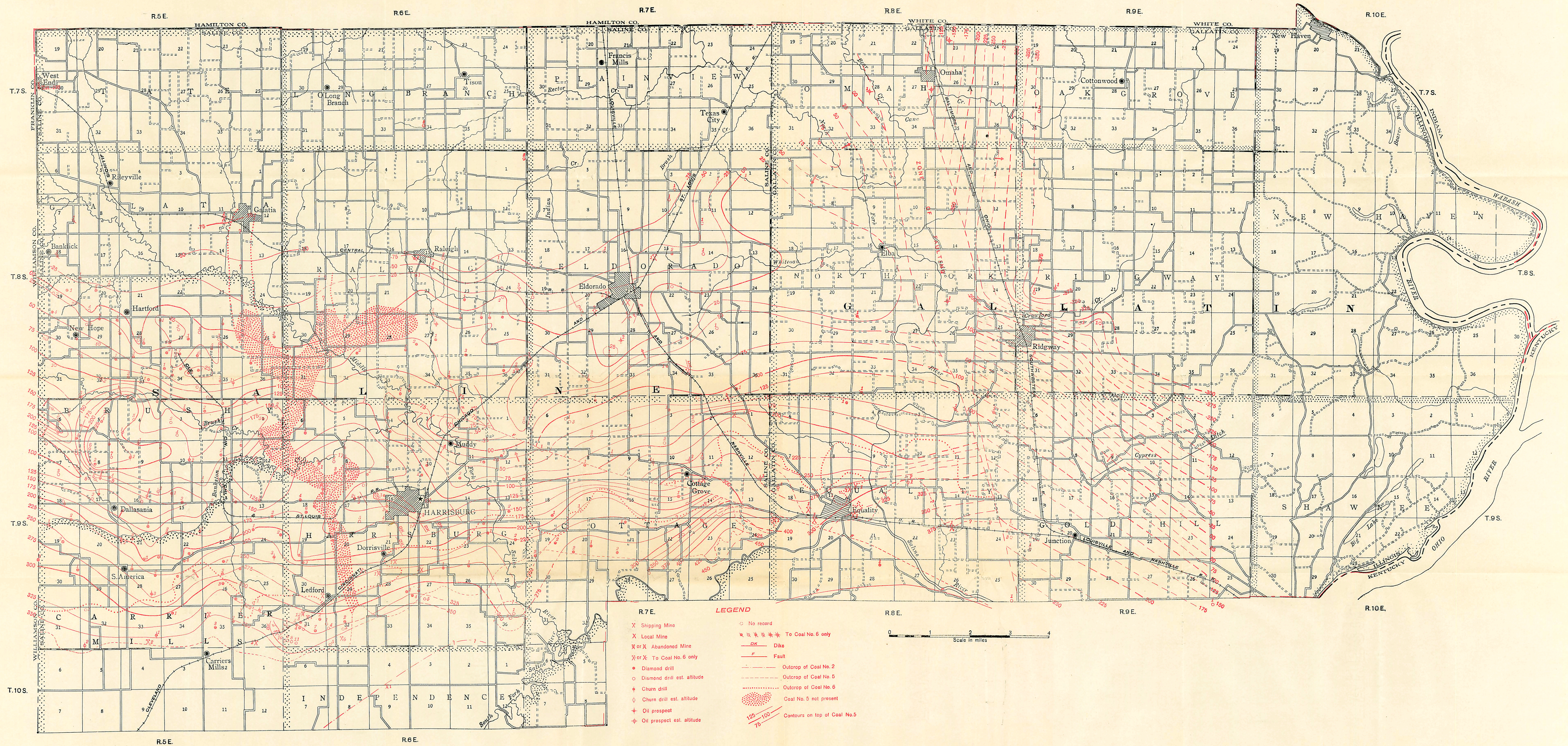
PLATE I. Map of District V showing locations of mines, drill holes, outcrops, and structure contours on No. 5 coal.
