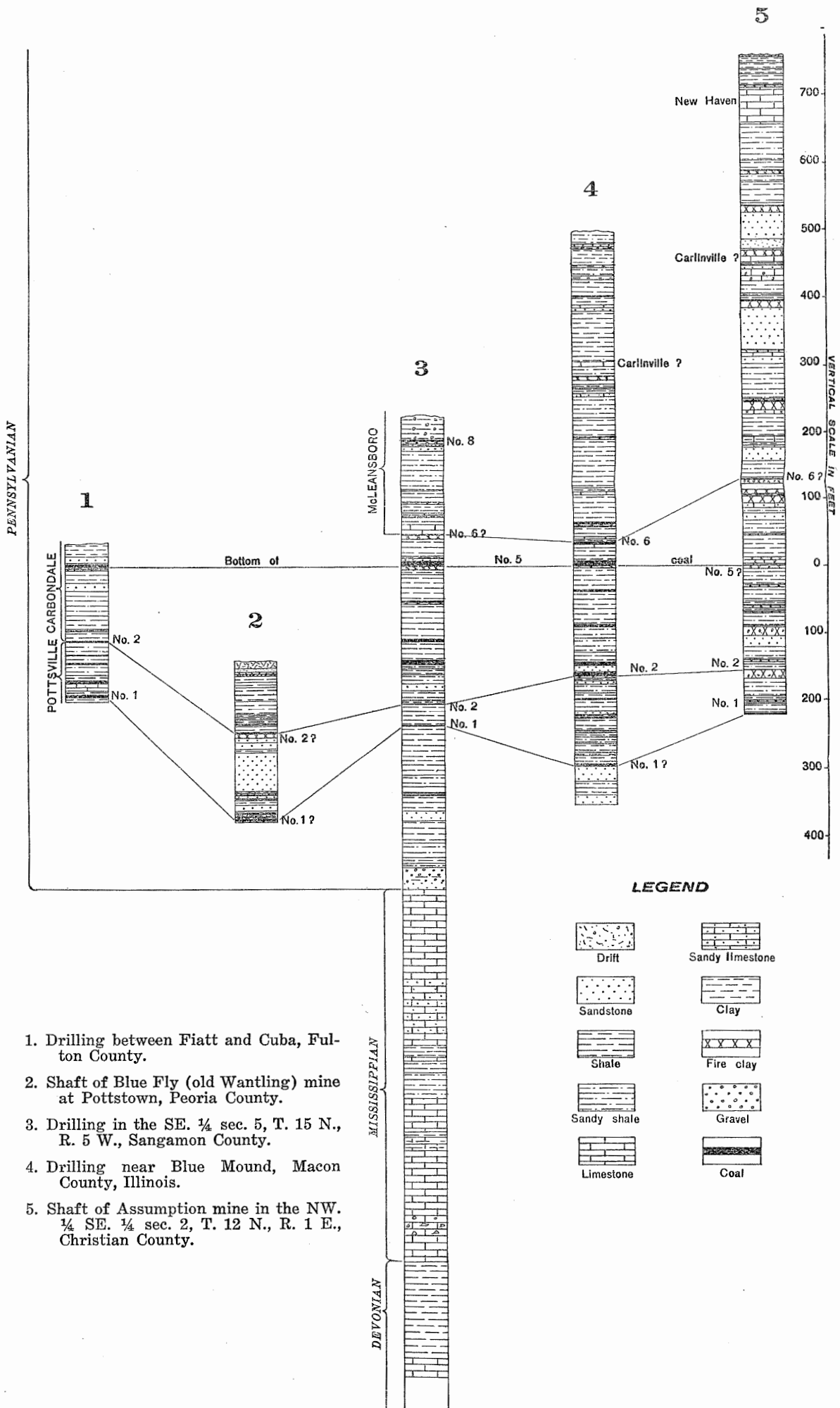
PLATE II.—Sections showing the stratigraphic relations of the coal-bearing rocks in District IV.
