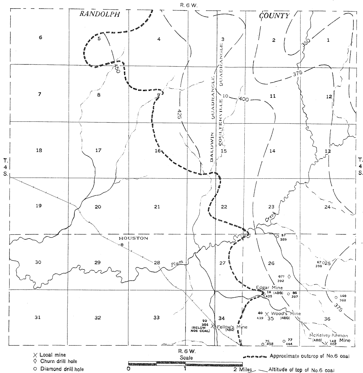
Map of Area III in northern Randolph County northwest of Sparta. Of the two numbers near a mine or drill-hole symbol, the upper represents the depth to No. 6 coal, the lower the altitude of No. 6 coal with reference to sea level
