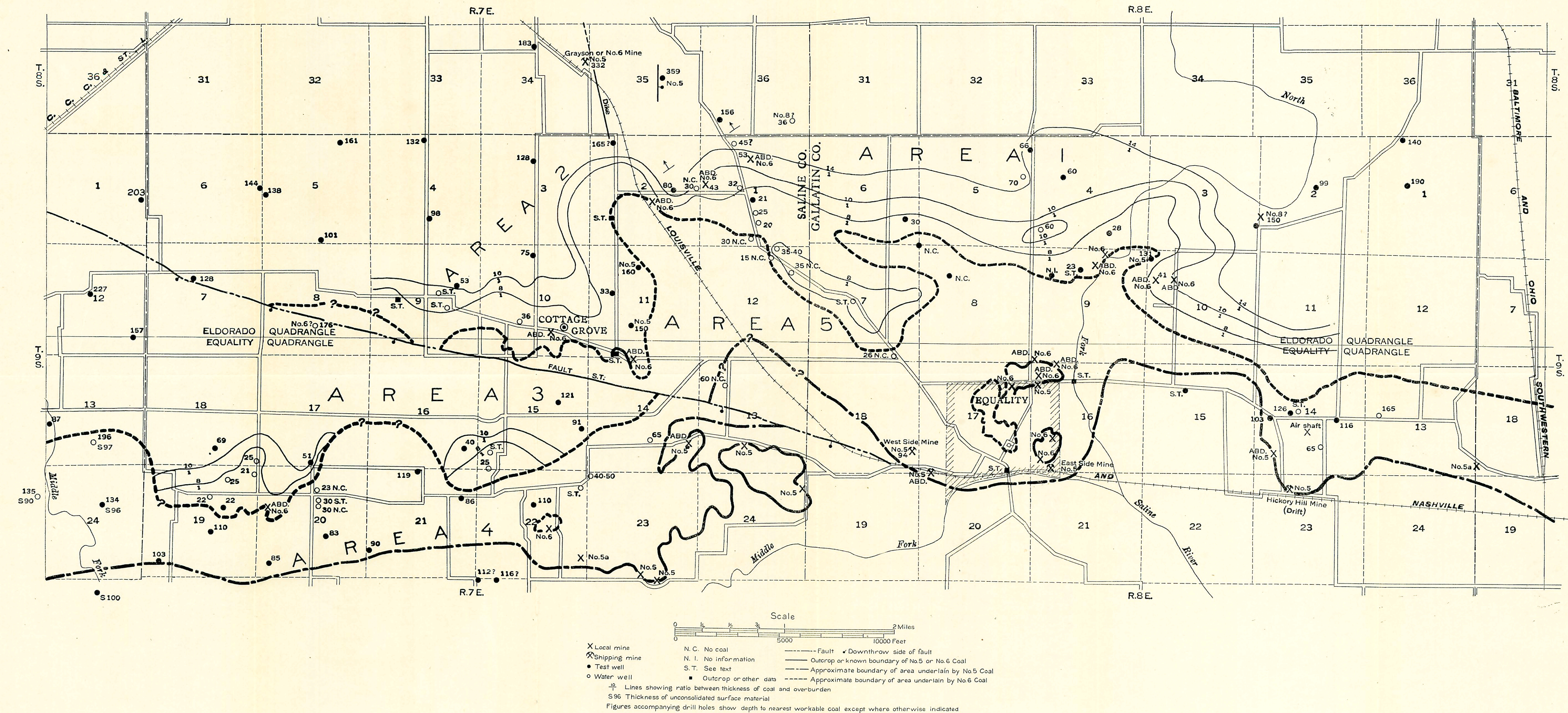
Map of portion of Saline and Gallatin counties showing the outcrop of coals No. 5 and No. 6 and data regarding the thickness of the overburden
