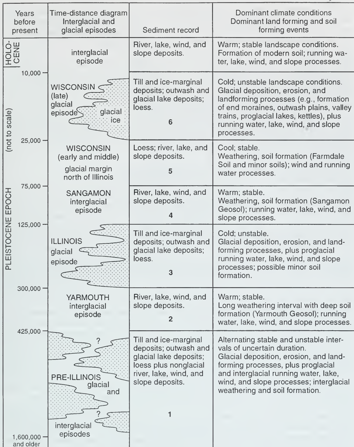
Figure 12 Timetable of glacial and interglacial events, sediment record, and dominant climate conditions of the Ice Age in Illinois (modified from Killey 1998).
