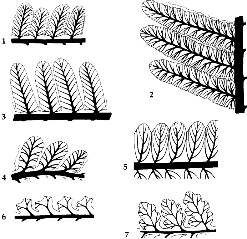
Figure 7 Venation of various forms of fern foliage: (1) Pecopteris mazoniana , X 2.5; (2) Pecopteris mazoniana , X 2.5; (3) Pecopteris hemitelioides , X 2.5; (4) Pecopteris miltonii , X 2.5; (5) Pecopteris unita , X 2.5; (6) Alloiopteris angustissima , X 4.0; (7) Sphenopteris gracilis , X 4.0
