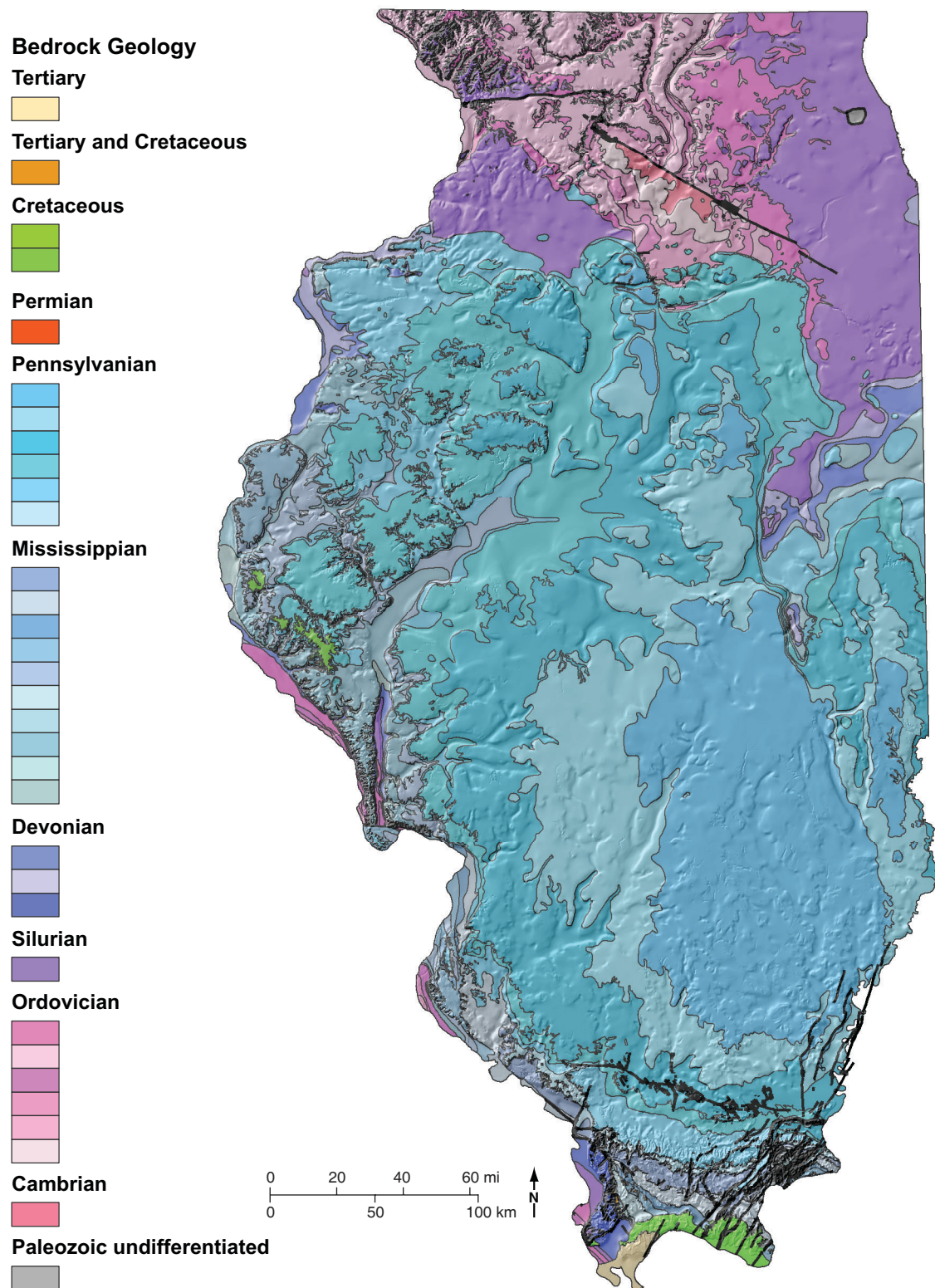
Figure 4 Generalized bedrock geology map of Illinois (Figure 2-12 from Kolata and Nimz 2010, p. 68). The black lines in the north-central and southern parts of the map are faults and fault zones.
