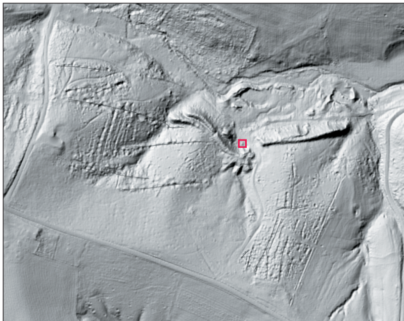
Figure 17 Lidar shaded-relief elevation model of the Vinegar Hill Mine in Vinegar Hill Township, northwestern Jo Daviess County. The distinctive linear patterns are mine diggings (also referred to as sucker holes), ranging in depth from approximately 1 to 4 feet (0.3 to 1.2 meters). The major alignments are generally oriented east–west and north–south, consistent with the orientations of bedrock fractures containing veins of minerals. The red outline marks the location of the original mine shaft. North is at the top of the image. Map by Donald E. Luman, adapted from Panno et al. (2015).
