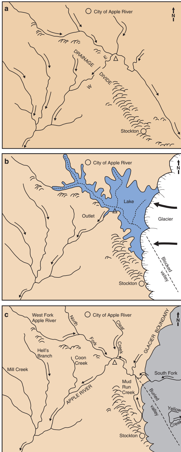
Figure 52 Formation of Apple River Canyon: (a) Preglacial drainage. (b) Formation of a lake during the Illinois glacial episode. (c) Postglacial drainage today (Figure 18 from Frankie and Nelson 2002, p. 51).
