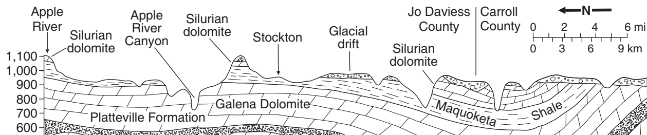
Figure 9 Cross section across Jo Daviess County showing isolated Silurian dolomite-capped mounds of the Dodgeville surface (see also Figure 56; modified from Figure 10 in Frankie and Nelson 2002, p. 15).
