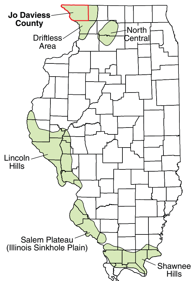
Figure 11 Map of the karst areas of Illinois showing the extent of karst terrain in Illinois, including northwestern Illinois (from Weibel and Panno 1997).
