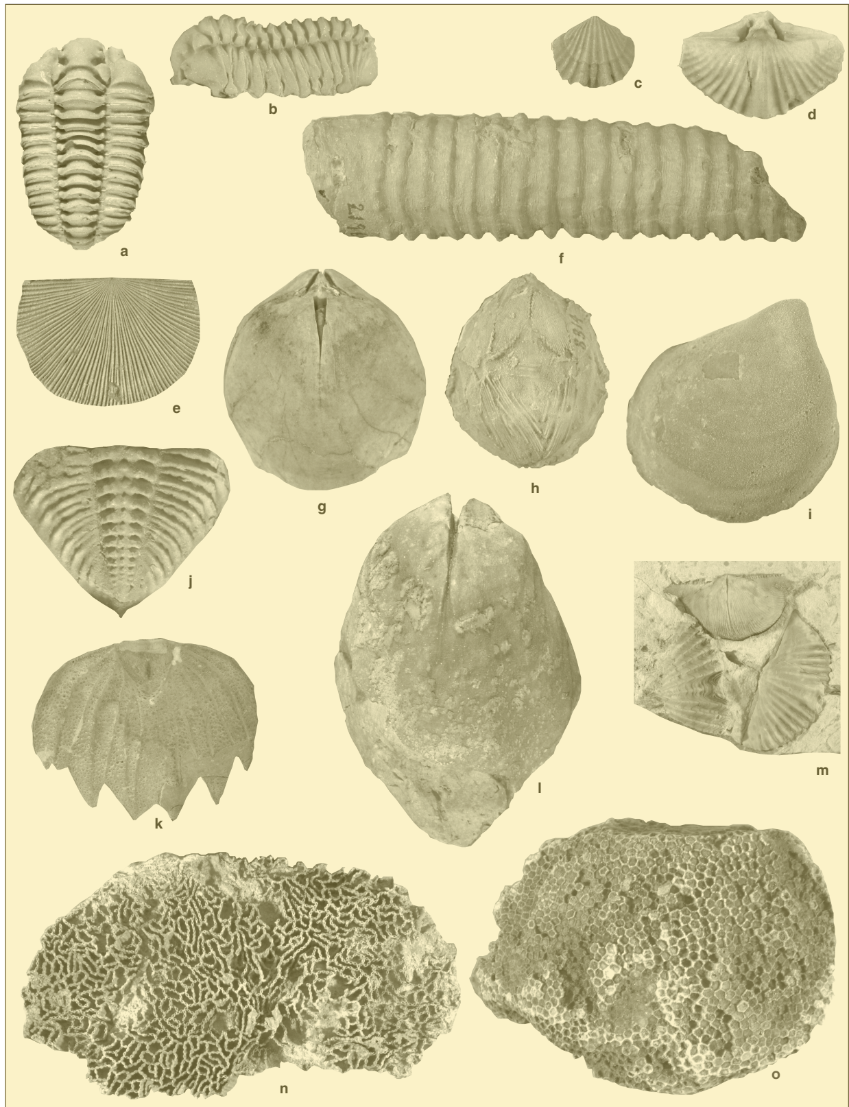
Characteristic fossils of the Silurian Period and the Early Devonian Epoch. (a, b) Trilobite Gravidicalymene celebra , 1.25×, Joliet Dolomite; (c, d) spiriferid brachiopods, 1.5×; (e) brachiopod Schuchertera sp., 1.8×; (f) cephalopod Dawsonoceras annulatum , 0.7×, Racine Dolomite; (g) brachiopod Amphigenia curta , 1.4×; (h) cystoid Caryocrinites sp., 1.2×, Racine Dolomite; (i) bivalve Amphicoelia neglecta , 1.0×, Racine Dolomite; (j) trilobite pygidium Glyptambon gassi , 2.0×, Racine Dolomite; (k) trilobite pygidium Arctinurus occidentalis , 0.9×, Racine Dolomite; (l) brachiopod Pentamerus sp., 0.9×, Marcus Dolomite; (m) brachiopod Eodevonaria arcuata (upper) and spiriferid brachiopods (lower), 1.1×; (n) colonial coral Halysites sp., 0.6×; (o) colonial coral Favosites sp., 0.6×, Louisville Limestone. Fossils c, d, e, g, and m are from the Lower Devonian Clear Creek Formation (from Kolata and Nimz 2010, p. 162).
