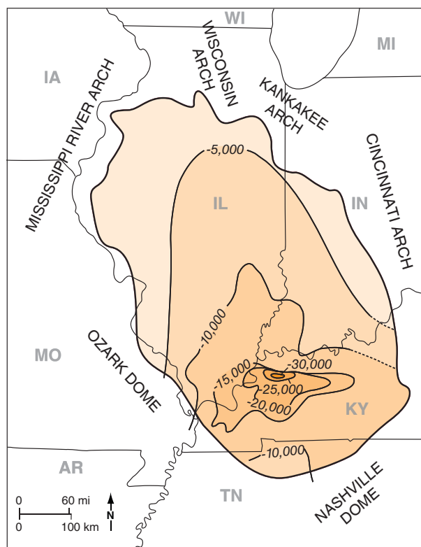
Figure 3 The Illinois Basin and all the surrounding structures (arches and domes) that bound the basin margins (Figure 2-2 from Kolata and Nimz 2010, p. 60).
