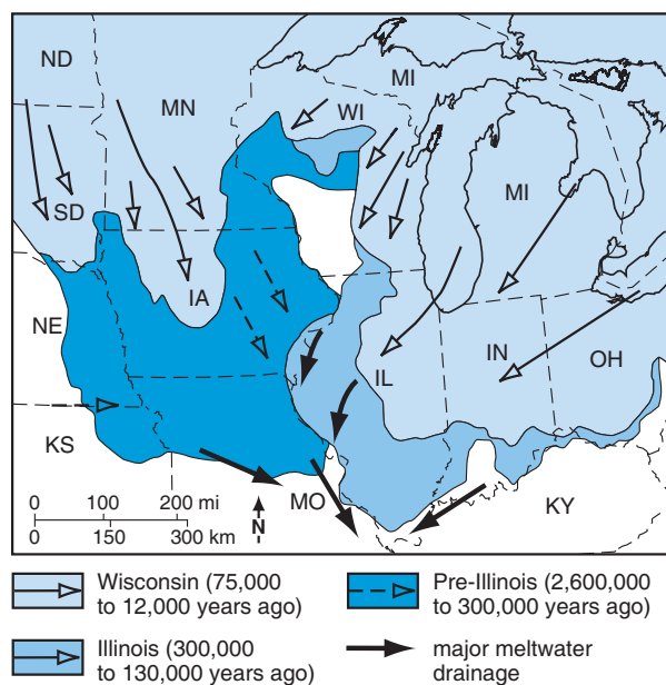
Figure 6 Glaciation of North America in the vicinity of Jo Daviess County showing the extent of pre-Illinois glaciation, the extent of the Illinois glacial episode, and the extent of the Wisconsin glacial episode (Figure 3 modified from Killey, 2007, p. 3). Note the Driftless Area in white surrounded by glaciers in the upper center of the figure.
