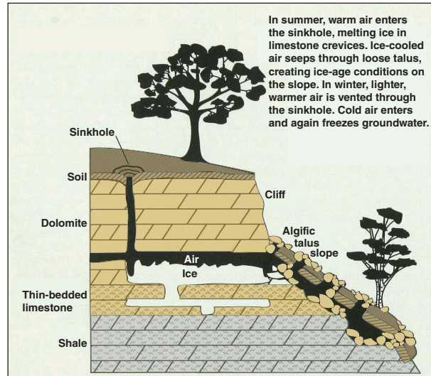
Figure 47 Conceptual model of an algific talus slope (modified from Anderson and Danielson 1999). Used with permission.
