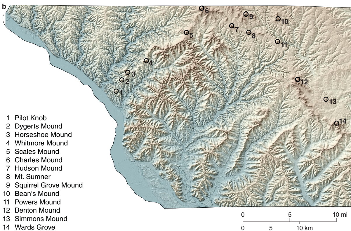
Figure 56 (a) Numerous Silurian dolomite-capped knobs may be seen in the distance, as viewed from Benton Mound. Photograph by Samuel V. Panno; used with permission. (b) Lidar surface topography map of Jo Daviess County. The darker reddish-brown portions demarcate the highest elevations, which are capped by resistant Silurian-age dolomite. Fourteen named mounds mark the summits along the ridge tops. Map by Donald E. Luman.
