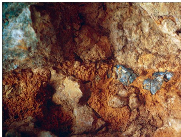
Figure 26 Lead ore (galena) is found within crevices in the Galena-Platteville Formation. The cubic crystal structure of the mineral can be seen here. Photograph by Samuel V. Panno; used with permission.
