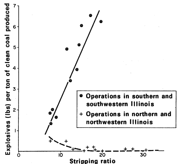
Fig. 11 - Correlation between quantity of explosives used and stripping ratio, 1970 (Illinois Dept. of Mines and Minerals, 1970).
