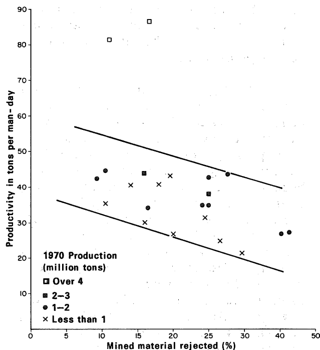
Fig. 15 - Strip mine productivity in relation to the percentage of material rejected in 1970.
