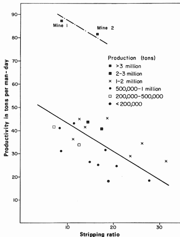
Fig. 10 - Stripping ratio and mine productivity of Illinois mines in 1970.
