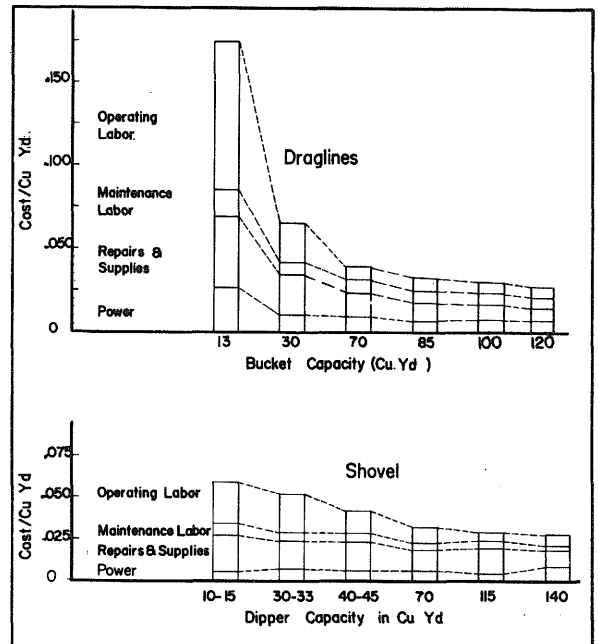
Fig. 12 - Relative gains made with larger equipment (after Weimer and Weimer, 1973).
