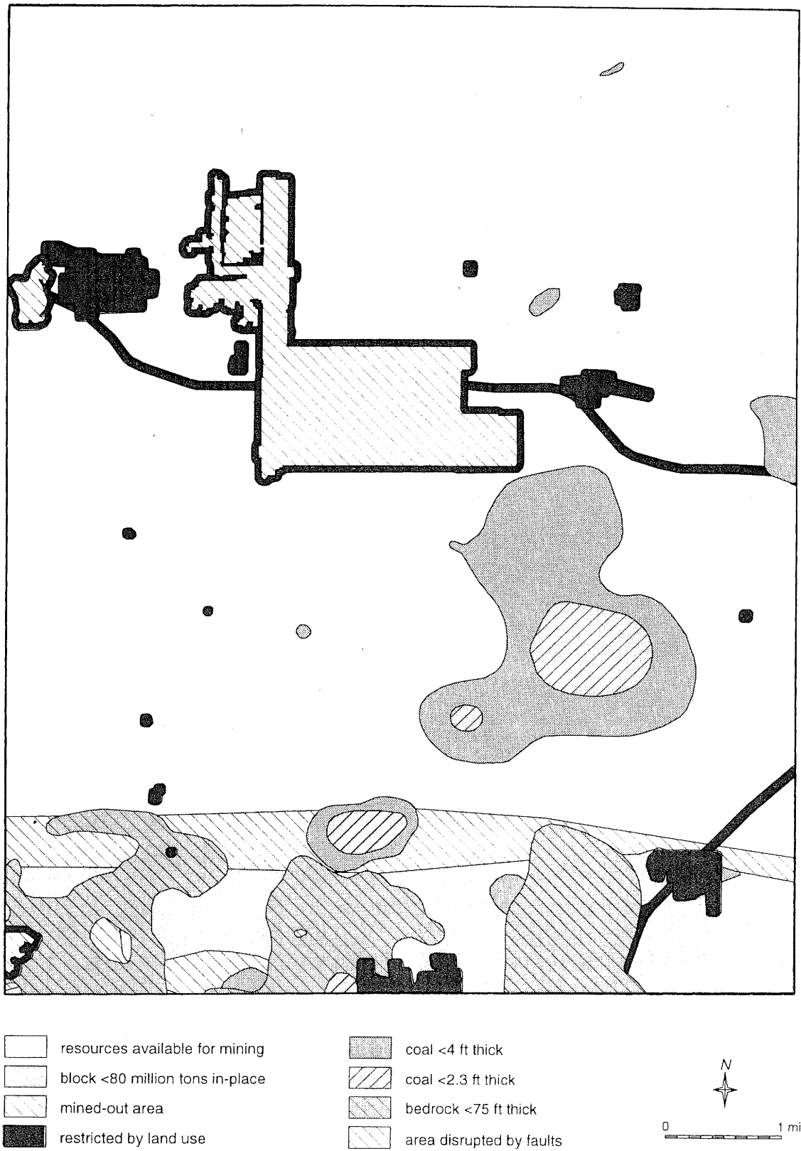
Figure 16 Availability of Herrin Coal resources for underground mining in the Galatia Quadrangle.
