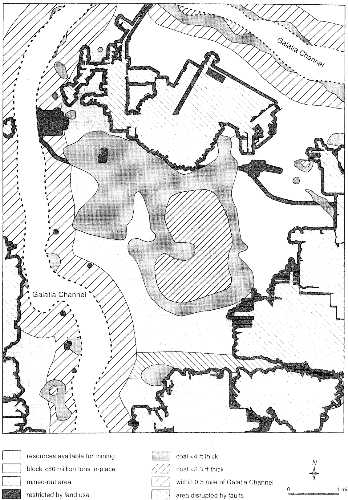
Figure 17 Availability of Springfield Coal resources for underground mining in the Galatia Quadrangle.
