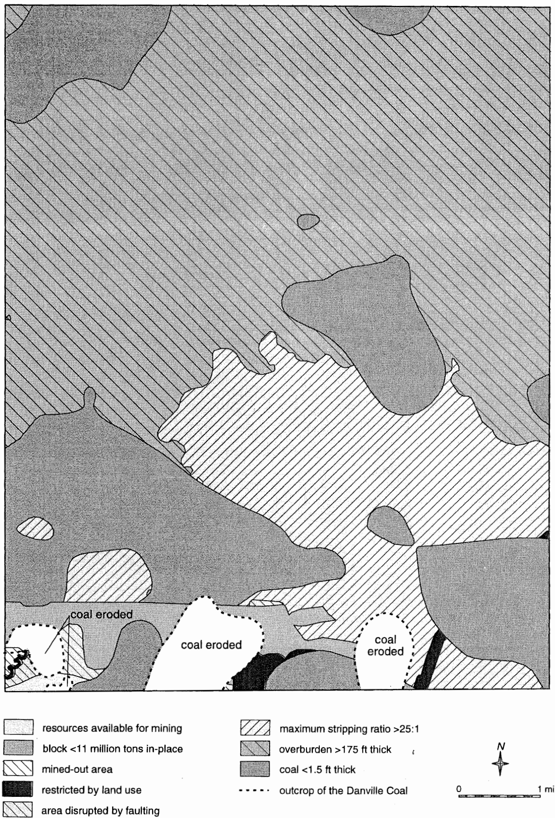
Figure 13 Availability of Danville Coal resources for surface mining in the Galatia Quadrangle.
