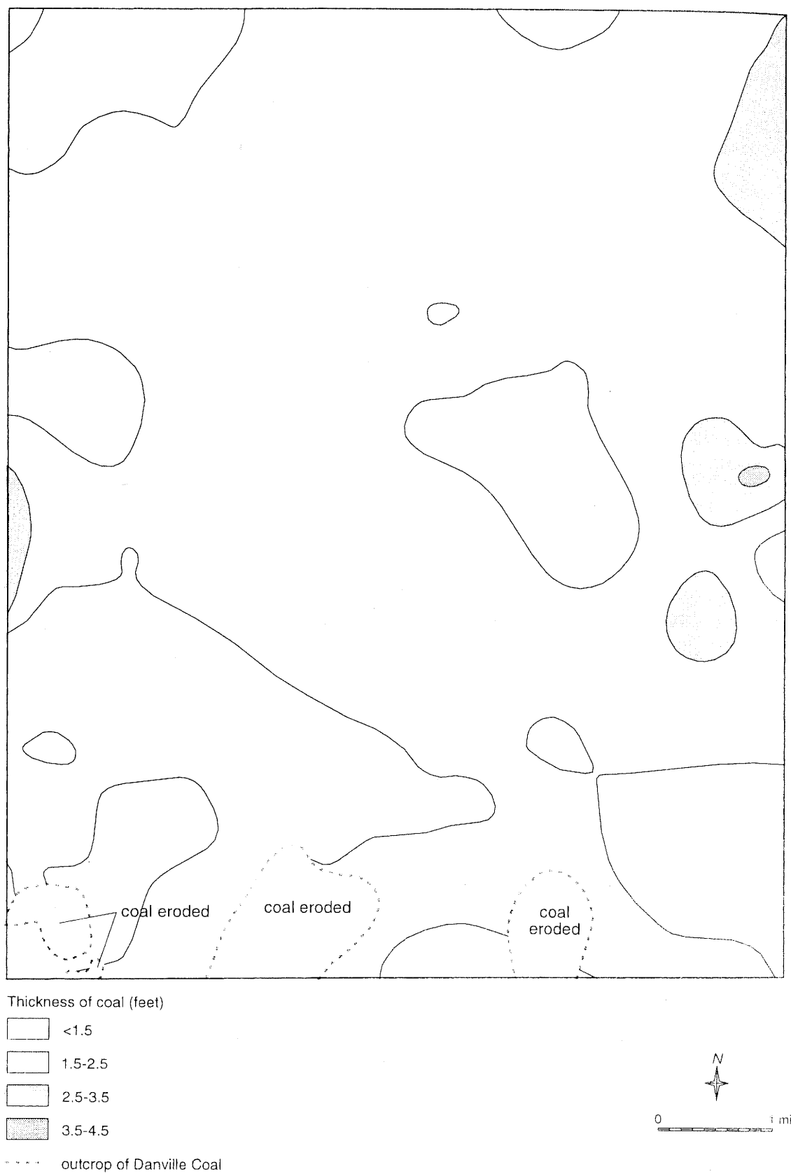
Figure 12 Thickness of the Danville Coal in the Galatia Quadrangle.
