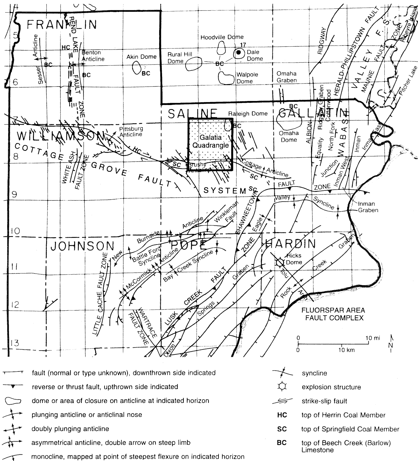
Figure 2 Structural features in the coal-bearing portion of region 7 (from Nelson 1995).
