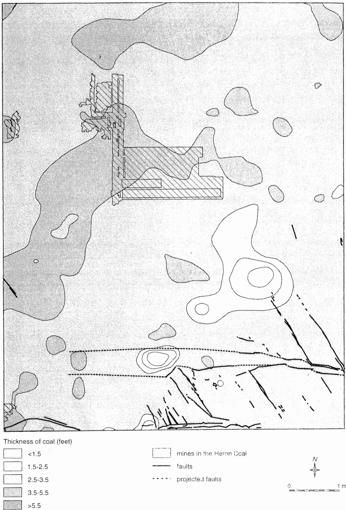
Figure 14 Thickness of the Herrin Coal in the Galatia Quadrangle.
