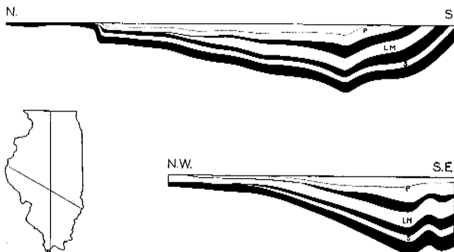
FIG. 2.—CROSS-SECTIONS OF ILLINOIS BASIN
