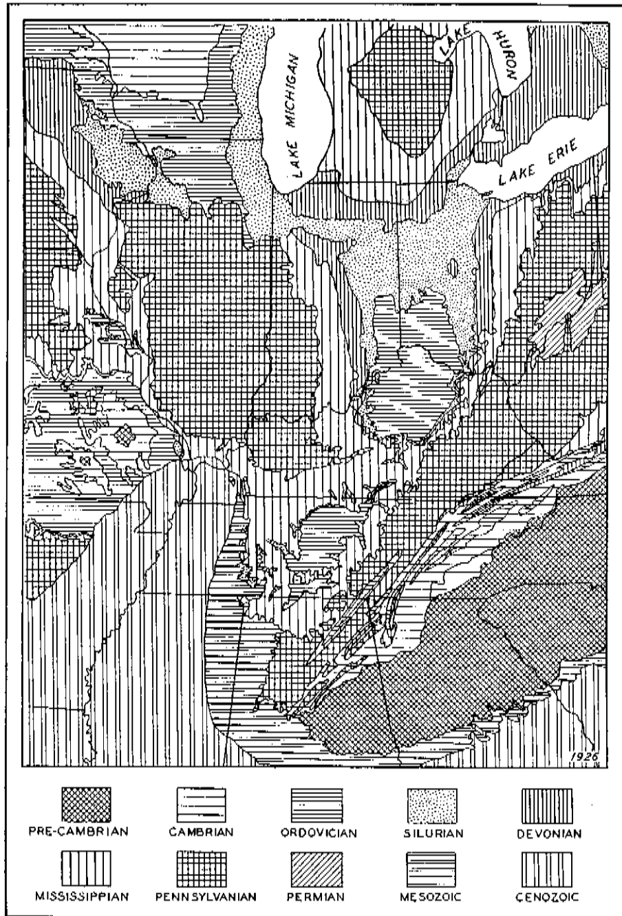
FIG. 1.—GEOLOGICAL MAP OF EAST CENTRAL UNITED STATES
