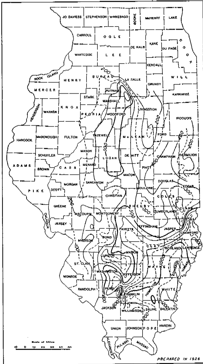
FIG. 5.—ISOPACH MAP SHOWING THE THICKNESS OF PENNSYLVANIAN BEDS BELOW COAL NO. 6 For correction see explanation below Plate 1
