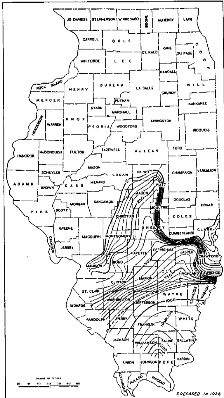
FIG. 6.—ISOPACH MAP SHOWING THE THICKNESS OF THE UPPER MISSISSIPPIAN STRATA For correction see explanation below Plate I
