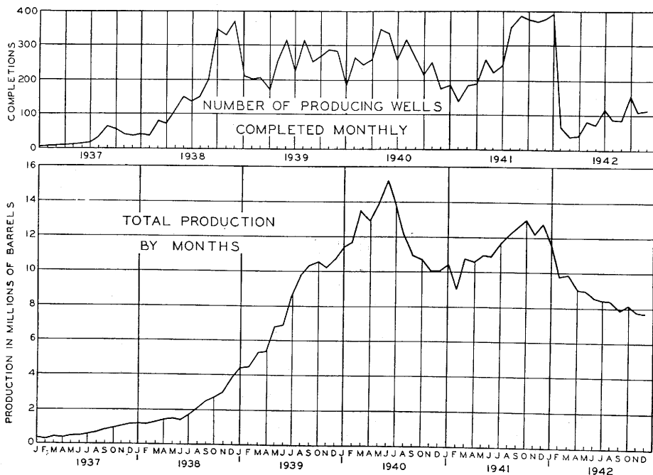
FIG. 1.—MONTHLY OIL PRODUCTION AND WELL COMPLETIONS IN ILLINOIS 1937-1942.
