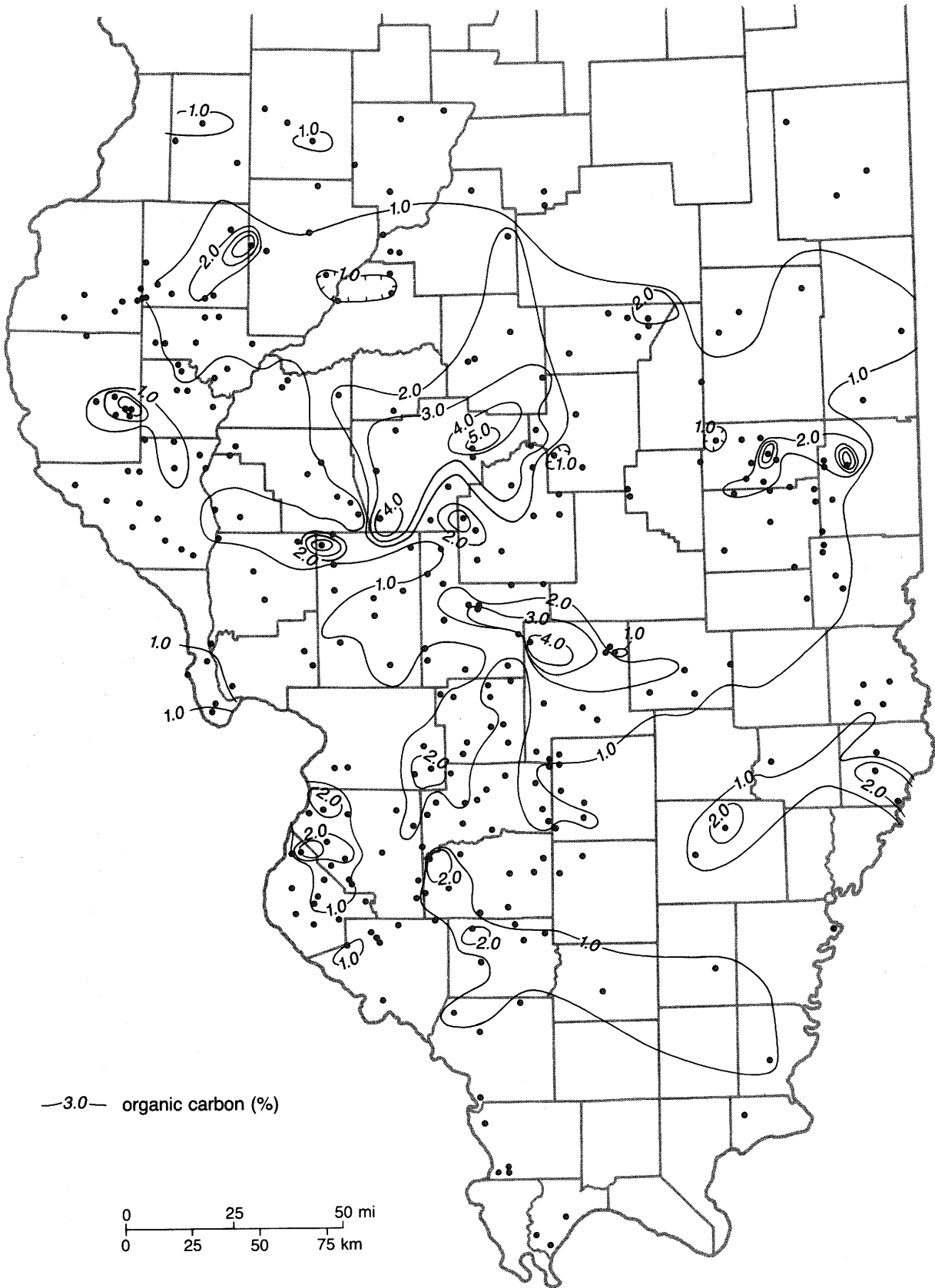
Figure 1 Variation in the geographic distribution of organic carbon content of shales from the Maquoketa Group.
