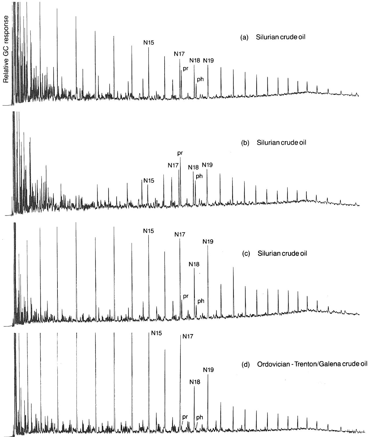
Figure 9 Typical GC fingerprints of whole crude oils from reservoirs in (a) Silurian (Adams County, IL); (b) Silurian (De Witt County, IL); (c) Silurian (Sangamon County, IL); and (d) Ordovician (Macon County, IL). Peak numbers correspond to n -alkane carbon numbers (ex. N15 = n -C 15 ), pr = pristane; ph = phytane.
