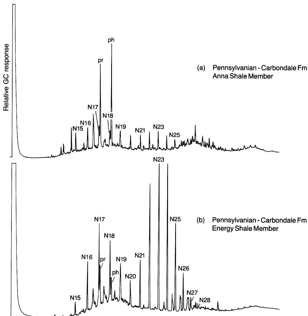
Figure 13 Typical GC fingerprints of the extractable aliphatic hydrocarbons from the (a) Anna Shale Member and (b) Energy Shale Member of the Pennsylvanian Carbondale Formation. Peak numbers correspond to n -alkane carbon numbers (ex. N15 = n -C 15 ); pr = pristane; ph = phytane.
