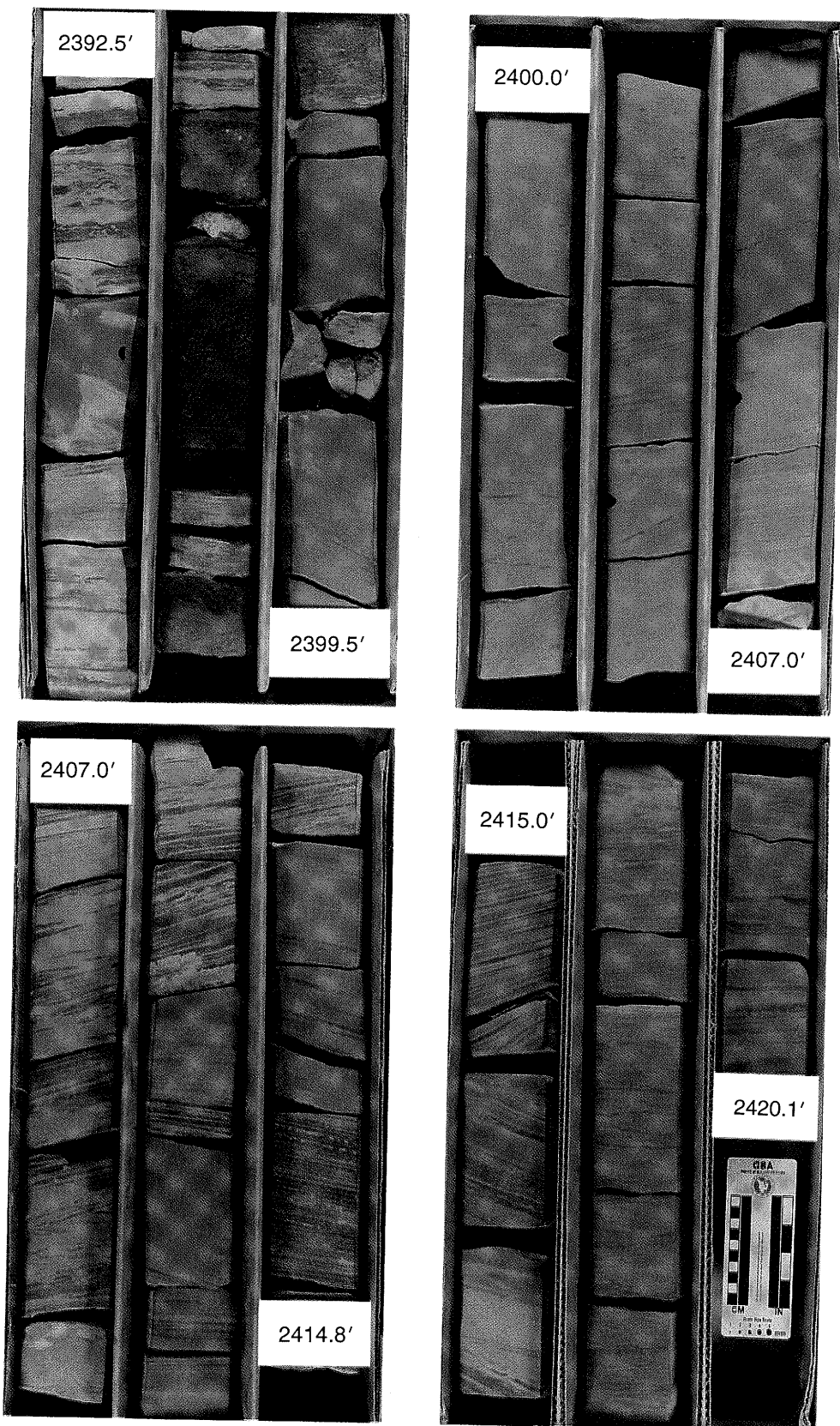
Plate 1 Core through Aux Vases siliciclastic interval (2,392.5 to 2,420.1 feet, Budmark Oil Company, Burr Oak No. 3 well, NE SE NE, Section 33, T8S, R4E). See appendix E for description.
