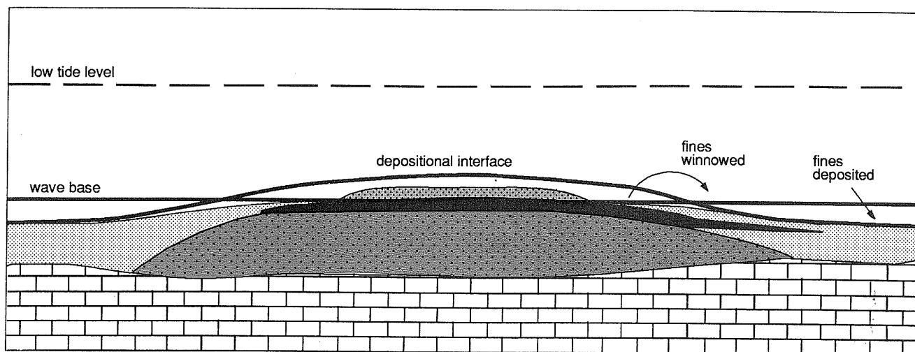
Figure 12 Subtidal winnowing of sediments by wave action concentrates coarser material on top of lower bars and produces upper sand reservoirs as crestal deposits.
