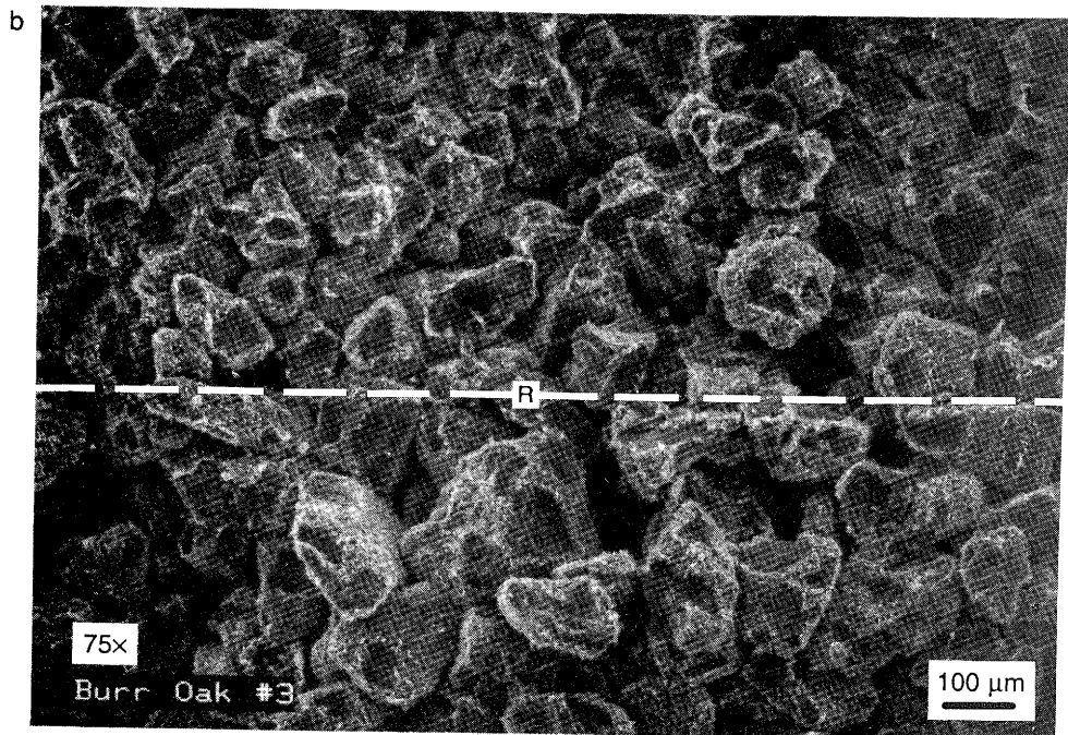
Plate 11 Comparison of low magnification SEM images of a) at 2393.5 ft depth, upper sandstone, and b) at 2405.2 ft depth, lower sandstone. Note difference in grain sizes and upper sand porosity occlusion by cement. A rhythmite sequence (R) is visible in the lower sandstone. Surface separates fine grained sand from coarse grained sand in lower portion of image.
