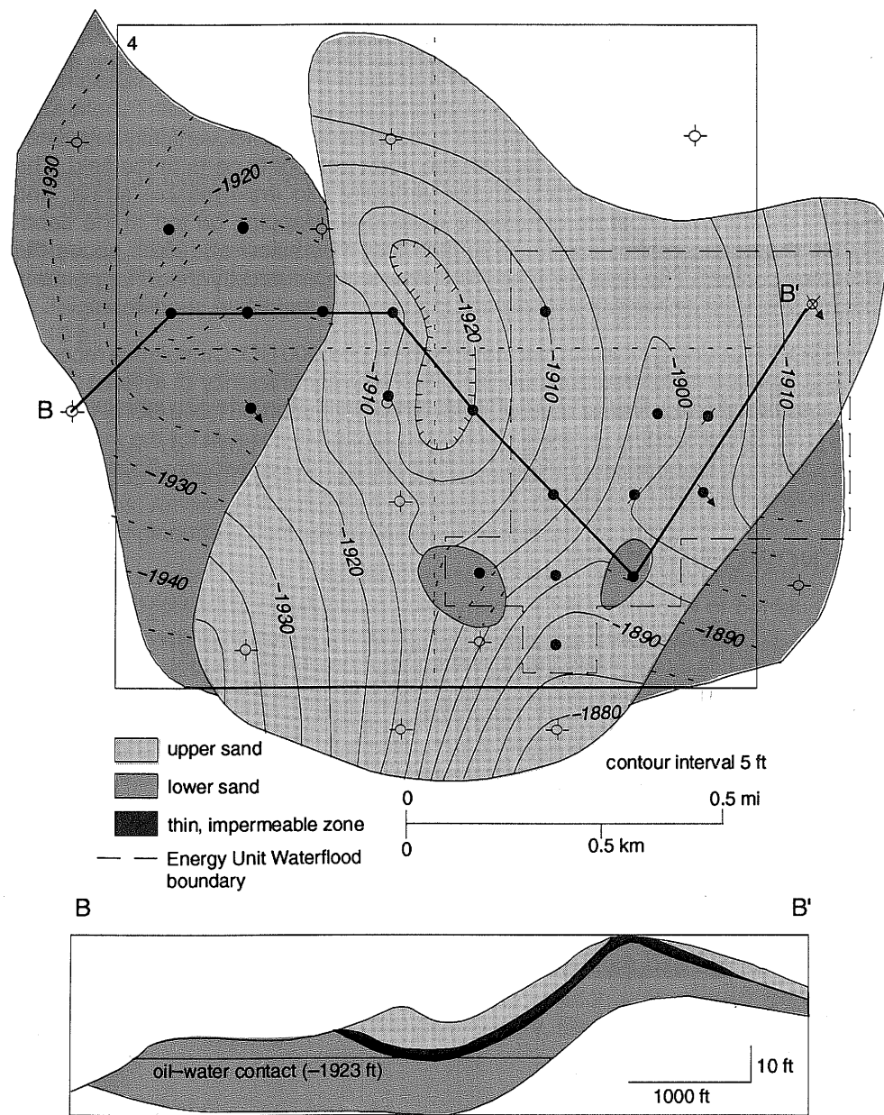
Figure 14 Structure contour map on top of Aux Vases Sandstone, southern bar complex, Section 4, T9S, R2E. Cross section B-B' shows Aux Vases sandstone interval. Solid contours show upper sand elevation; dashed contours show lower sand elevation.
