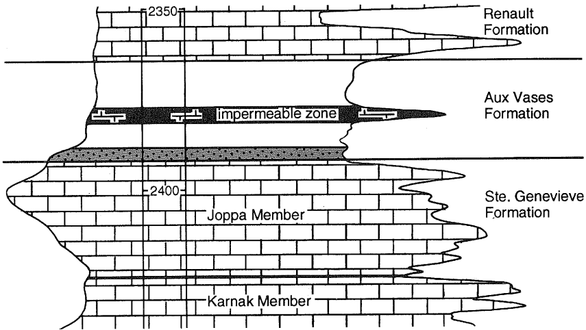
Figure 5 Log responses and lithofacies from Energy Field.
