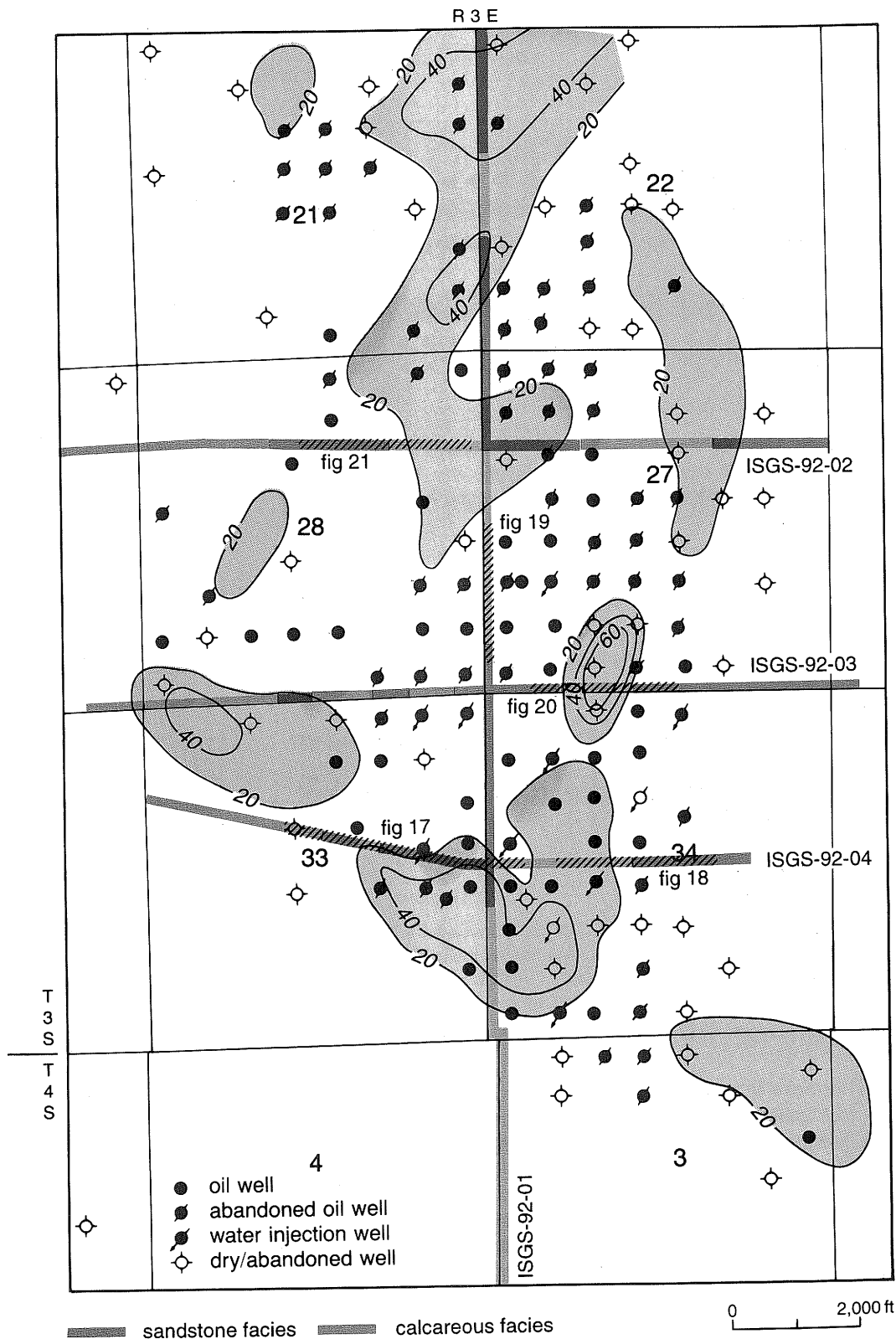
Figure 13 Map of the percentage of calcareous lithofacies in the Aux Vases Formation. The areas in blue contain greater than 20% calcareous lithofacies (Leetaru 1991). The calcareous lithofacies is characterized by log intervals with measured resistivities greater than 40 ohm-m. The two colors on the seismic lines indicate sandstone or calcareous Aux Vases lithofacies as interpreted by seismic character analysis.
