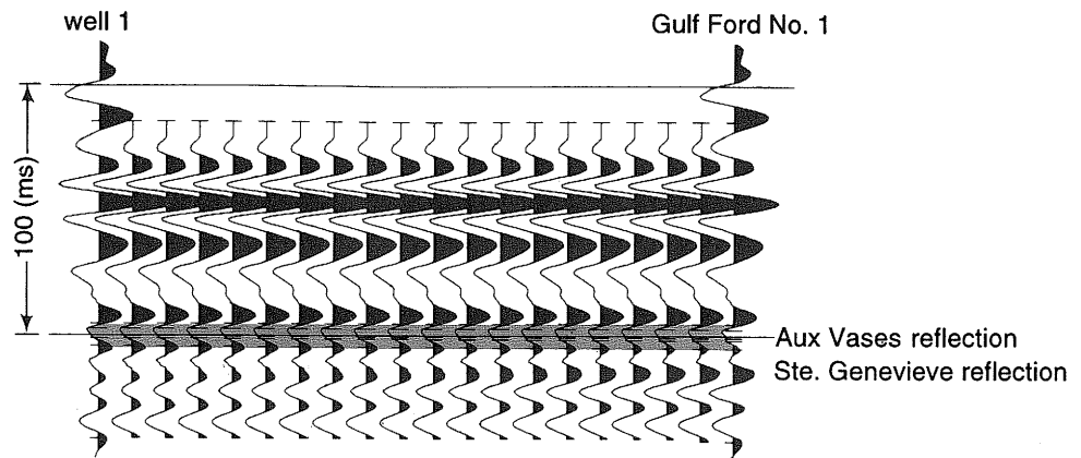
Figure 12b Synthetic seismic model convolved with wavelet A. The seismic amplitude variation in the reflection at the top of the Ste. Genevieve is a result of destructive and constructive interference by the changes in the Aux Vases facies.
