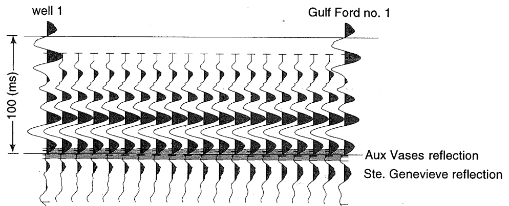
Figure 12c Synthetic seismic model convolved with wavelet B. The seismic amplitude variation in the Ste. Genevieve reflector is similar to that illustrated by the higher frequency model (fig. 12b).
