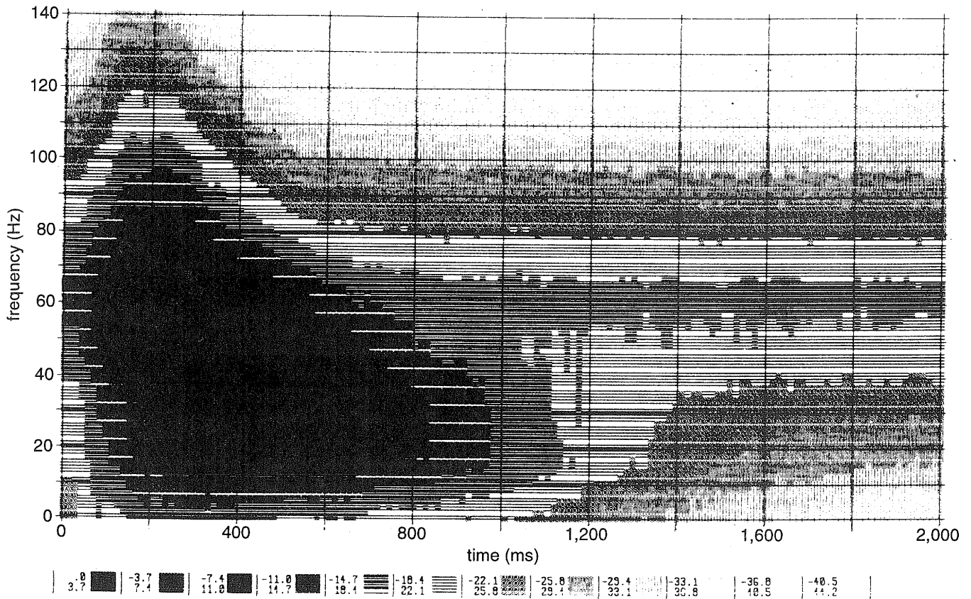
Figure 5b Frequency-time plot of the raw field record. There is a 30% attenuation of the high frequencies from 200 to 500 ms.
