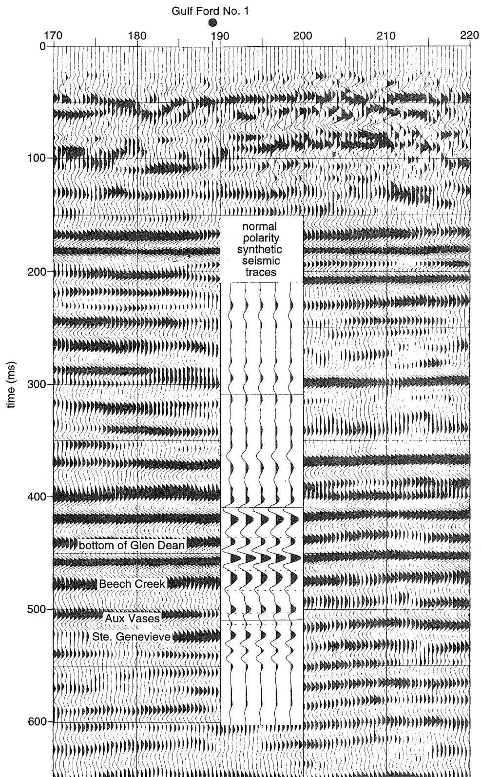
Figure 9b Seismic line ISGS-92-04 compared to the normal polarity synthetic seismic traces of Gulf Ford No. 1.
