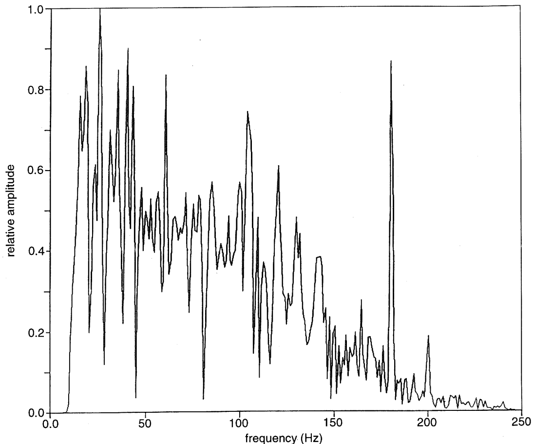
Figure 6 Amplitude spectrum versus frequency for a single trace deconvolution. The spectrum shows a rapid attenuation of the signal above 140 Hz.
